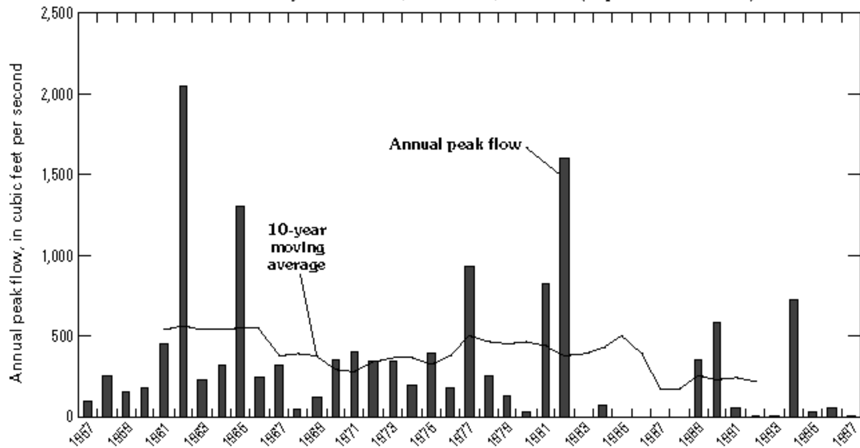
Figure 5VV. Annual peak flows and 10-year moving averages using available periods of record—Continued. Location of station shown in figure 3.
