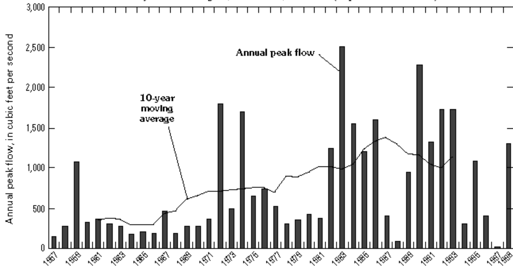
Figure 5W. Annual peak flows and 10-year moving averages using available periods of record—Continued. Location of station shown in figure 3.
