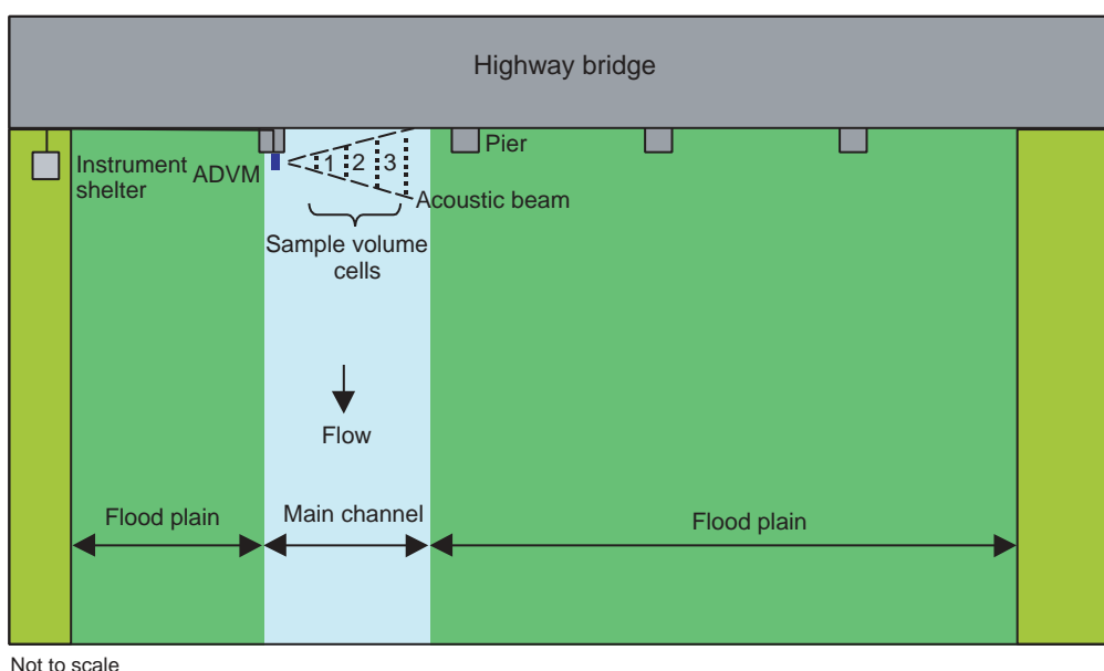
Figure 6. Photographs and site sketch of Fall Creek at Millersville, Ind., acoustic Doppler velocity meter (ADVM) evaluation station.
