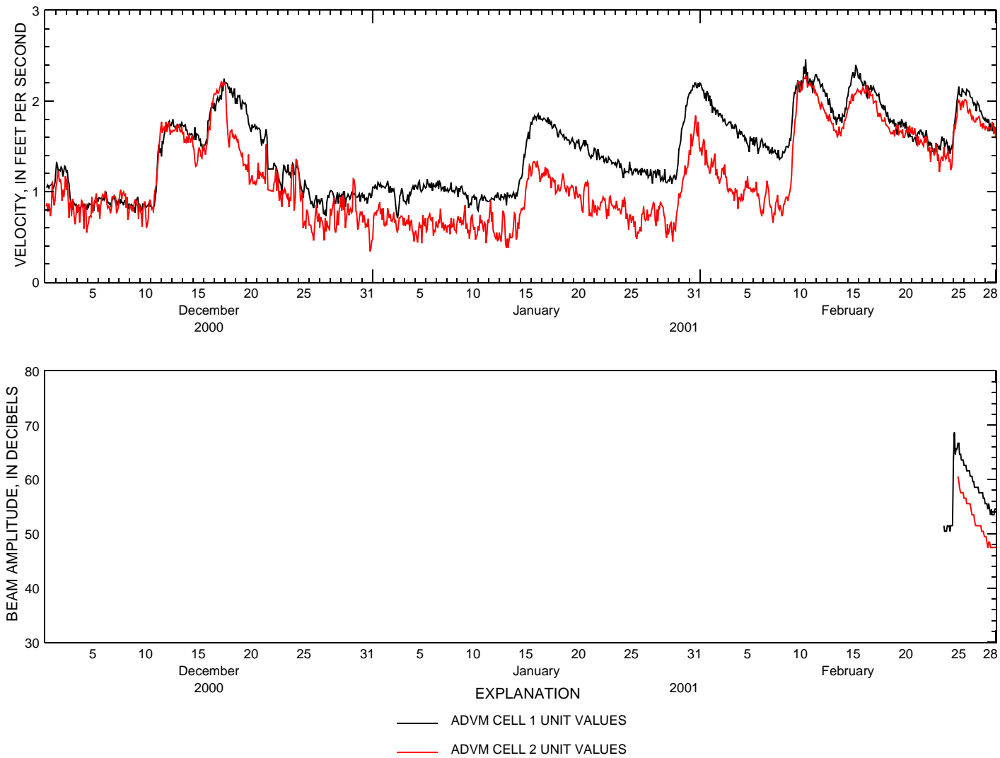
Figure 16. Acoustic Doppler velocity meter (ADVM) cell 1 and 2 velocity unit values and beam-amplitude unit values from the ADVM evaluation site Fall Creek at Millersville, Ind., December 1, 2000–February 28, 2001 (Note: beam-amplitude scale is approximate).
