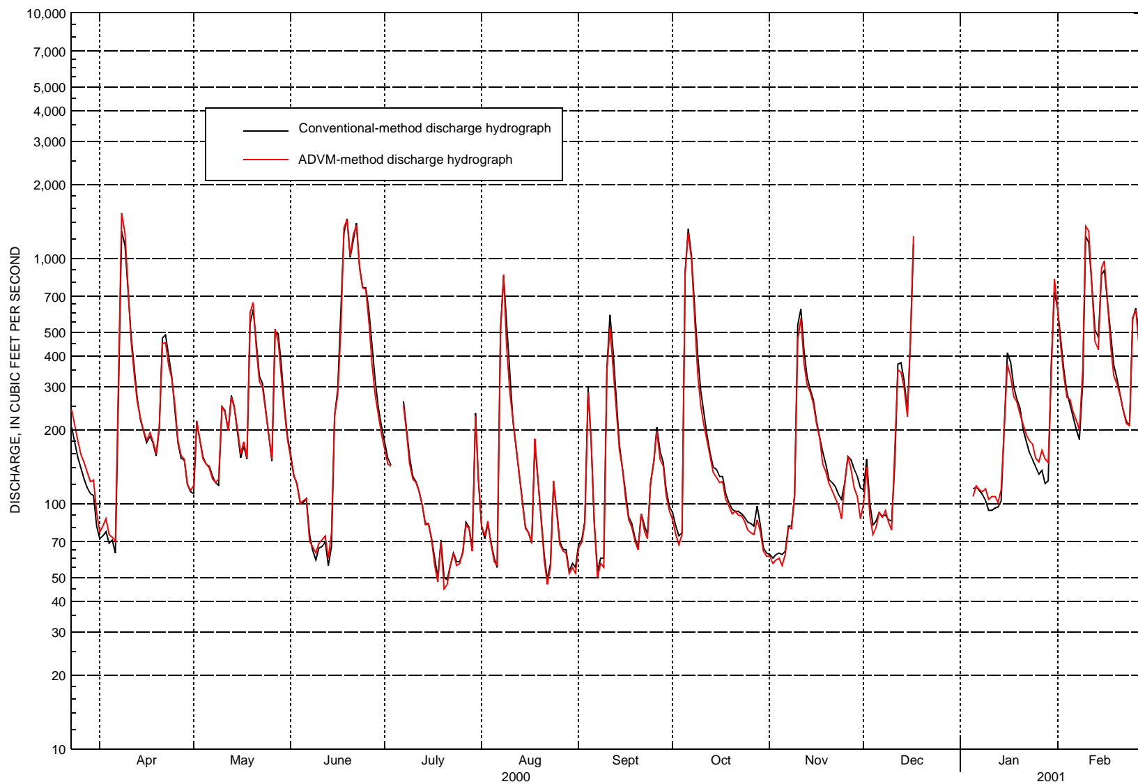
Figure 19. Comparison of mean-daily discharge hydrographs produced by conventional method and acoustic Doppler velocity meter (ADVM) methods, using ADVM cell 2, from the Fall Creek at Millersville, Ind., ADVM evaluation station, March 23, 2000–February 28, 2001 (Note: breaks in graph represent periods of missing data).
