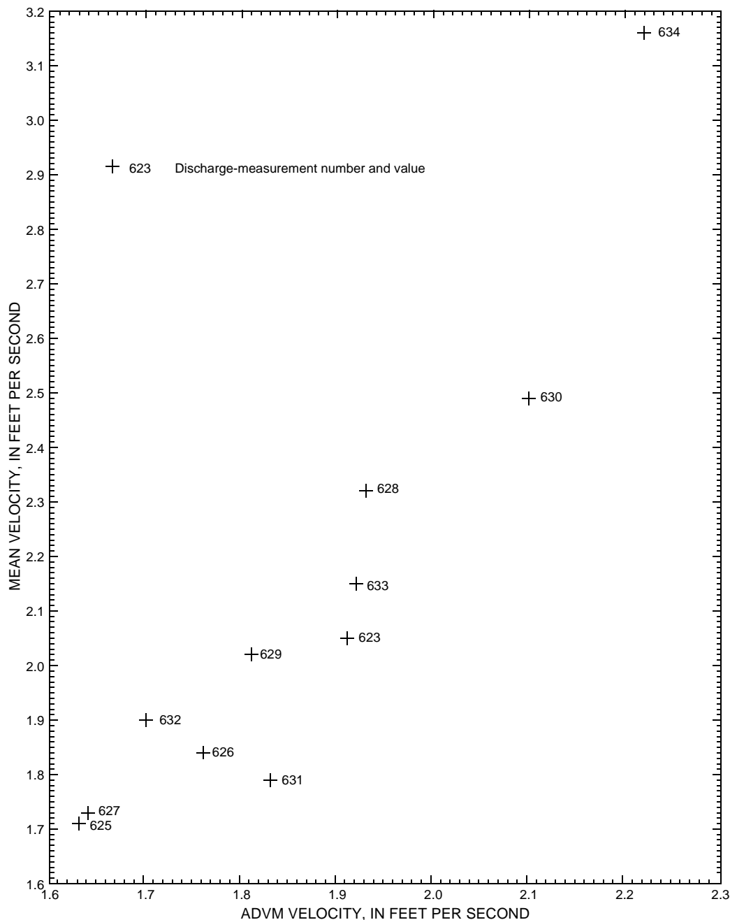
Figure 12. Mean velocity and acoustic Doppler velocity meter (ADV) velocities from discharge measurements made at the Kankakee River at Davis, Ind., ADV evaluation station.
