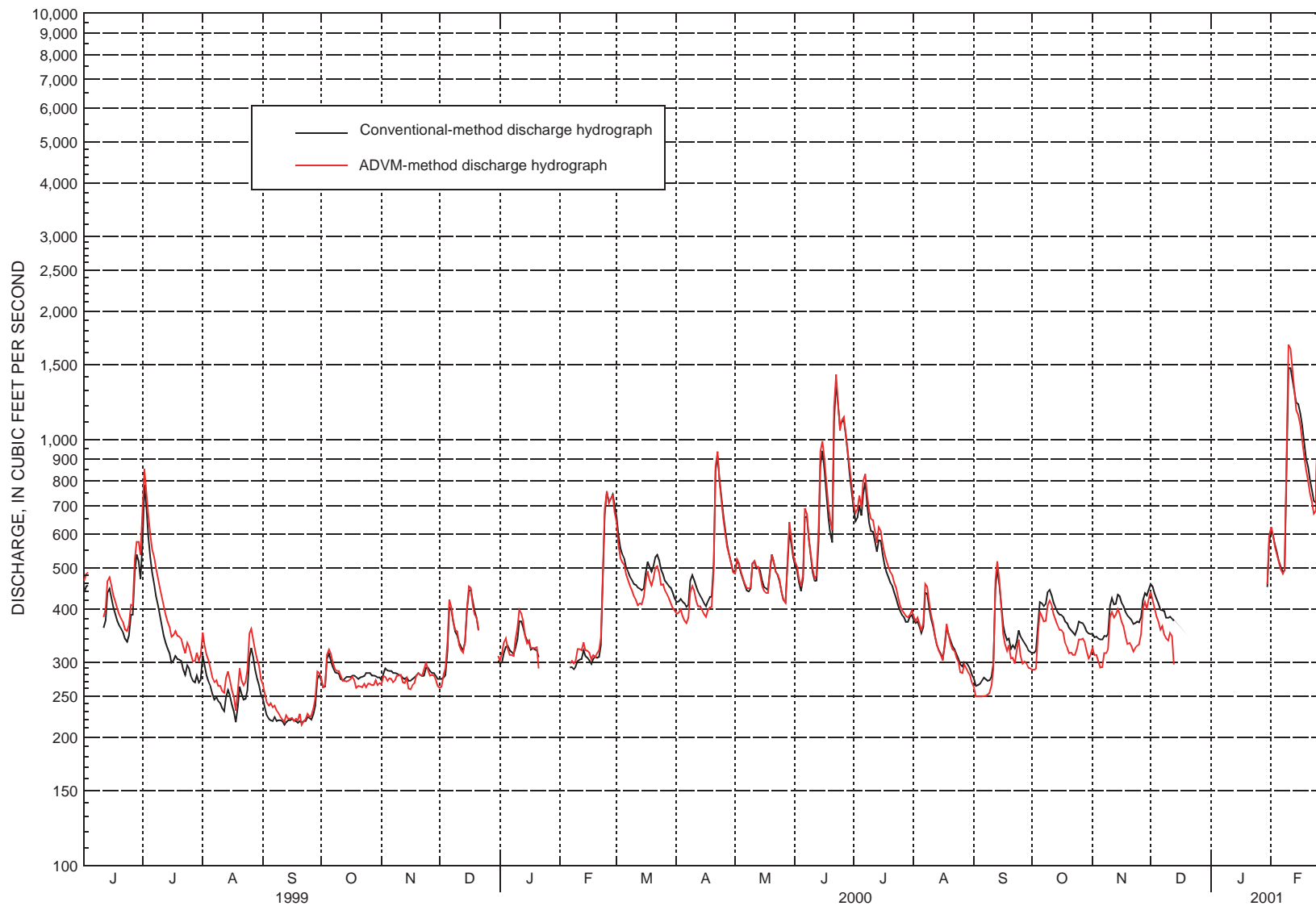
Figure 17. Comparison of mean-daily discharge hydrographs produced by conventional method and acoustic Doppler velocity meter (ADVM) methods from the Kankakee River at Davis, Ind., ADVM evaluation station, June 1, 1999–February 28, 2001 (Note: breaks in graph represent periods of missing data).
