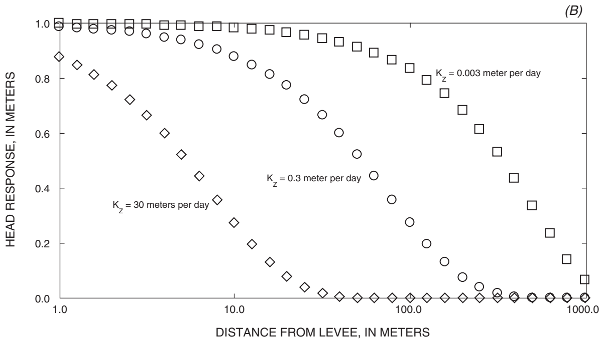
Figure 15. Hydrogeologic simulation of head change in aquifer capped with wetland peat responding to a change in water level at the left boundary (canal/levee complex). Schematic of simulated aquifer system (A), equilibrium head distribution after 1-meter rise in water level in canal at left boundary (B).
