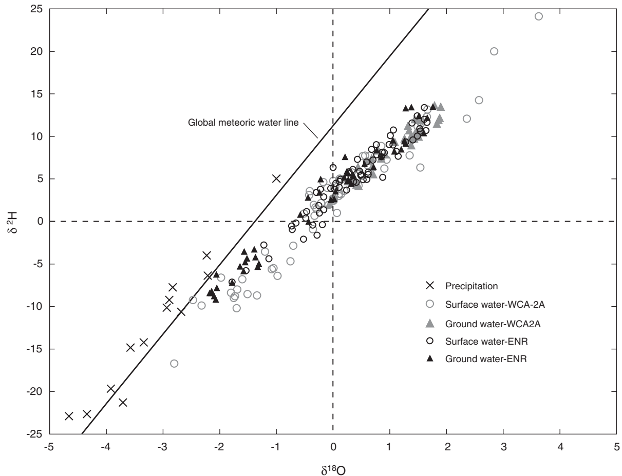
Figure 22. Water-stable isotopic ratios \delta^{2}\text{H} and \delta^{18}\text{O} from precipitation, surface water, and ground water in Everglades Nutrient Removal (ENR) project and Water Conservation Area 2A (WCA-2A), north-central Everglades, south Florida. Most isotopic values from ground water are relatively heavy (positive) on a trend with lower slope than the global meteoric water line, suggesting that appreciable evaporation occurred from that water. In contrast, precipitation and many surface-water samples are relatively light in isotopic value. Only a small group of ground-water samples are relatively light in isotopic value (negative). See text for interpretation.
