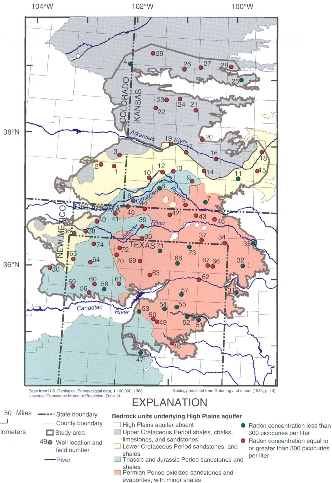
Figure 8. Radon concentration in samples collected in 1999 from 74 domestic water-supply wells completed in the central High Plains aquifer.
