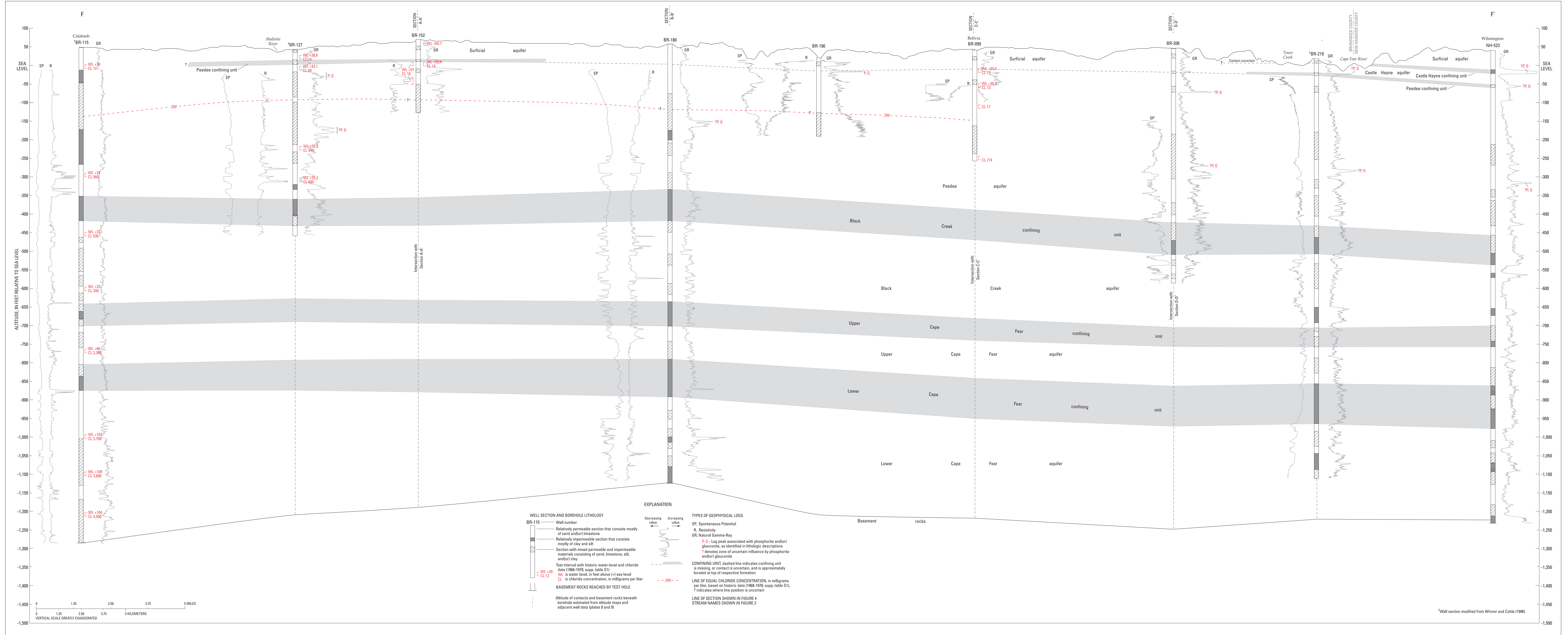
Plate 6. HYDROGEOLOGIC SECTION F-F', BRUNSWICK COUNTY, NORTH CAROLINA
