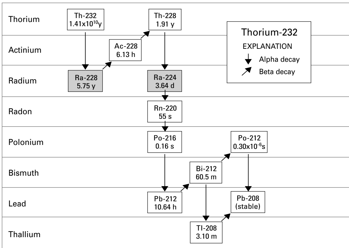
Figure 1. Diagram showing uranium-238 and thorium-232 radioactive decay series. (Radionuclides of interest in this study are shaded). [Times shown are half-lives: y, years; d, days; h, hours; m, minutes; s, seconds]. (From Hall and others, 1985.)
