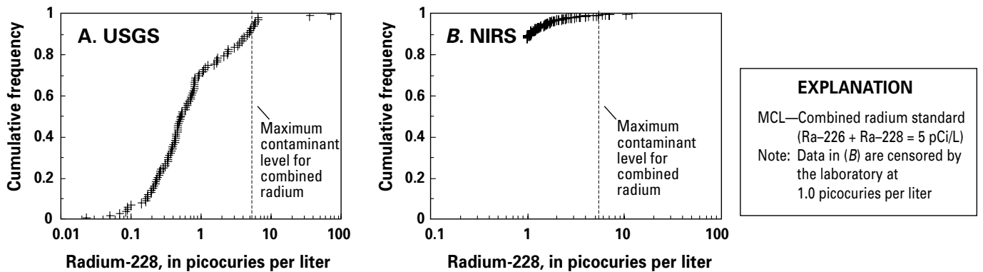
Figure 8. Cumulative frequency distributions for radium-228 in the 1998 U.S. Geological Survey (USGS) reconnaissance survey (A; targeted survey design) and radium-228 in the National Inorganics and Radionuclide Survey (NIRS) (B; random survey design). (MCL, maximum contaminant level.)
