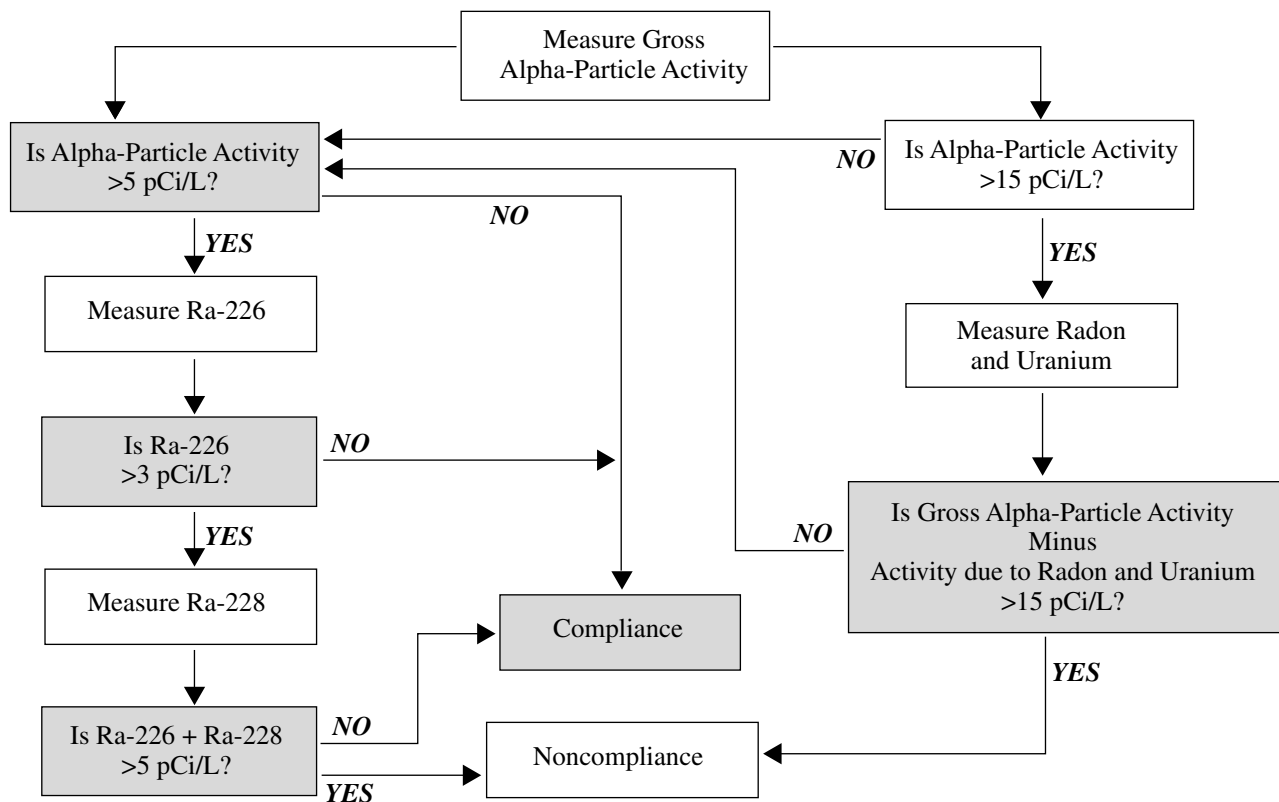
Figure 10. Schematic diagram showing the compliance monitoring scheme for radionuclides in public-drinking-water supplies. Shaded boxes emphasize where this, and other, studies have shown potential for errors in combined radium and short-term gross alpha-particle compliance monitoring. [Modified from Lappenbusch and Cothorn (1985).]
