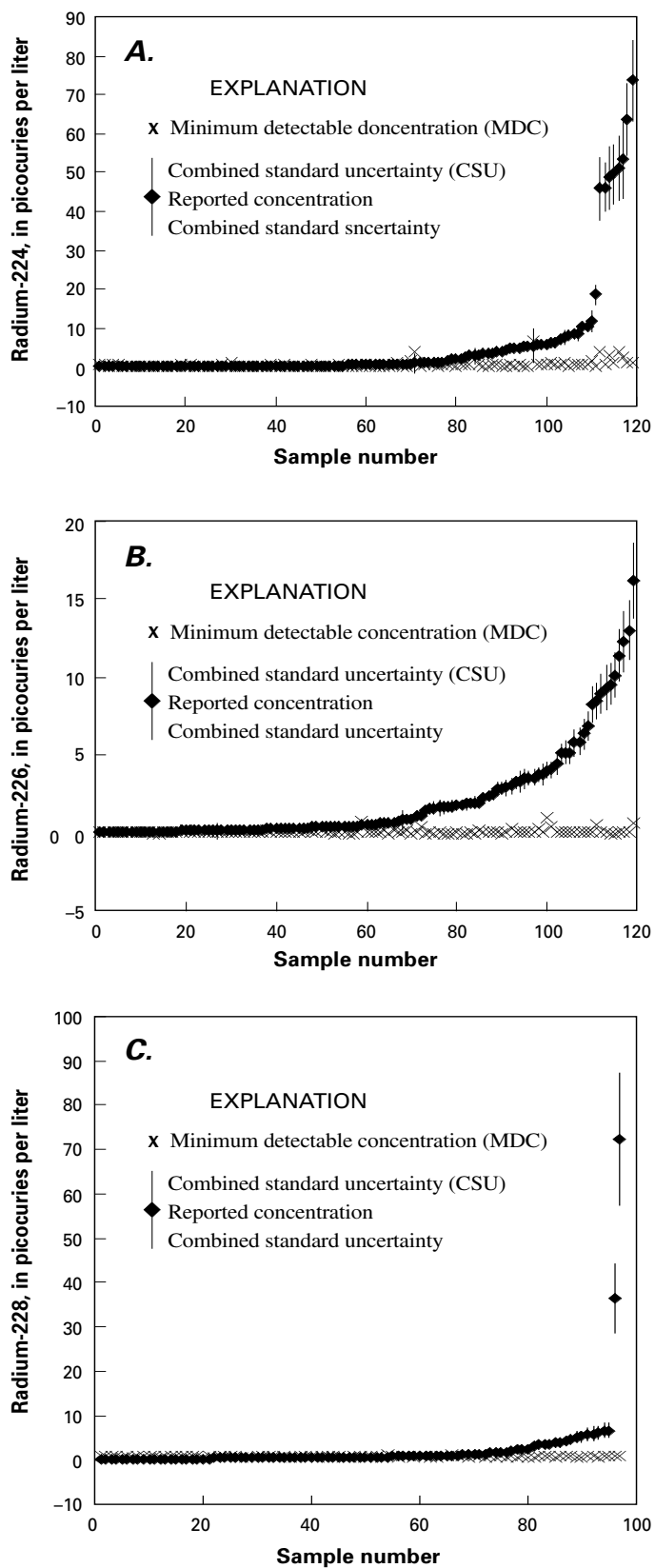
Figure 3. Graph showing reported concentrations, concentrations plus and minus the combined standard uncertainty (CSU), and the minimum detectable concentration (MDC) for Ra-224 (A), Ra-226 (B), and Ra-228 (C), for all samples including duplicates.
