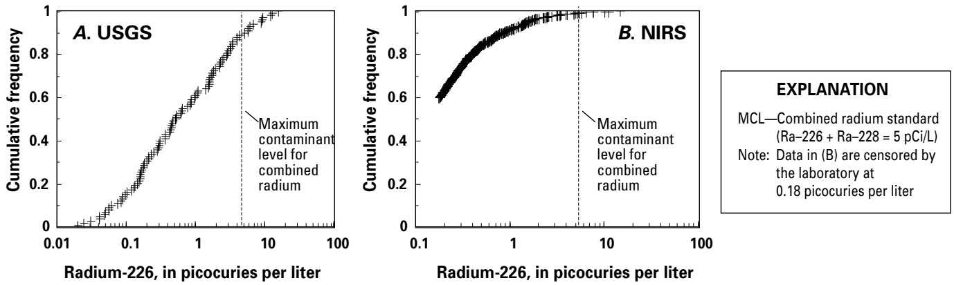
Figure 7. Cumulative frequency distributions for radium-226 in the 1998 U.S. Geological Survey (USGS) reconnaissance survey (A; targeted survey design) and in the National Inorganics and Radionuclide Survey (NIRS) (B; random survey design). (MCL, maximum contaminant level.)
