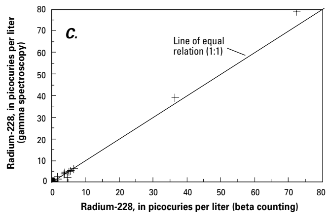
Figure 6. Duplicate environmental samples for radium-224 analyzed by alpha spectrometry and gamma spectrometry (A), and radium-226 analyzed by alpha spectrometry and gamma spectrometry (B), and radium-228 analyzed by beta counting and gamma spectrometry (C).
