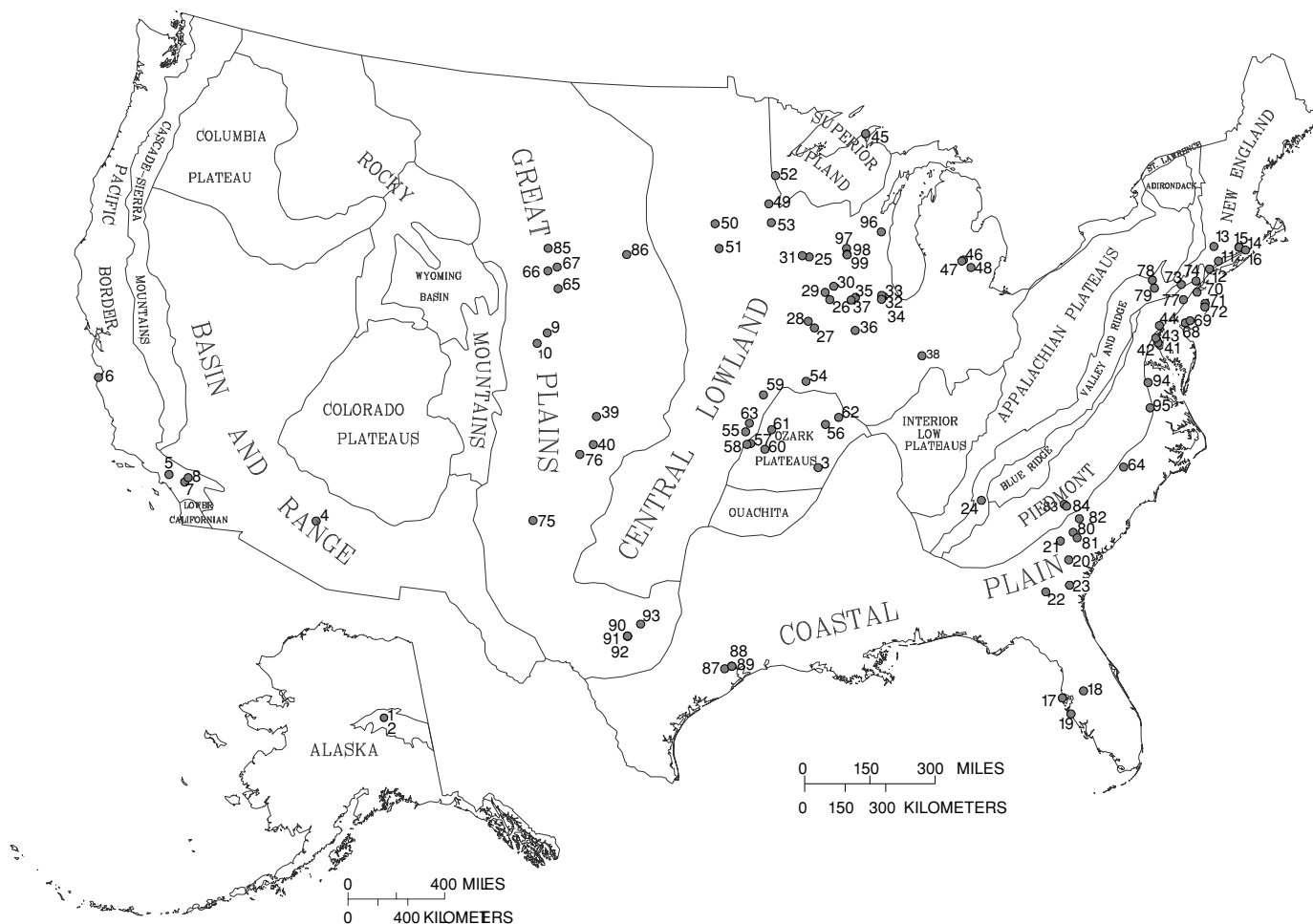
Figure 2. Major physiographic provinces of the United States and locations of wells with completed radium-224 analysis, 1998.
