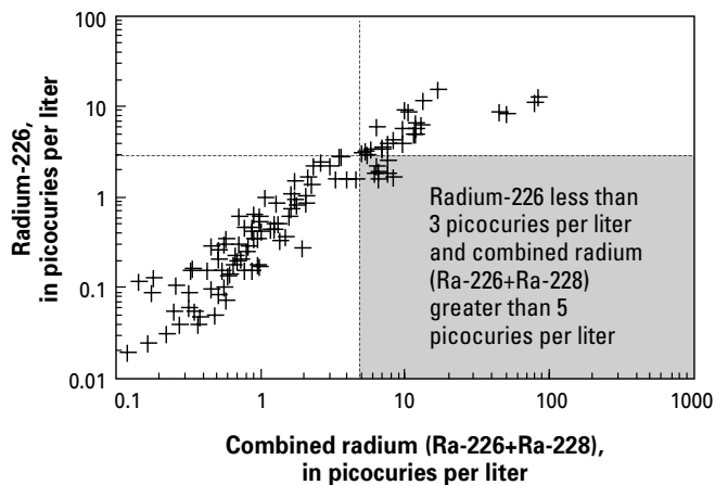
Figure 11. Graph showing relation between radium-226 and combined radium (radium-226 + radium-228) concentrations.
