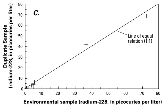
Figure 5. Environmental sample and duplicate environmental sample concentrations for radium-224 (A), radium-226 (B), and radium-228 (C).
