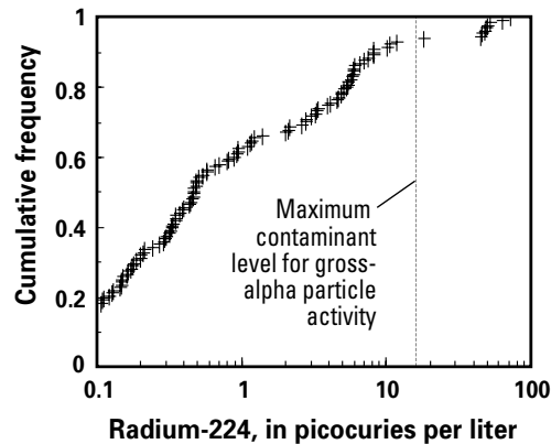
Figure 9. Cumulative frequency distribution for radium-224 in the 1998 U.S. Geological Survey Reconnaissance survey (targeted sampling design).
