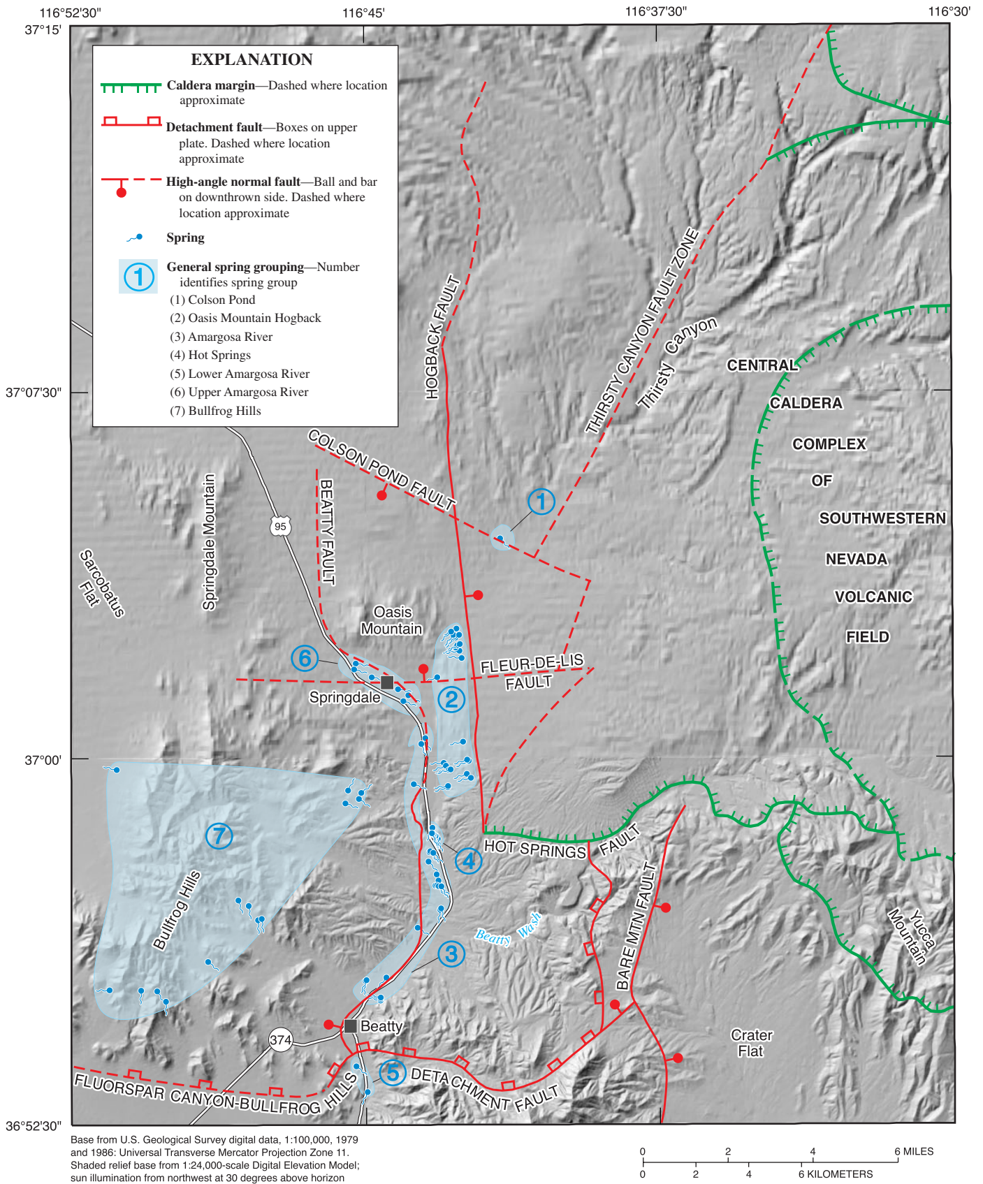
Figure 4. Major structural features controlling spring discharge in Oasis Valley, Nevada.
