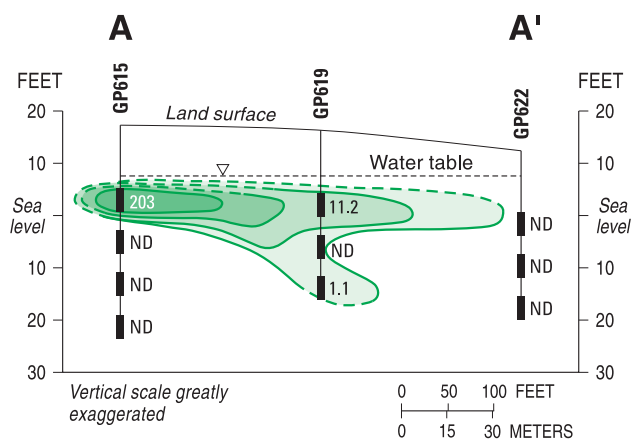
(c) cis -1,2-Dichloroethene
