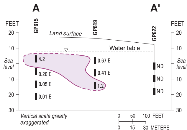
(b) Trichloroethene
