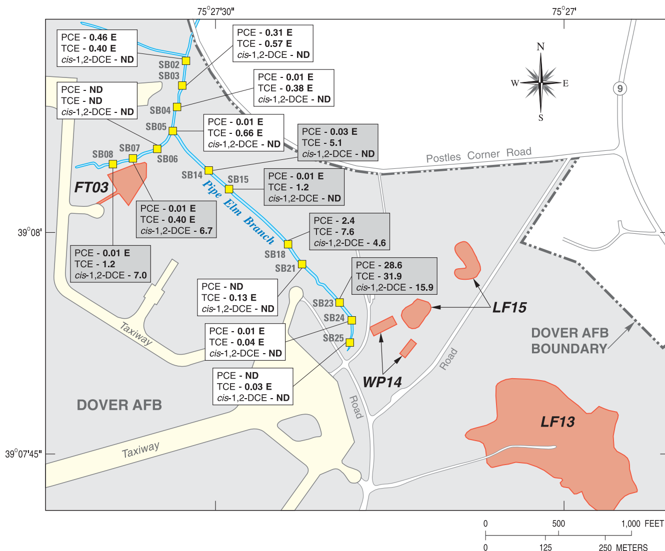
Figure 11. Distribution of tetrachloroethene, trichloroethene, and cis -1,2-dichloroethene in ground-water samples collected from the surficial aquifer underlying Pipe Elm Branch and the drainage ditch adjacent to site FT03 in the natural attenuation study area, Dover Air Force Base, Delaware, January 2001.
