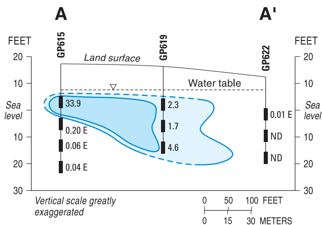
(a) Tetrachloroethene
