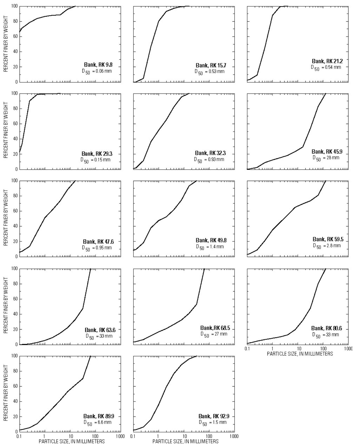
Appendix 2. Particle-size distribution, median diameter, and location of bank-material samples of the Alagnak River. (RK, river kilometer).
