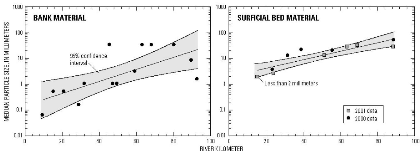
Figure 10. Downstream distribution of median particle size of bank material and surficial bed material in the Alagnak River. Regressions are significant at \alpha = 0.05 . R^2 is 0.49 for bank material and 0.68 for bed material.
