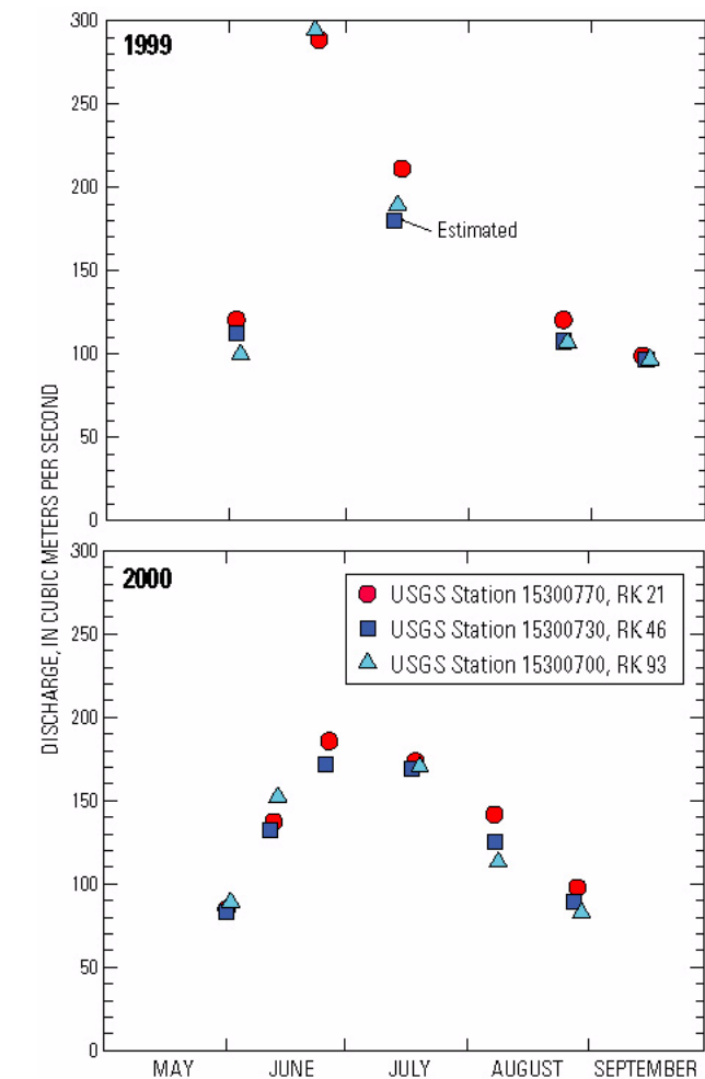
Figure 8. Measured discharge at Alagnak River river kilometer 21, 46, and 93 in 1999 and 2000.
