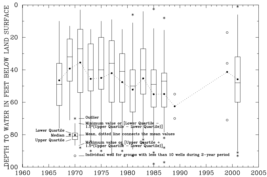
Figure C16. Glacial deposit ground-water levels reported in WellLogic database for Ann Arbor Township, Washtenaw County, Michigan.
