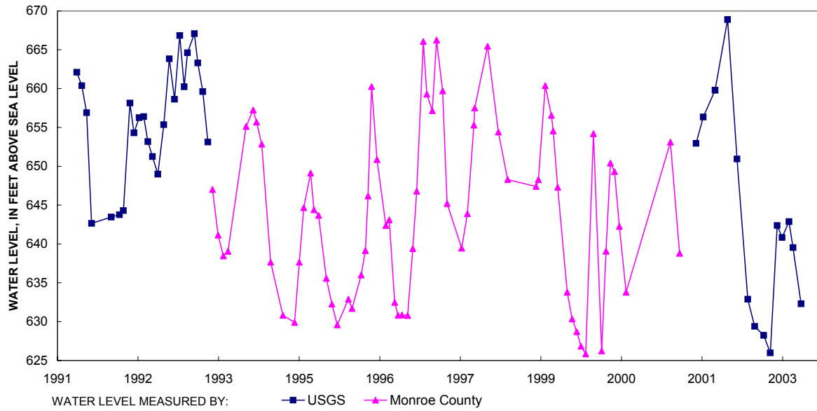
Figure A28. Ground-water levels for well G-28 Whiteford Township, Monroe County, Michigan.
