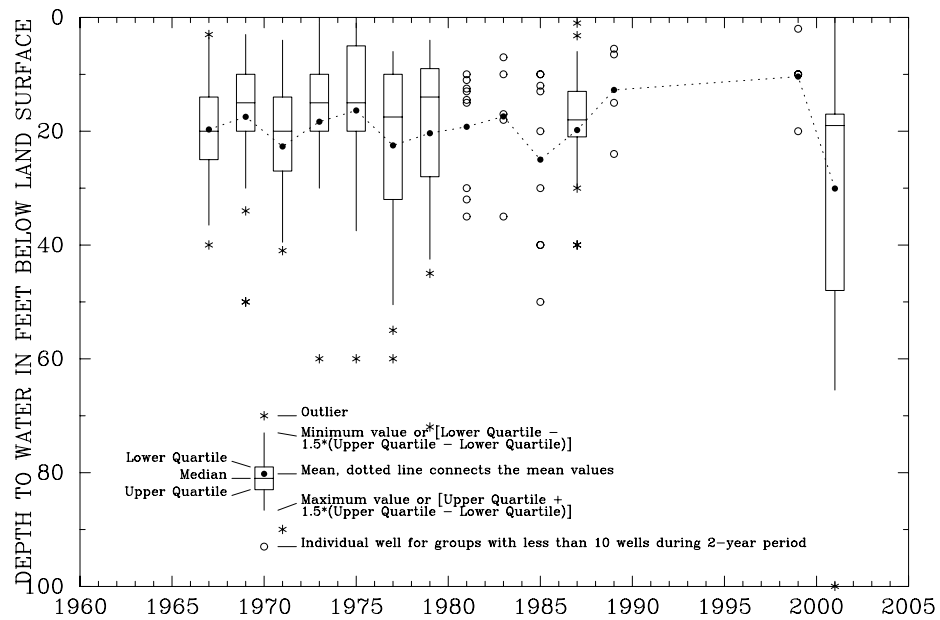
Figure C17. Glacial deposit ground-water levels reported in WellLogic database for Augusta Township, Washtenaw County, Michigan.
