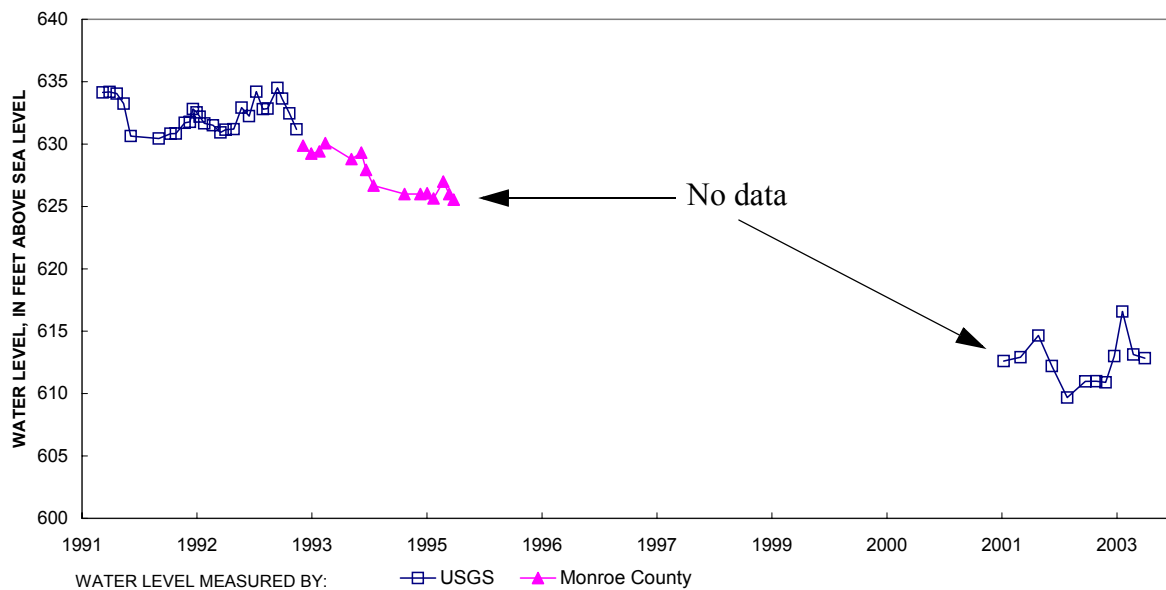
Figure A21. Ground-water levels for well G-21 Summerfield Township, Monroe County, Michigan.
