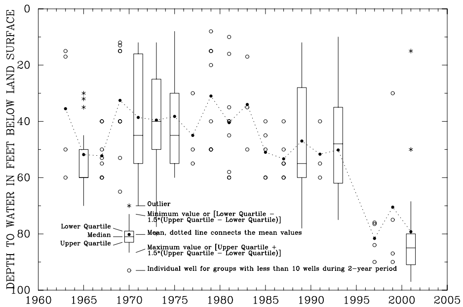
Figure C11. Bedrock aquifer ground-water levels reported in WelLogic database for Milan Township, Monroe County, Michigan.
