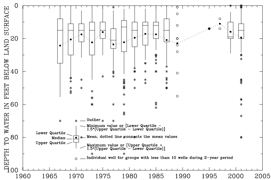
Figure C25. Glacial deposit ground-water levels reported in WellLogic database for Northfield Township, Washtenaw County, Michigan.
