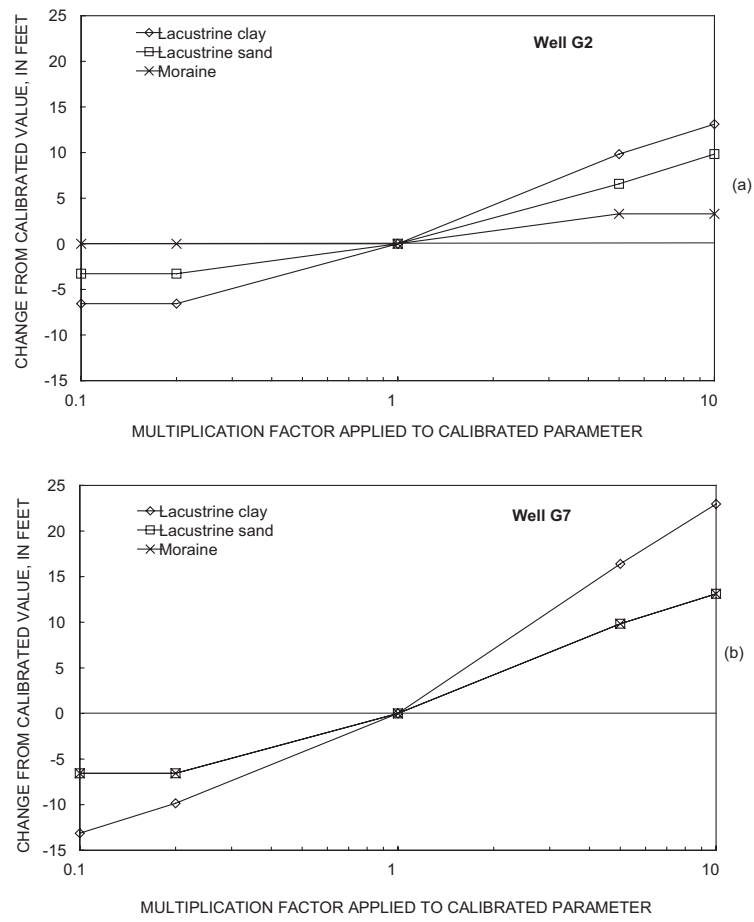
Figure 32. Change in hydraulic head for 2001 simulation at (a) G2, (b) G7, from varying model parameters.
