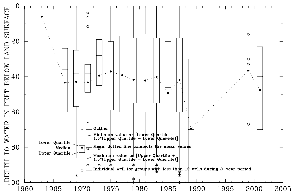
Figure C29. Glacial deposit ground-water levels reported in WellLogic database for Scio Township, Washtenaw County, Michigan.
