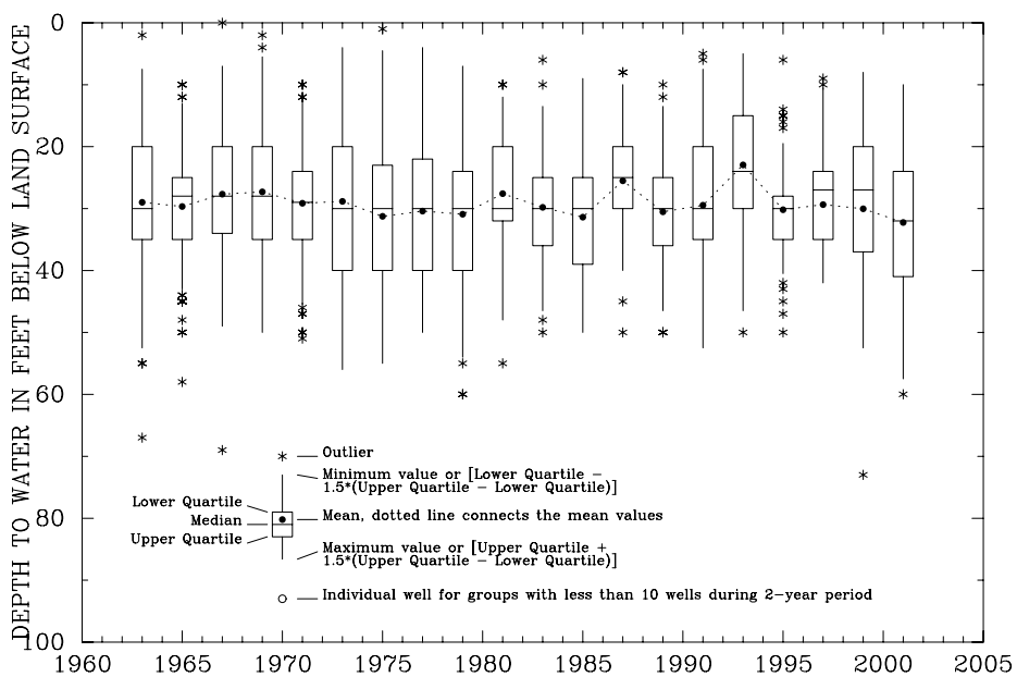
Figure C2. Bedrock aquifer ground-water levels reported in WellLogic database for Bedford Township, Monroe County, Michigan.
