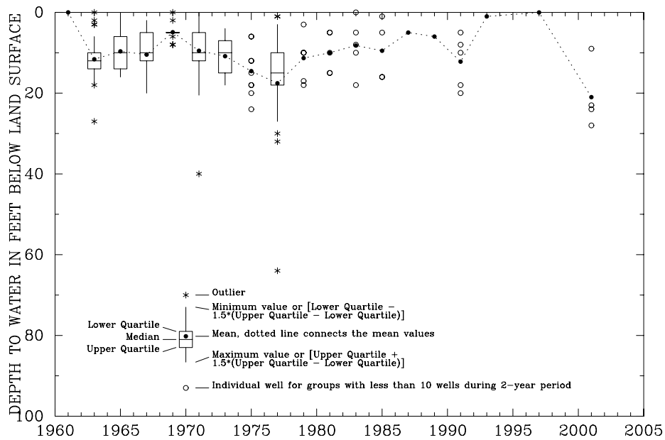
Figure C12. Bedrock aquifer ground-water levels reported in WelLogic database for Monroe Township, Monroe County, Michigan.
