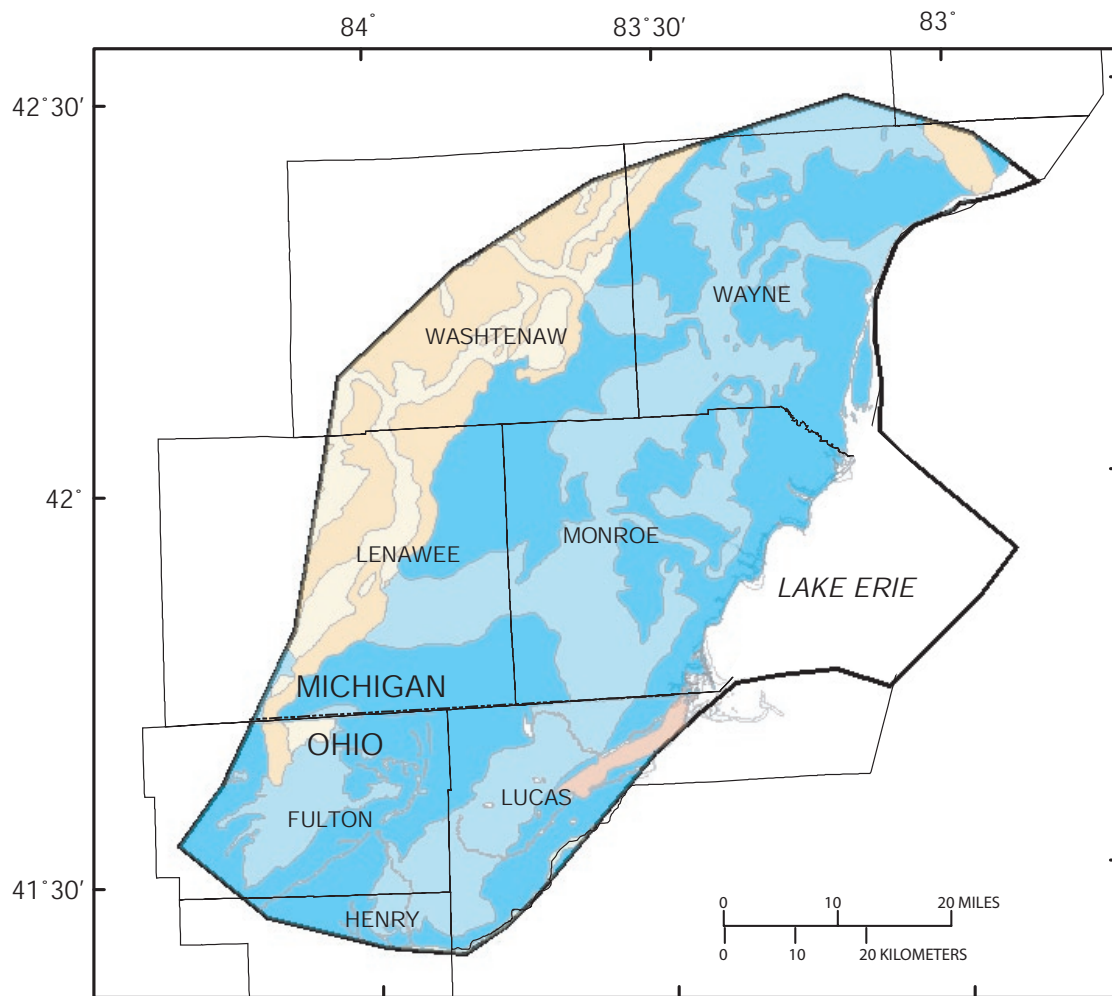
Figure 3. Generalized glacial deposit map for study area, modified from Ferrand and Bell (1982) and Ohio Department of Natural Resources (2000b).
