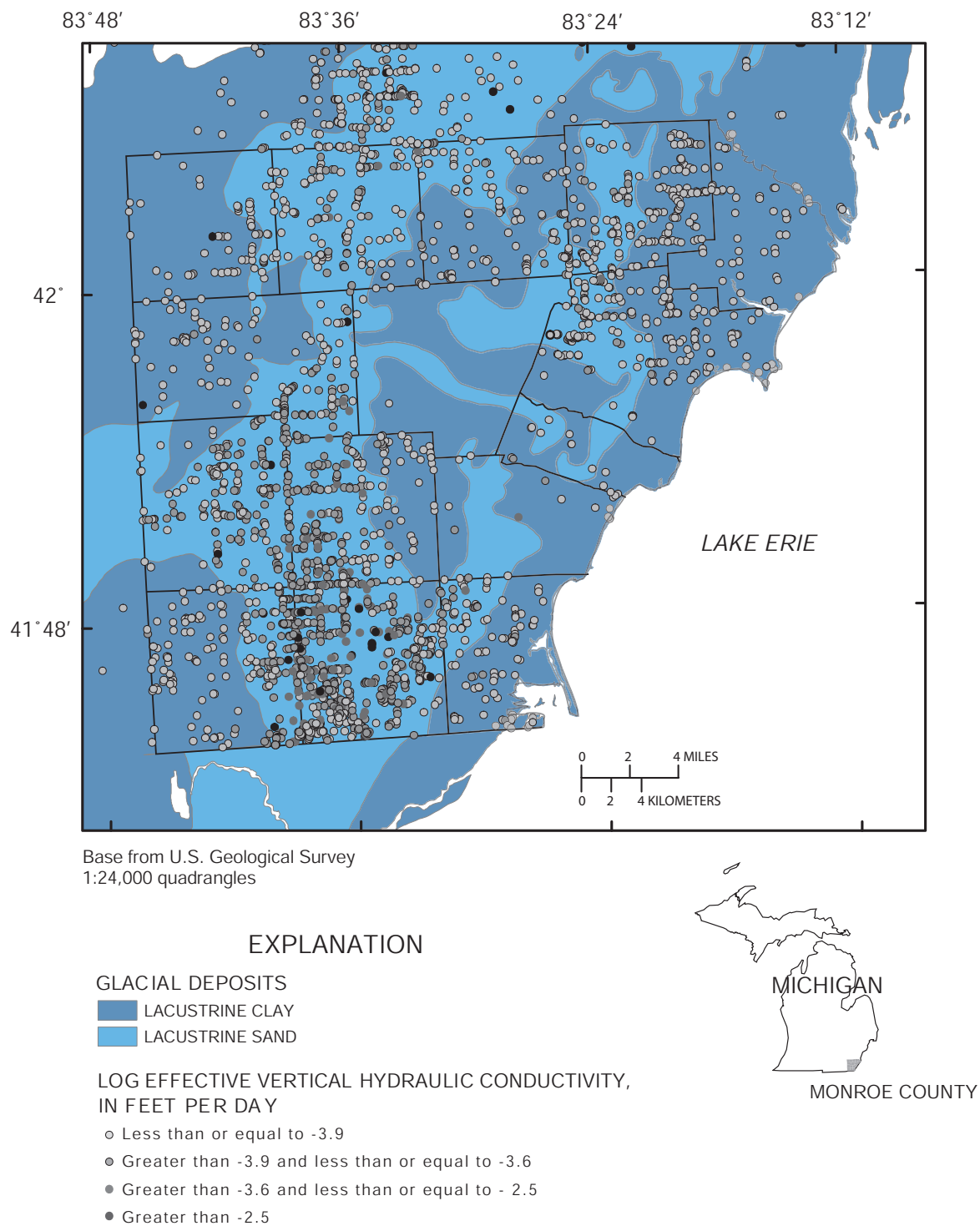
Figure 4. Estimated \log(K_v^{eff}) for Monroe County, Michigan, based on thickness and lithology of units reported in the WelLogic database. Shaded areas are glacial deposits mapped by Ferrand and Bell (1982).
