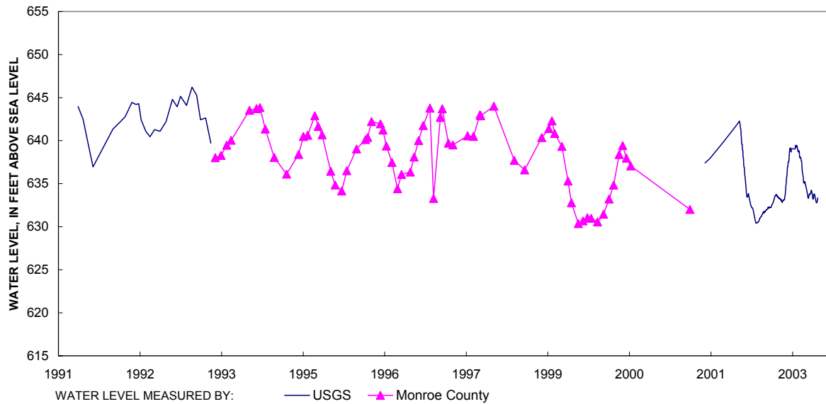
Figure A29. Ground-water levels for well G-29 Whiteford Township, Monroe County, Michigan.
