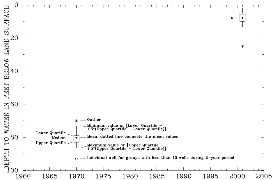
Figure C9. Bedrock aquifer ground-water levels reported in WelLogic database for Lasalle Township, Monroe County, Michigan.
