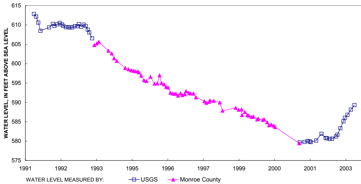
Figure A8. Ground-water levels for well G-8 London Township, Monroe County, Michigan.
