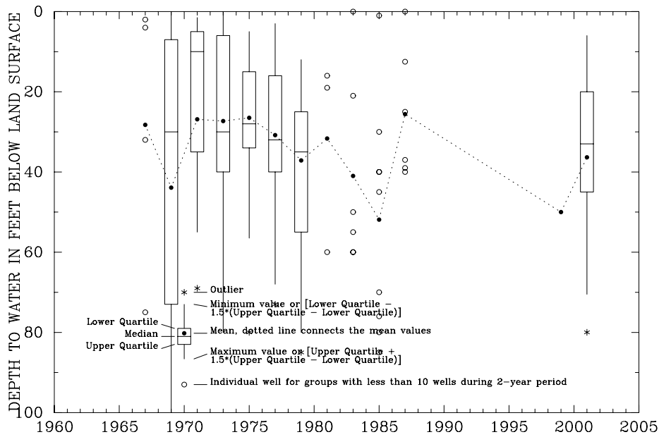
Figure C28. Glacial deposit ground-water levels reported in WellLogic database for Saline Township, Washtenaw County, Michigan.
