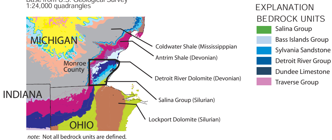
Figure 6. Bedrock units for Monroe County, Michigan and regional bedrock setting from Milstein (1987), Indiana Geological Survey (2002), Ohio Department of Natural Resources (2000a).
