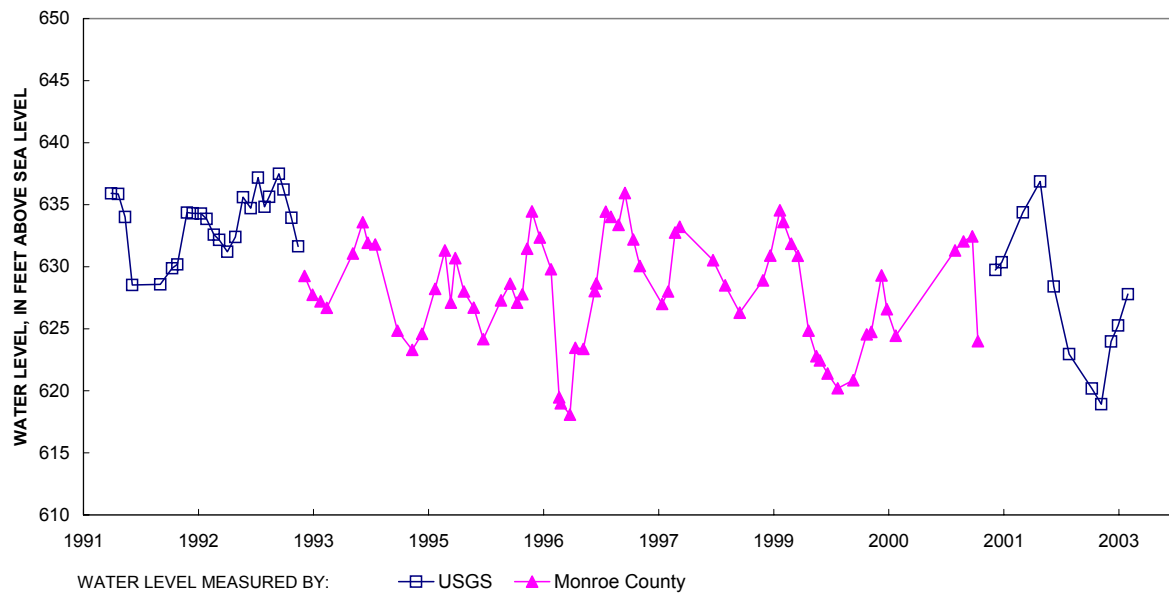
Figure A20. Ground-water levels for well G-20 Ida Township, Monroe County, Michigan.
