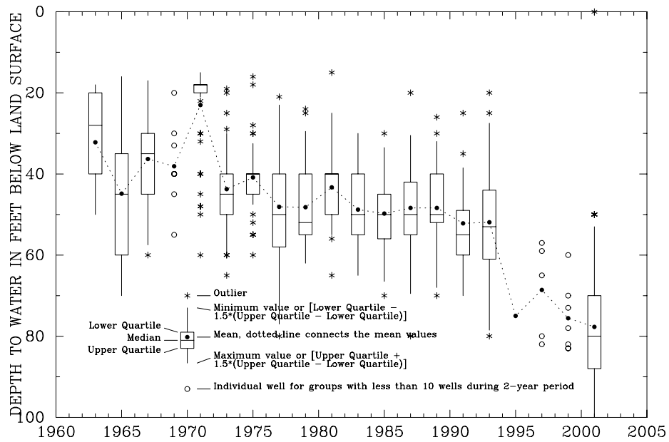
Figure C10. Bedrock aquifer ground-water levels reported in WelLogic database for London Township, Monroe County, Michigan.
