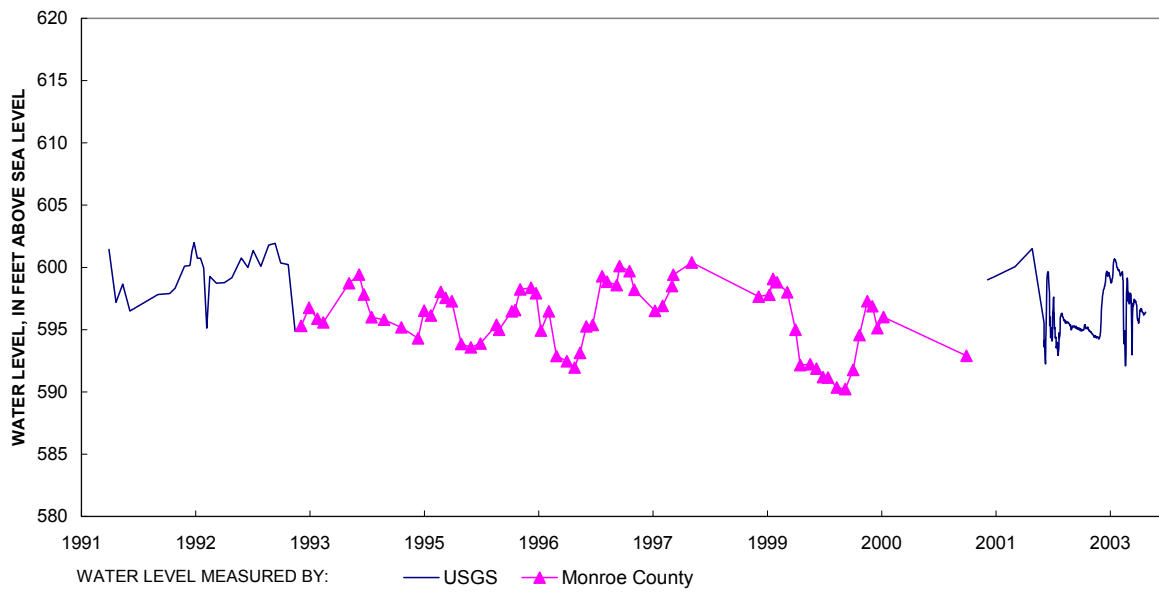
Figure A32. Ground-water levels for well G-32 Erie Township, Monroe County, Michigan.
