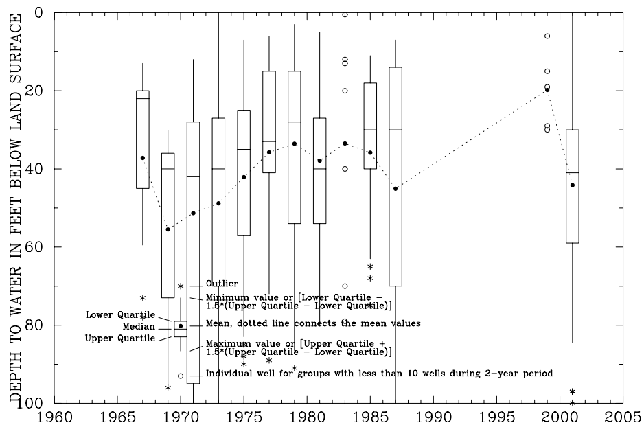
Figure C24. Glacial deposit ground-water levels reported in WellLogic database for Manchester Township, Washtenaw County, Michigan.
