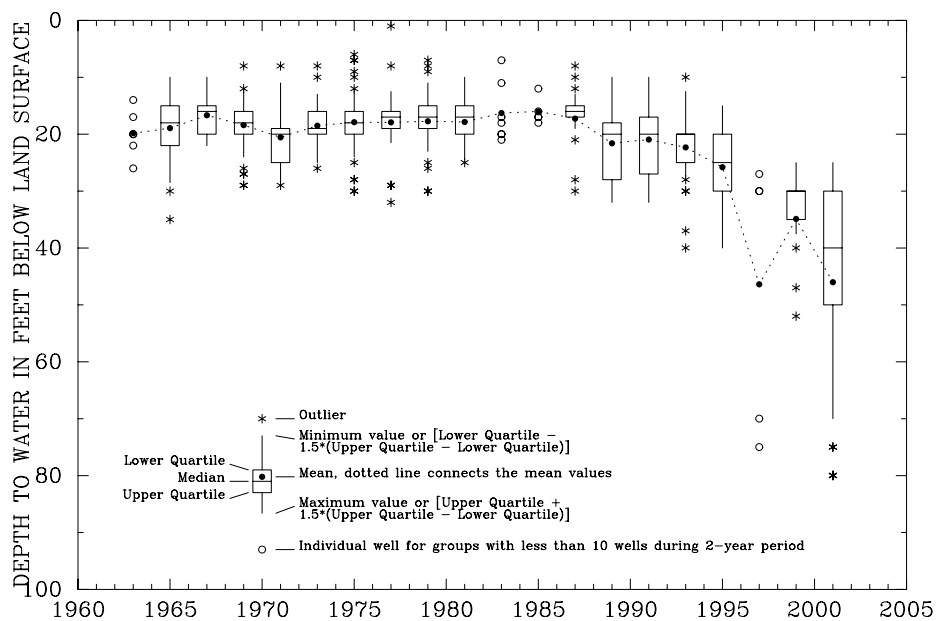
Figure C1. Bedrock aquifer ground-water levels reported in WellLogic database for Ash Township, Monroe County, Michigan.
