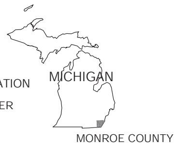
Figure 2. U.S. Geological Survey streamflow-gaging stations and monitoring wells in Monroe County, Michigan.
