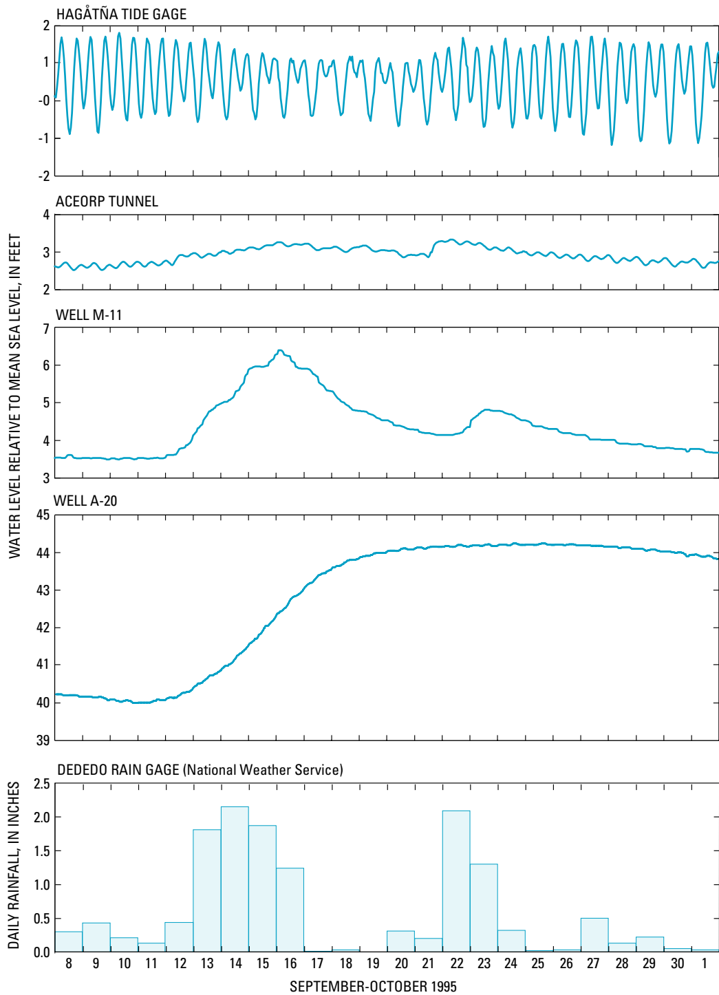
Figure 7. Tides at Hagåtña tide gage, water-level response in selected wells, and rainfall at Dededo rain gage (September 8 to October 1, 1995) Guam. (Dededo data from National Climatic Data Center, 2000)
