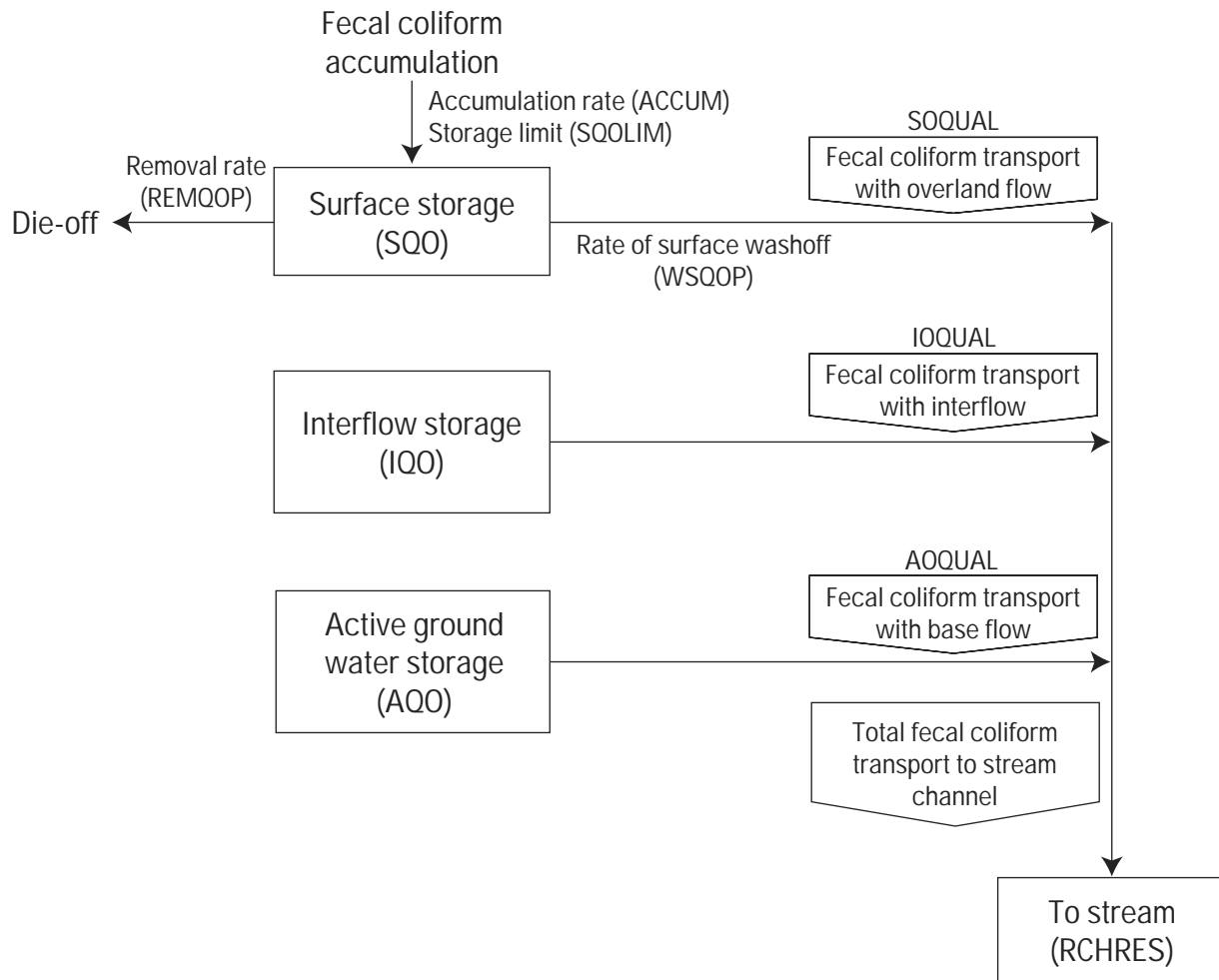
Figure 4. Routing processes represented by the Hydrological Simulation Program-FORTRAN for the simulation of fecal coliform bacteria transport in Blacks Run, Rockingham County, Virginia. (See table 5 for definition of fecal coliform bacteria transport and storage parameters.)
