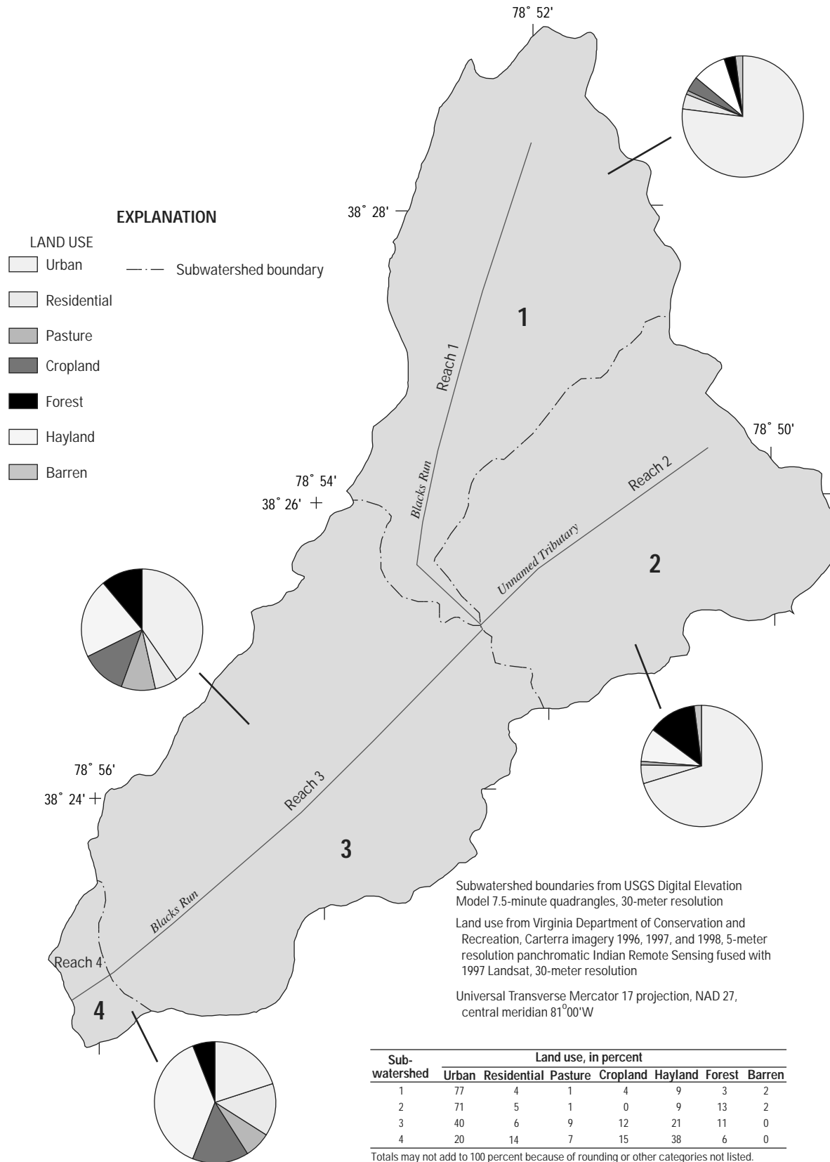
Figure 3. Hydrologic subwatersheds, land use, and reaches as represented in the streamflow and fecal coliform models for Blacks Run, Rockingham County, Virginia.
