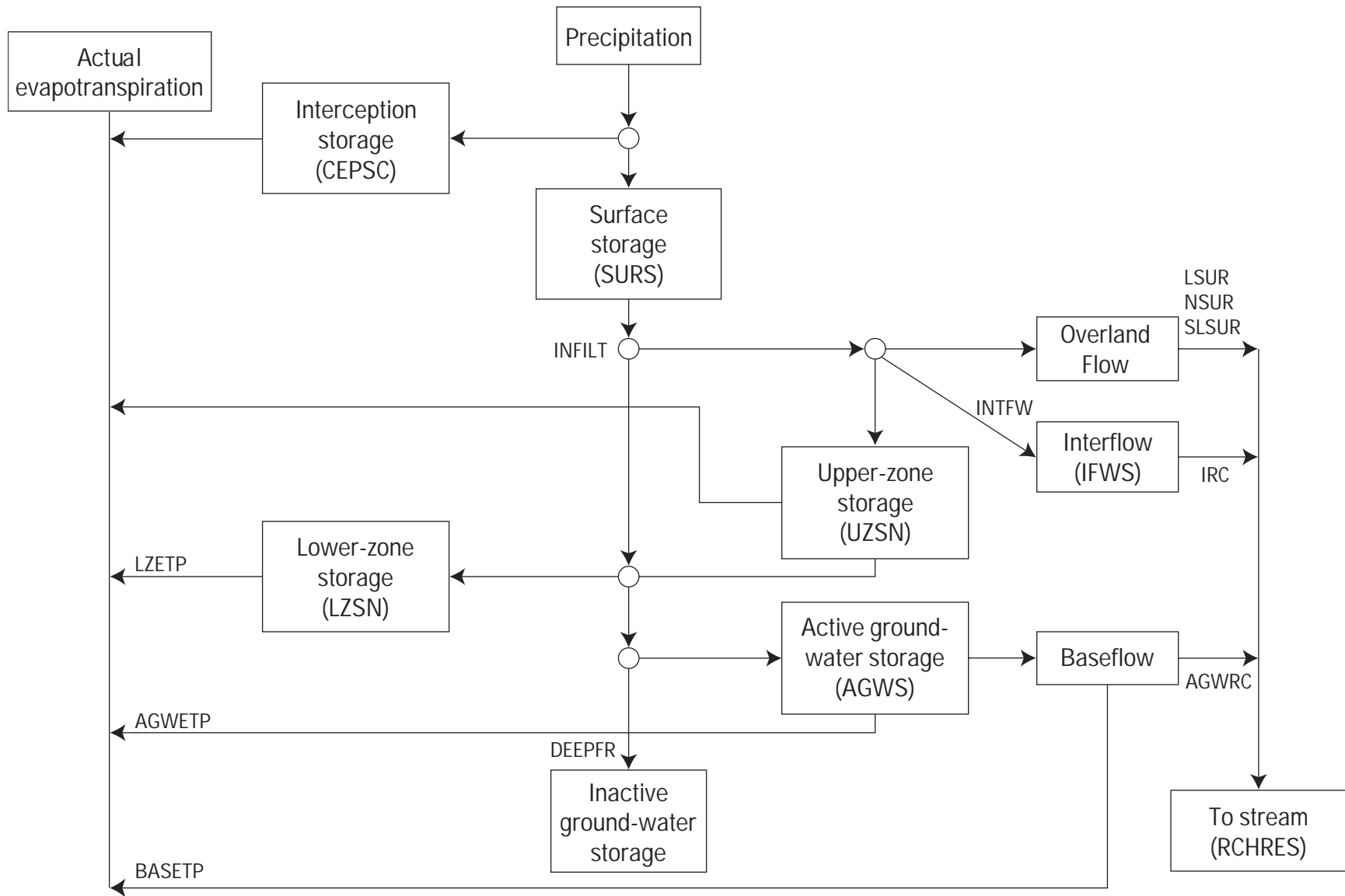
Figure 2. Rainfall-routing processes, associated with pervious land segments, represented by the Hydrological Simulation Program-FORTRAN for the simulation of streamflow in Blacks Run, Rockingham County, Virginia. (See table 1 for definition of hydrologic parameters.)
