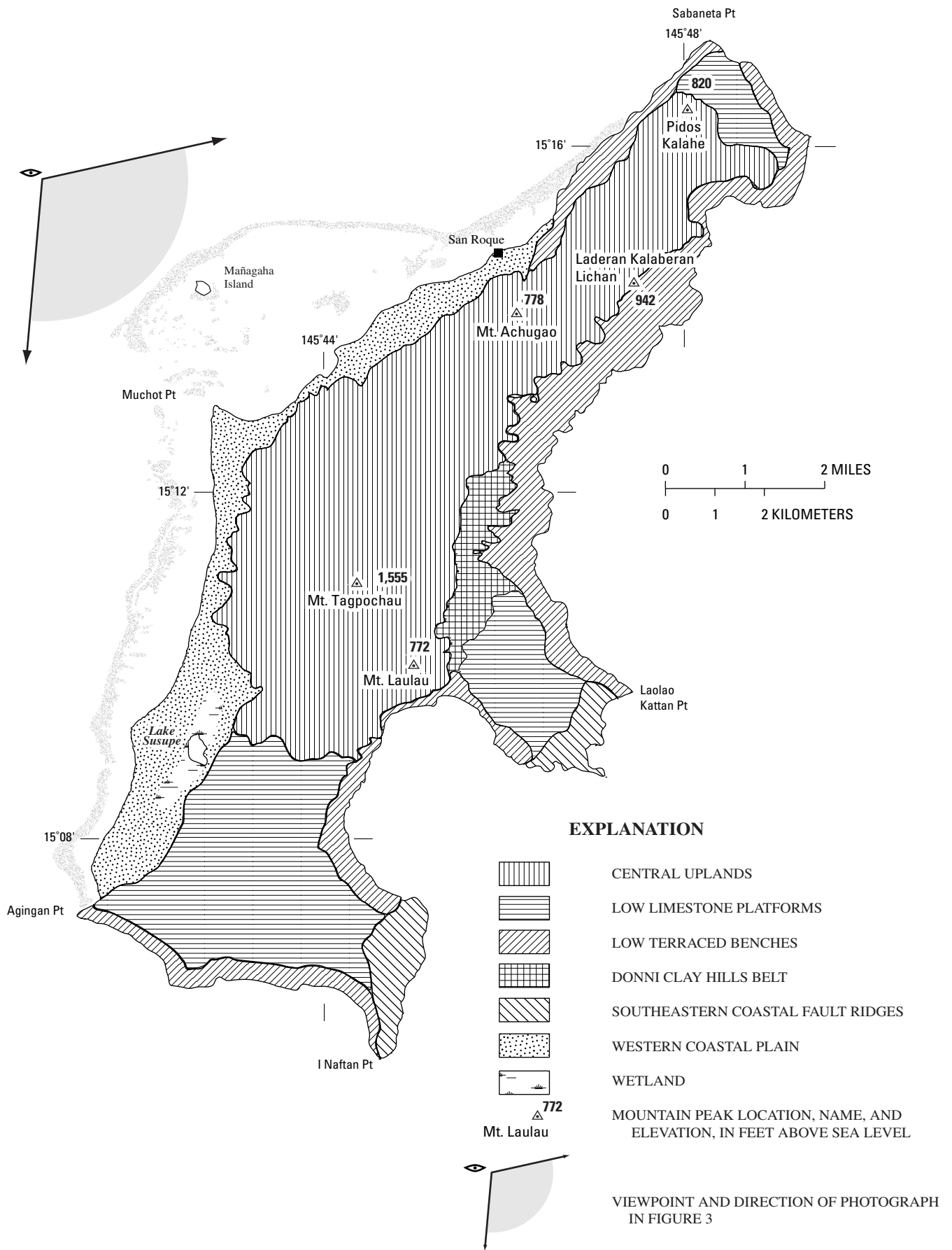
Figure 2. Physiographic subdivisions of Saipan (modified from Cloud and others, 1956).
