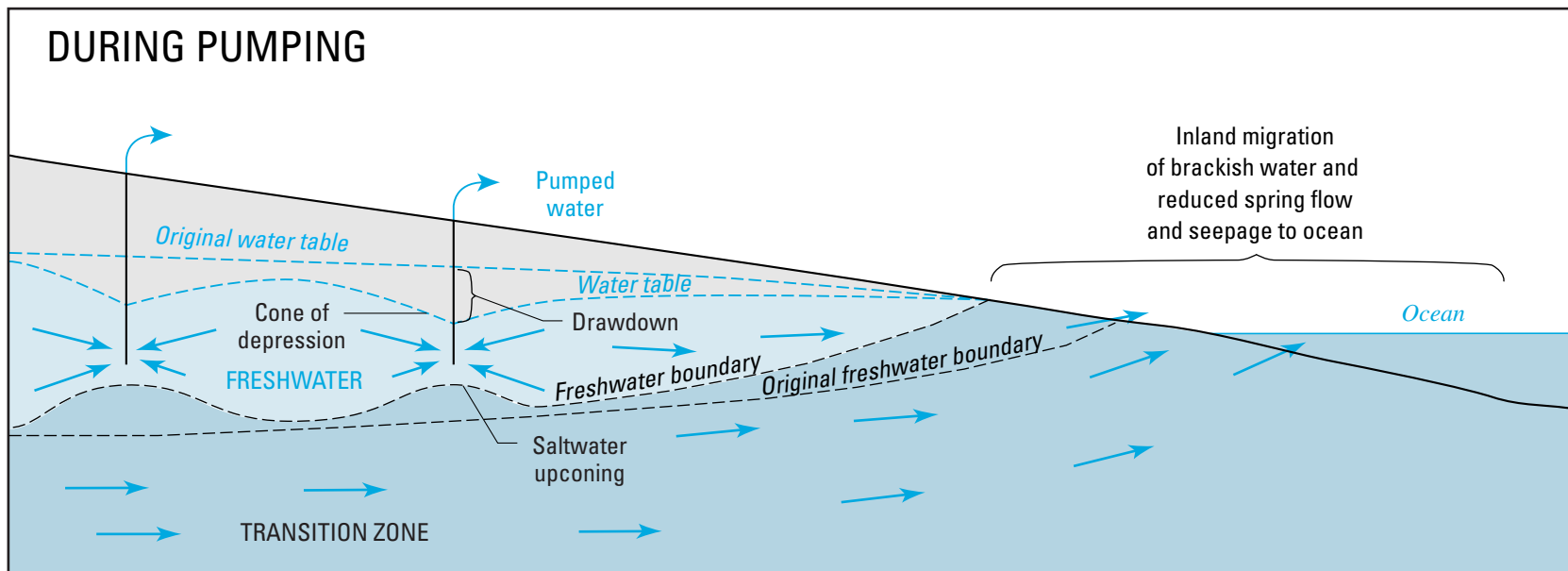
Figure 6. Effects of ground-water withdrawal on the potable part of the freshwater lens in a high permeability island aquifer.
