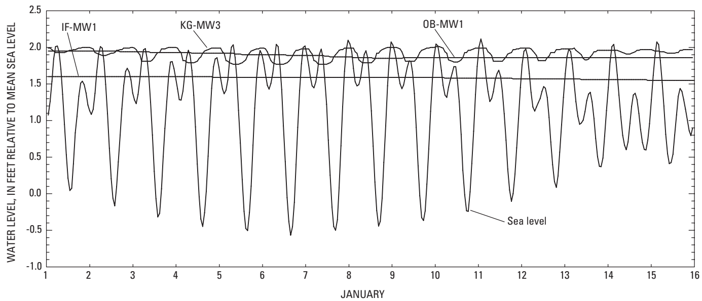
Figure 10. Selected hourly ground-water levels and sea level, Saipan, January 1-15, 1999. Sea-level data from the University of Hawaii Sea Level Center (UHSLC).
