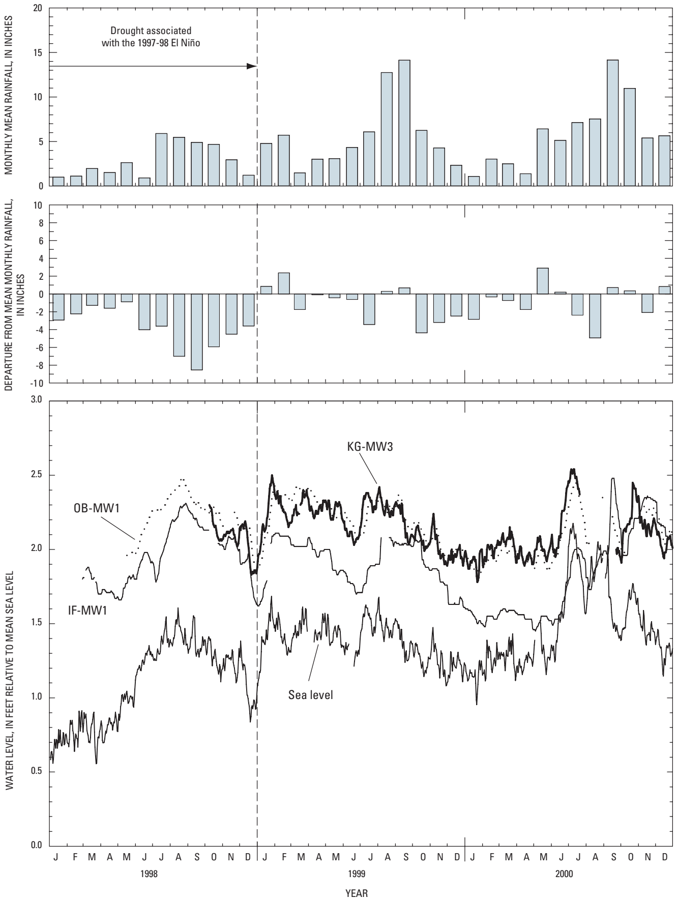
Figure 11. Monthly mean rainfall of all Saipan stations and selected daily mean ground-water levels and sea level, Saipan, 1998-2000. Sea-level data from the University of Hawaii Sea Level Center (UHSLC).
