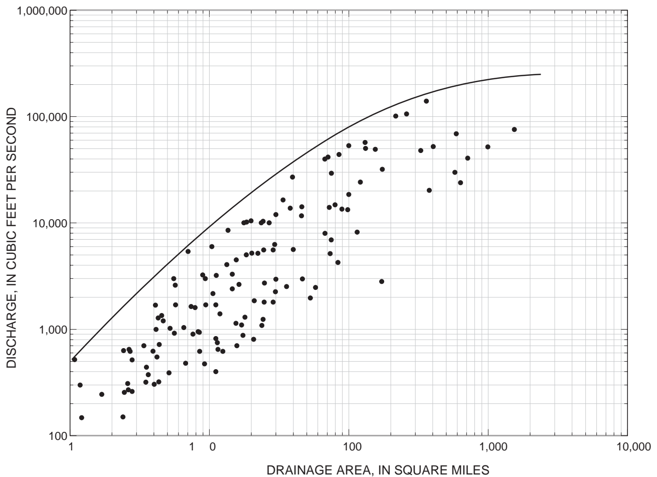
Figure 5. Relation of discharge for 100-year recurrence interval to drainage area for streamflow-gaging stations in Connecticut. (Curve defines the upper boundary of the 100-year peak-flow estimates.)
