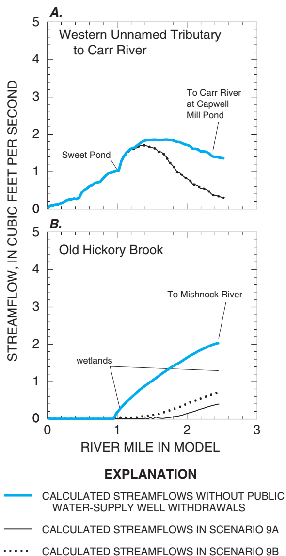
Figure 27. Model-calculated steady-state streamflows and streamflow depletions in scenarios 9A and 9B for the (A) western unnamed tributary to the Carr River and (B) Old Hickory Brook, Rhode Island. (Streamflows calculated for model cells along the centerlines of on-stream ponds were used.)
