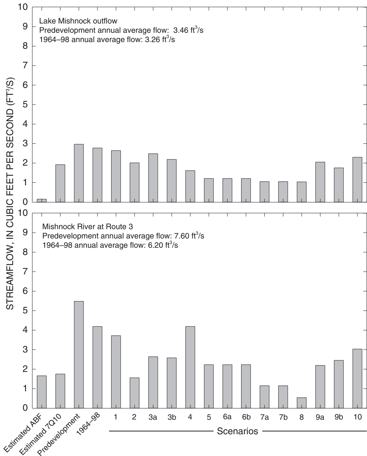
Figure 26. Model-calculated monthly average August streamflow at the Lake Mishnock outfall, the Mishnock River at Route 3, the Carr River above Capwell Mill Pond, and the Big River at Hill Farm Road for the predevelopment conditions, conditions during 1964–98, and 14 withdrawal scenarios, Big River study area, Rhode Island. (Location of streamflow sites shown on fig. 23; withdrawal scenarios described in table 10.)
