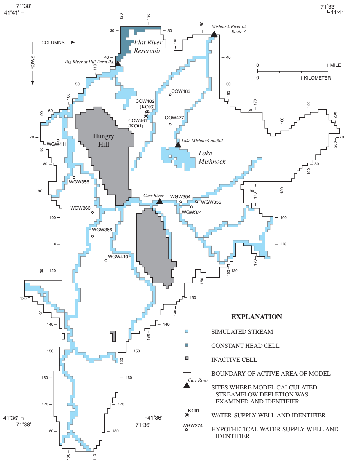
Figure 23. Location of current and hypothetical ground-water-development sites and streamflow sites selected for examination of streamflow depletion in the Big River study area, Rhode Island.
