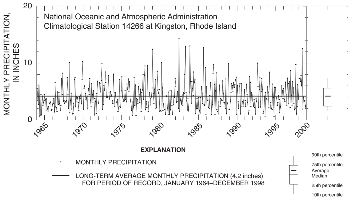
Figure 3. Record of total monthly precipitation and distribution of monthly precipitation measurements for the National Oceanic and Atmospheric Administration climatological station 14266, Kingston, Rhode Island, 1964–98. (Location of climatological station shown on fig. 2.)
