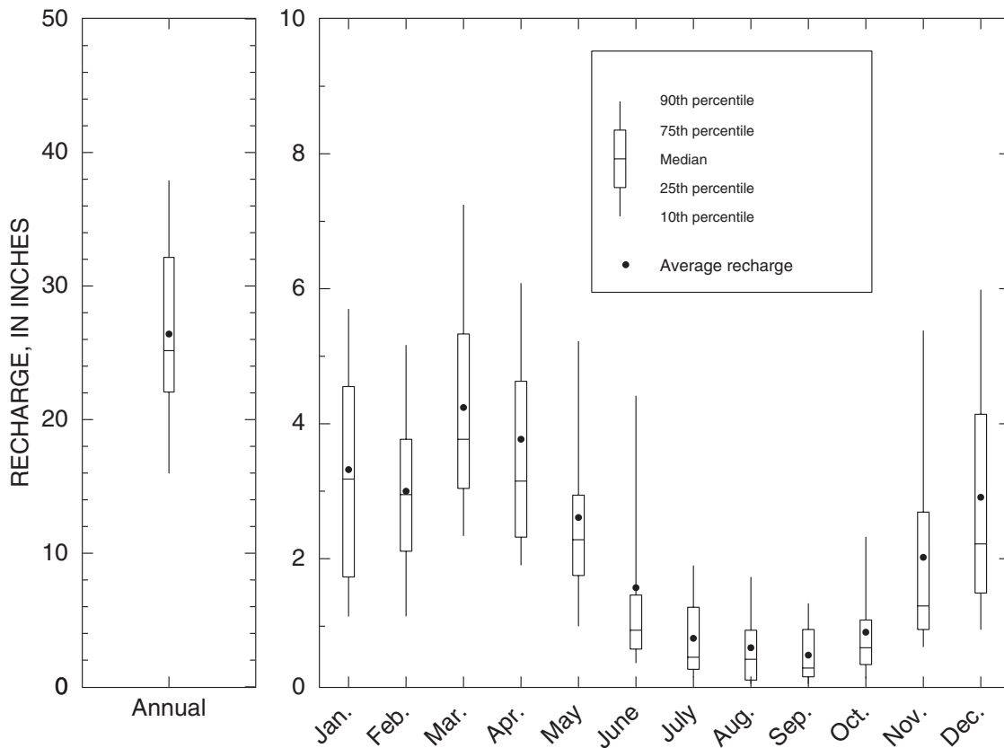
Figure 15. Distributions of annual and monthly recharge estimated from streamflow records for the Hunt River near East Greenwich, Rhode Island, 1964–98.
