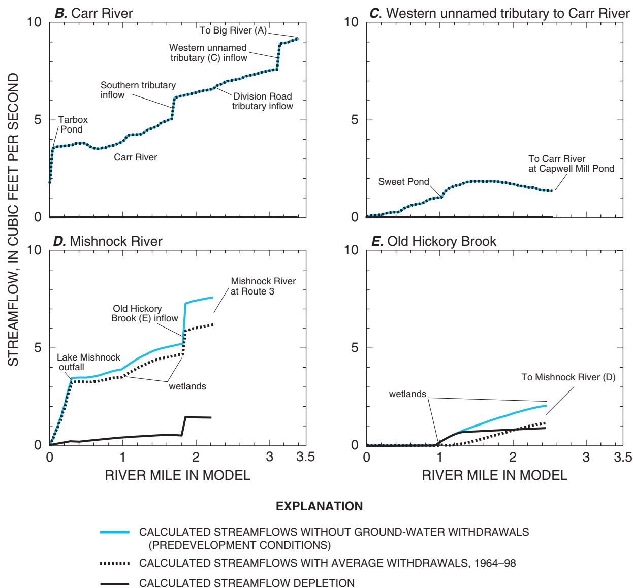
Figure 21—Continued. Model-calculated steady-state streamflows and streamflow depletions for the 1964–98 period in the (A) Congdon and Big Rivers, (B) Carr River, (C) western unnamed tributary to the Carr River, (D) Mishnock River, and (E) Old Hickory Brook, Rhode Island. (For on-stream ponds, streamflows were calculated for model cells along the centerline of the ponds.)
