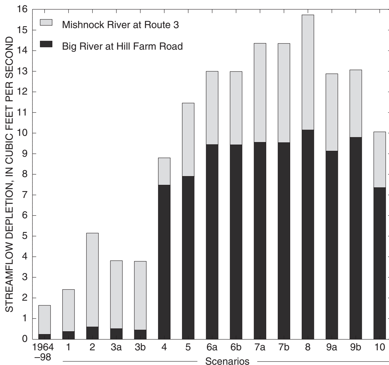
Figure 25. Total model-calculated steady-state streamflow depletion for the Mishnock River Basin (at Route 3), and the Big River Basin (at Hill Farm Road) for conditions during 1964–98 and 14 withdrawal scenarios, Big River study area, Rhode Island. (Location of streamflow index sites shown on fig. 23; withdrawal scenarios described in table 10.)
