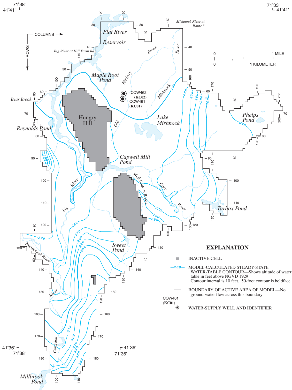
Figure 18. Model-calculated steady-state water table, Big River study area, Rhode Island.
