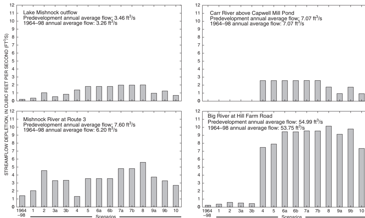
Figure 24. Model-calculated steady-state streamflow depletion at the Lake Mishnock outfall, Mishnock River Basin (at Route 3), Carr River above Capwell Mill Pond, and the Big River Basin (at Hill Farm Road) for conditions during 1964–98 and 14 withdrawal scenarios, Big River study area, Rhode Island. (Location of streamflow index sites shown on fig. 23; withdrawal scenarios described in table 10.)
