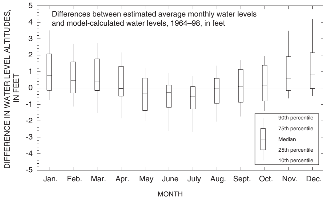
Figure 19. Distribution of differences between estimates of average monthly water levels during 1964–98 and model-calculated water levels, in feet, at the 21 well sites used for model calibration in the Big River study area, Rhode Island. (Well locations shown on fig. 4.)
