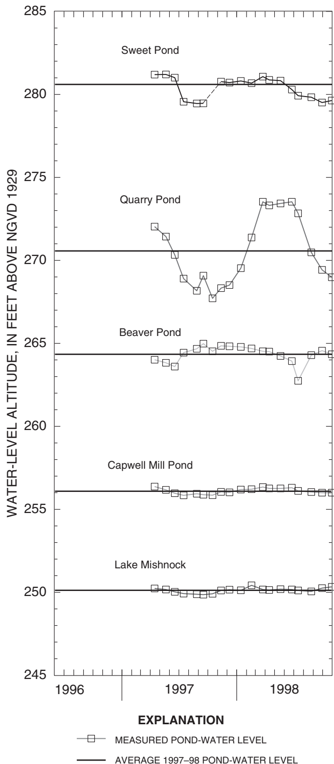
Figure 8. Water-level altitude measurements and the average of water-level altitudes measured at selected ponds in the Big River study area, Rhode Island, 1996–98. (Pond gage locations shown on fig. 4.)
