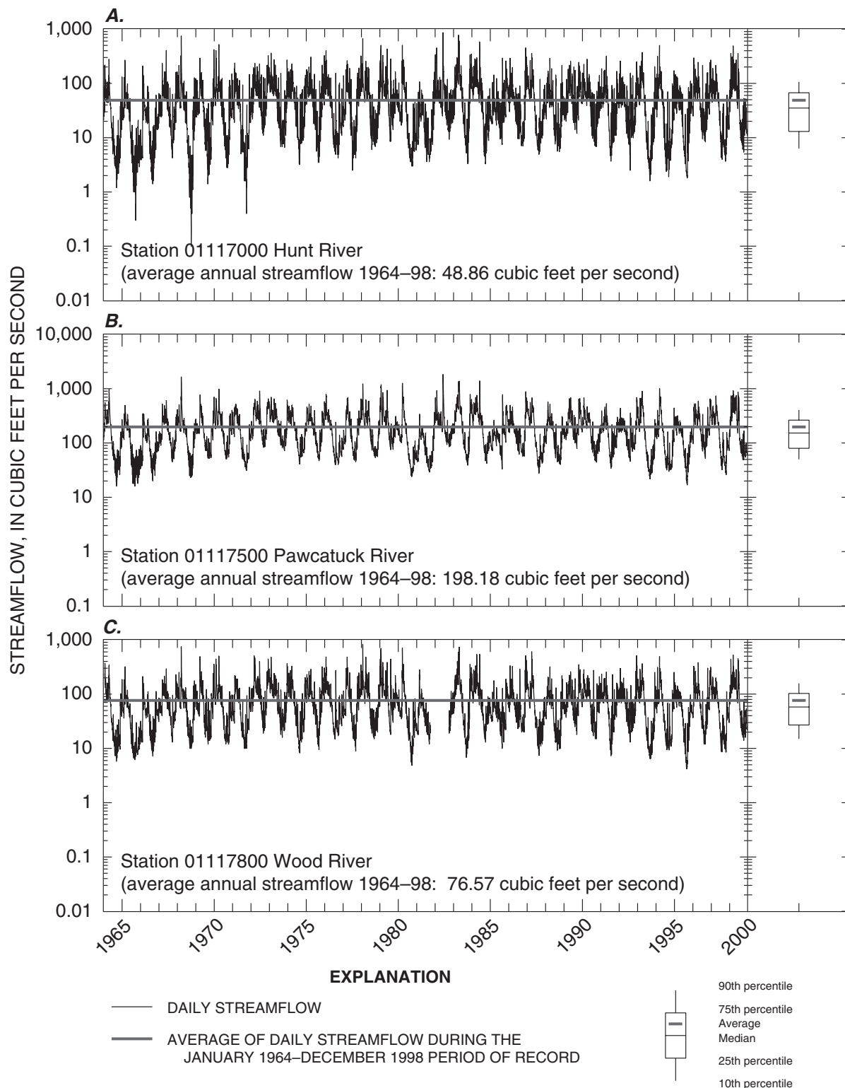
Figure 10. Record of daily streamflow and boxplot of streamflow statistics at gaging stations on the (A) Hunt River, (B) Pawcatuck River, (C) Wood River, (D) Nipmuc River, (E) Nooseneck River, and (F) Carr River, Rhode Island, 1964–98. (Gaging-station identification information listed in table 2. Locations of stations shown on fig. 2.)
