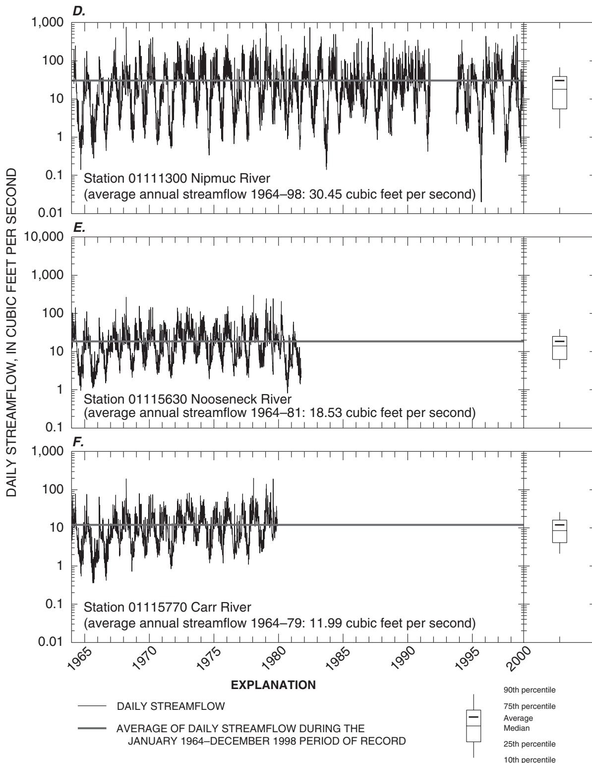
Figure 10—Continued. Record of daily streamflow and boxplot of streamflow statistics at gaging stations on the (A) Hunt River, (B) Pawcatuck River, (C) Wood River, (D) Nipmuc River, (E) Nooseneck River, and (F) Carr River, Rhode Island, 1964–98. (Gaging-station identification information listed in table 2. Locations of stations shown on fig. 2.)
