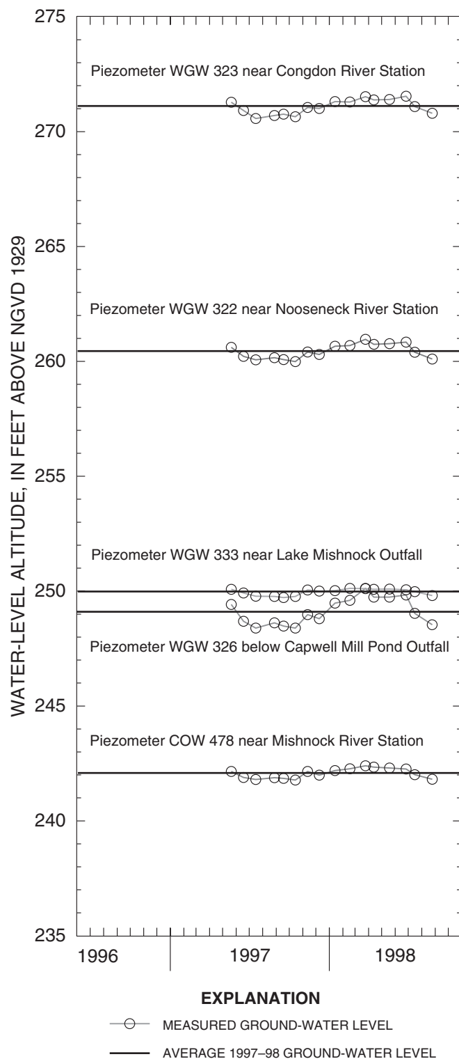
Figure 7. Water-level altitude measurements and the average of water-level altitudes measured in selected streambed piezometers in the Big River study area, Rhode Island, 1996–98. (Piezometer locations shown on fig. 4.)
