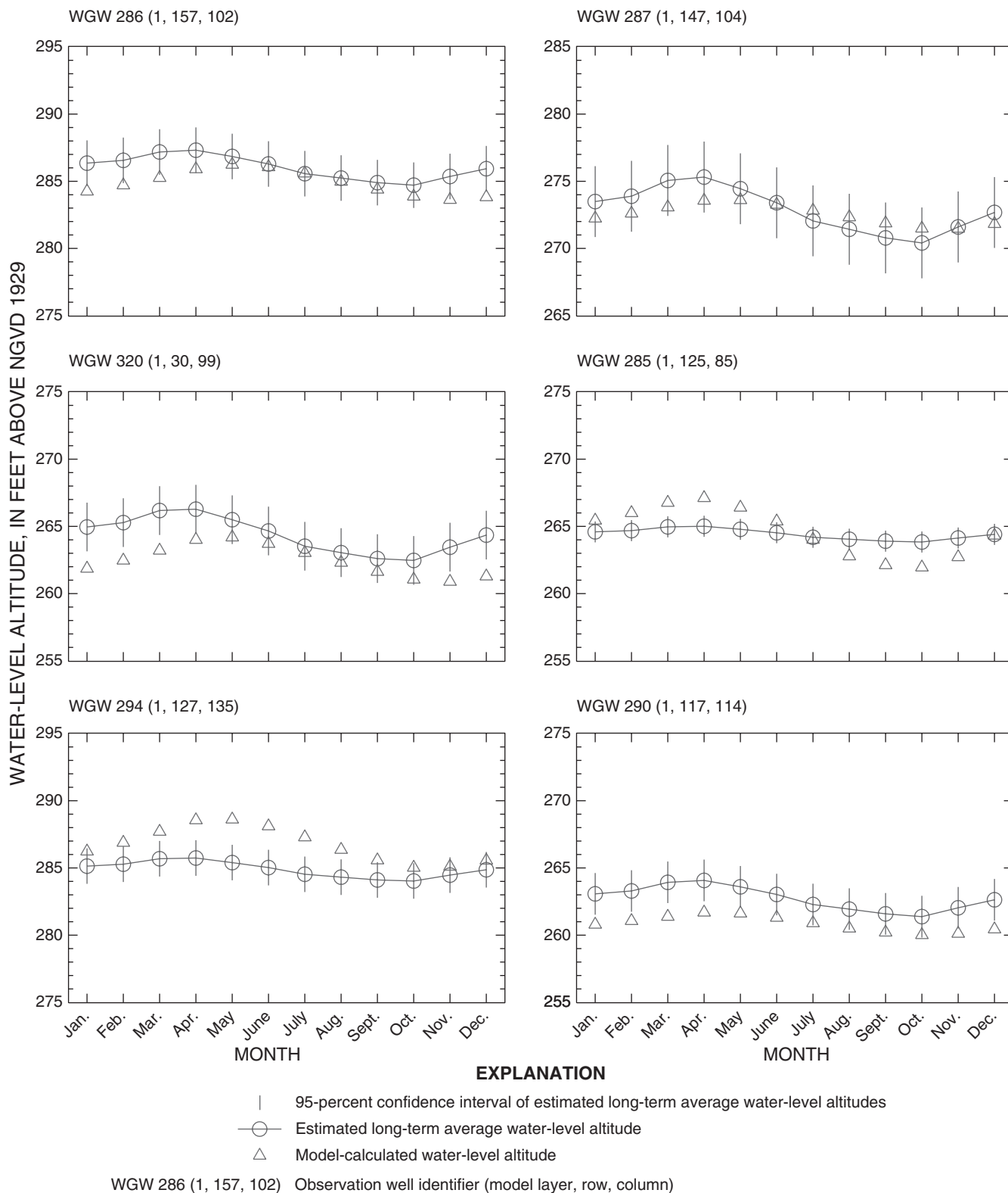
Figure 29. Estimated monthly average and model-calculated ground-water altitudes at 21 observation wells within the Big River study area, Rhode Island. (Locations of wells shown on fig. 4.)
