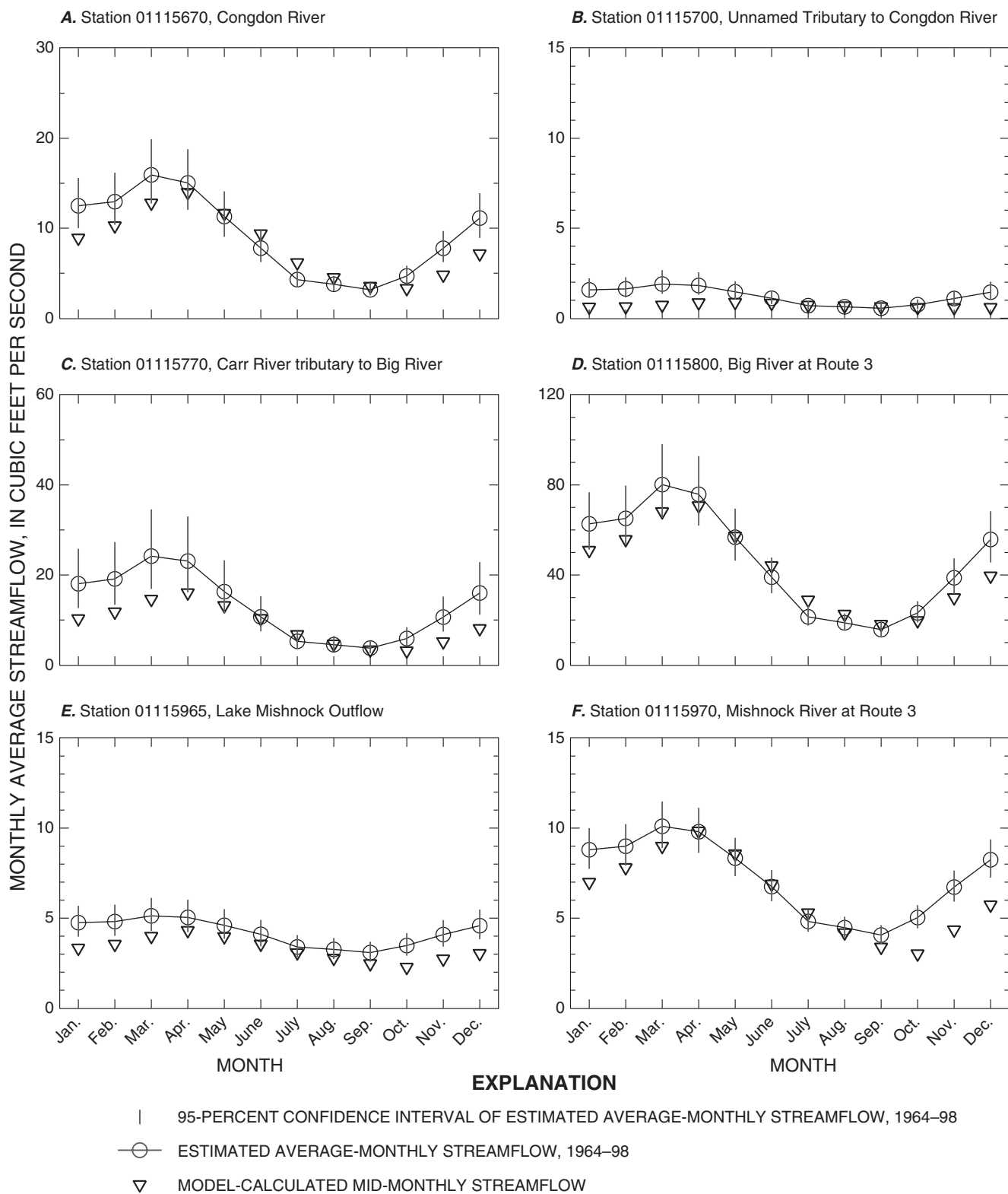
Figure 20. Estimated average monthly and model-calculated streamflows at six partial-record streamflow-gaging stations within the Big River study area, Rhode Island. (Locations of streamflow-gaging stations shown on fig. 4.)
