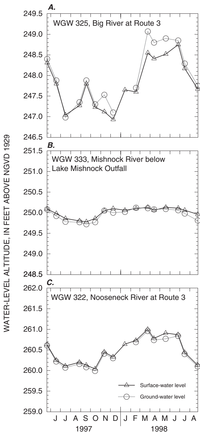
Figure 9. Paired surface-water-level altitudes and ground-water-level altitudes measured at selected streambed piezometers on the (A) Big River, (B) Mishnock River, and (C) Nooseneck River, Rhode Island, 1997–98. (Piezometer locations shown on fig. 4.)
