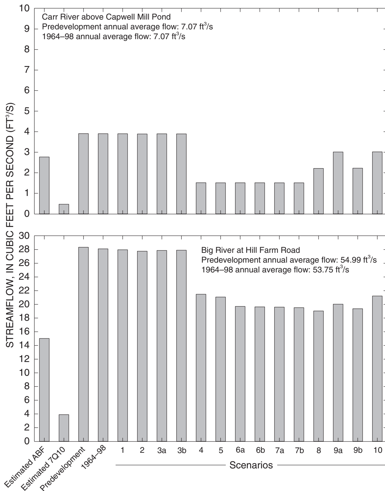
Figure 26—Continued. Model-calculated monthly average August streamflow at the Lake Mishnock outfall, the Mishnock River at Route 3, the Carr River above Capwell Mill Pond, and the Big River at Hill Farm Road for the predevelopment conditions, conditions during 1964–98, and 14 withdrawal scenarios, Big River study area, Rhode Island. (Location of streamflow sites shown on fig. 23; withdrawal scenarios described in table 10.)
