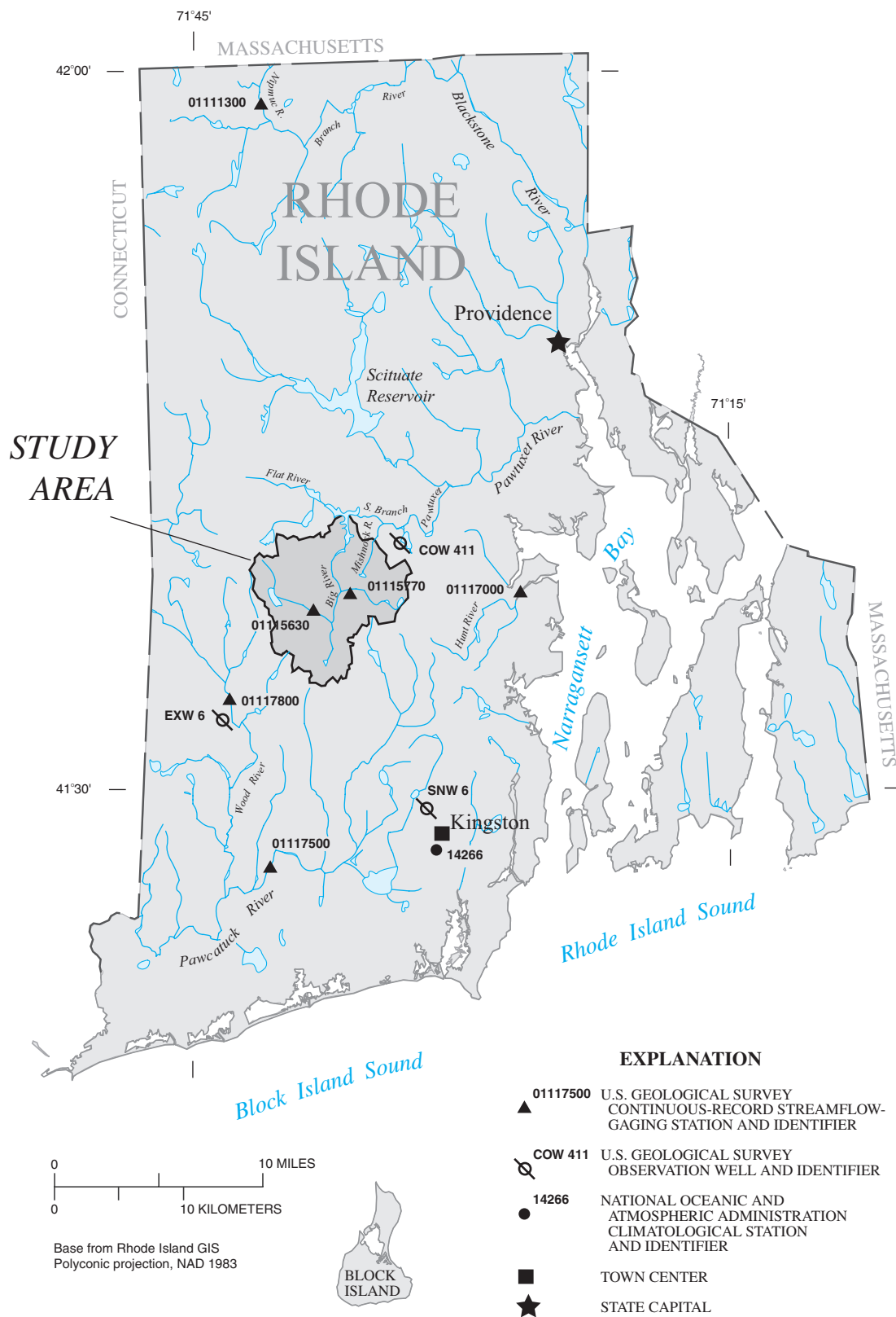
Figure 2. Location of U.S. Geological Survey continuous streamflow-gaging stations, observation wells, and National Oceanic and Atmospheric Administration climatological station used to estimate hydrologic conditions in the Big River study area, Rhode Island, 1964–98.
