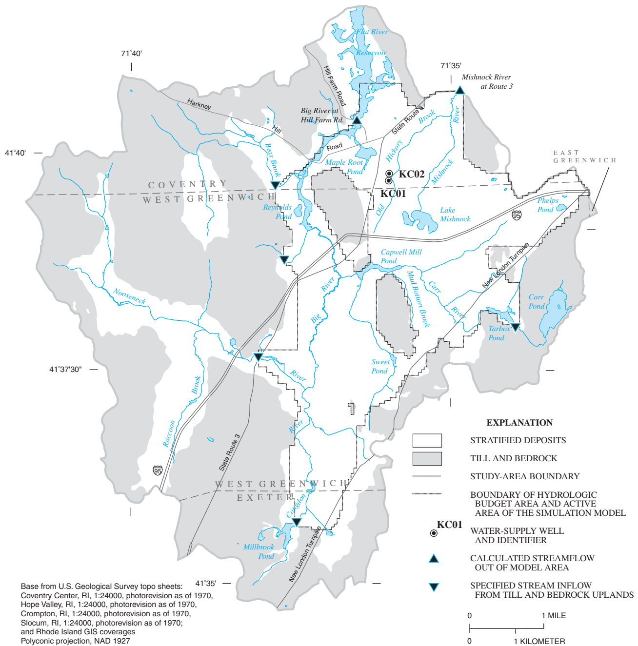
Figure 13. Spatial extent of the hydrologic-budget area, active area of simulation model, specified stream-inflow locations, and location of model-calculated streamflows out of the Big River study area, Rhode Island.
