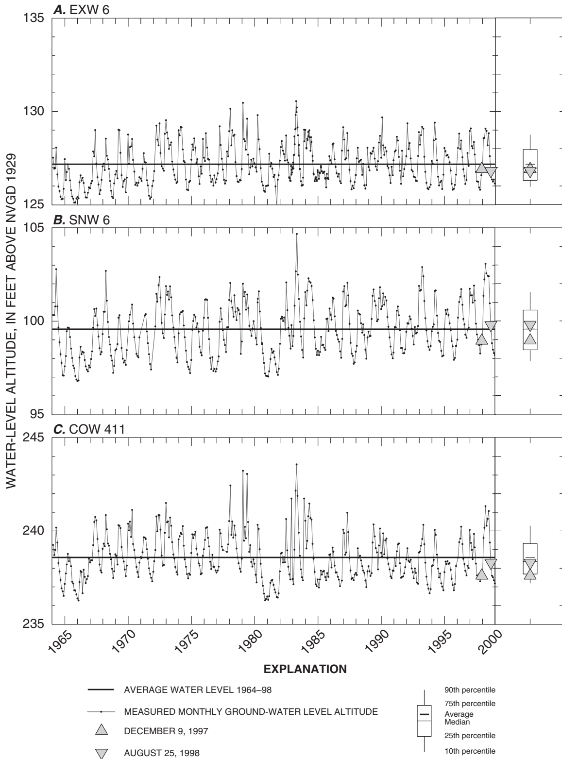
Figure 6. Record of monthly water-level altitudes and distribution of water-level altitudes recorded at wells (A) EXW 6, (B) SNW 6, and (C) COW 411, Big River study area, Rhode Island, 1964–98. (Locations of wells shown on fig. 2.)
