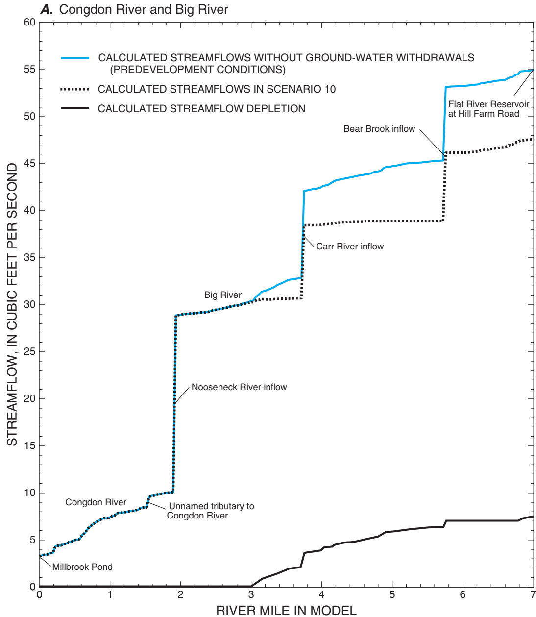
Figure 28. Model-calculated steady-state streamflows and streamflow depletions for scenario 10 in the (A) Congdon and Big Rivers, (B) Carr River, (C) western unnamed tributary to the Carr River, (D) Mishnock River, and (E) Old Hickory Brook, Rhode Island. (Streamflows calculated for model cells along the centerline of on-stream ponds were used.)
