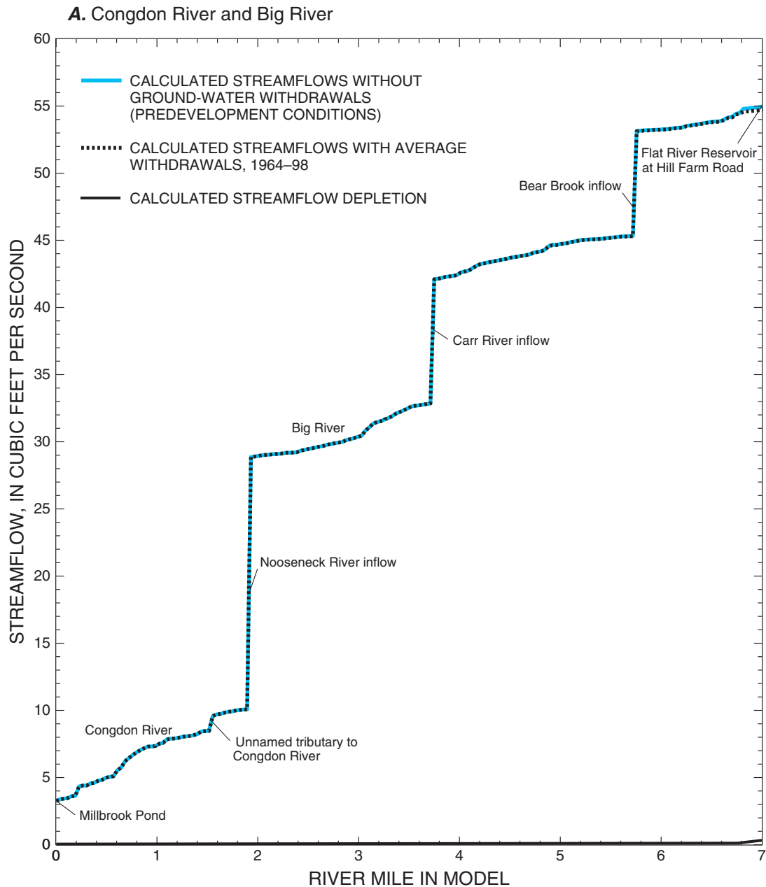
Figure 21. Model-calculated steady-state streamflows and streamflow depletions for the 1964–98 period in the (A) Congdon and Big Rivers, (B) Carr River, (C) western unnamed tributary to the Carr River, (D) Mishnock River, and (E) Old Hickory Brook, Rhode Island. (For on-stream ponds, streamflows were calculated for model cells along the centerline of the ponds.)
