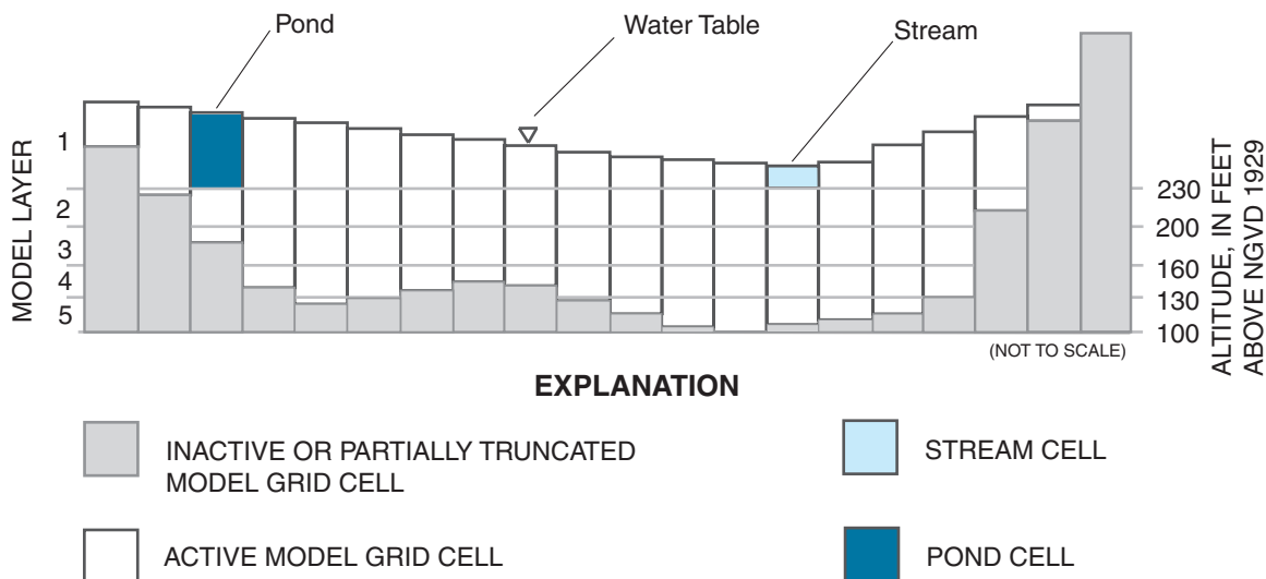
Figure 17. Schematic section showing active model cells and model layers for the simulation model of the Big River study area, Rhode Island.
