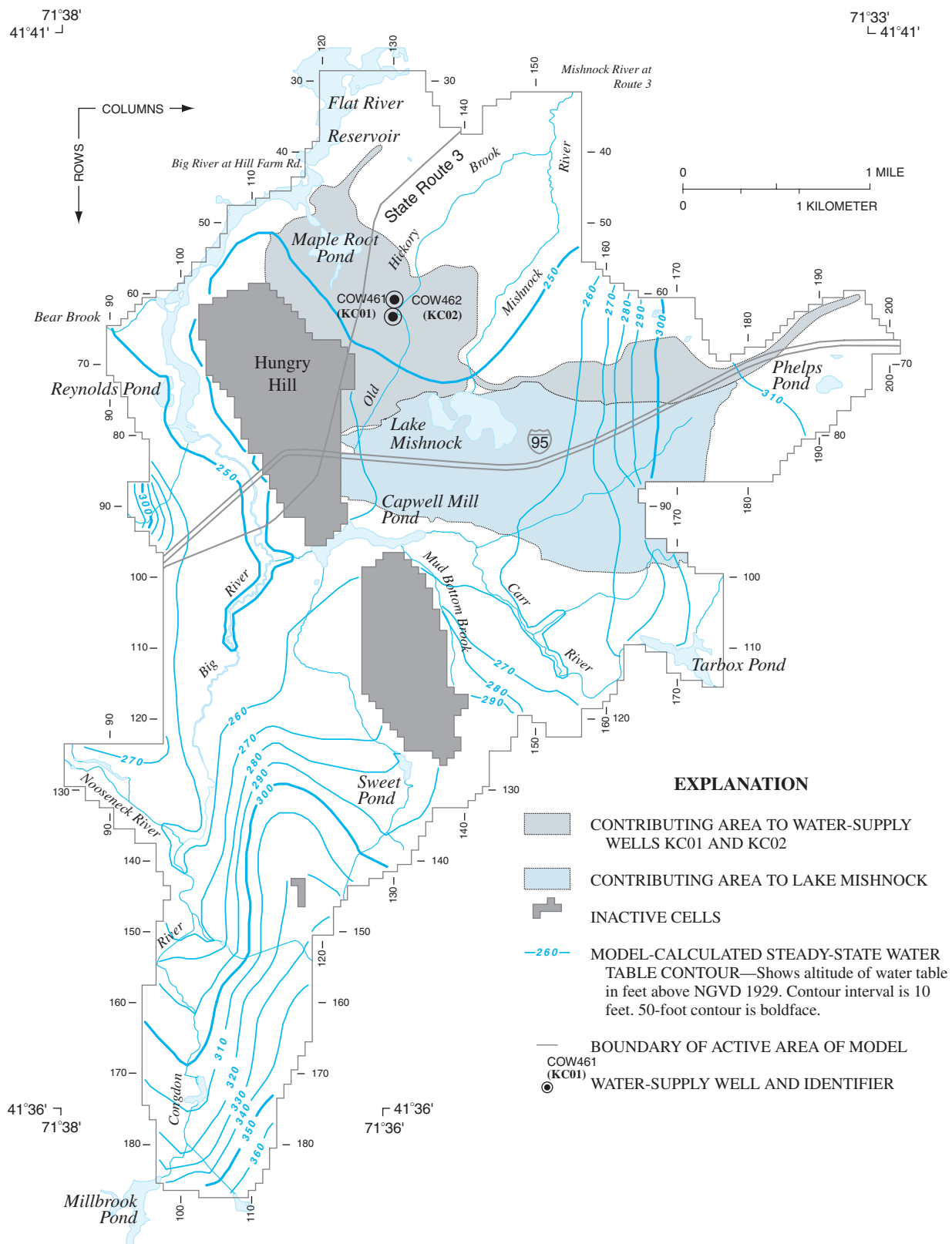
Figure 22. Model-calculated steady-state contributing areas for Lake Mishnock, Rhode Island, and for public-water-supply wells KC01 and KC02 for simulated conditions during 1964–98.
