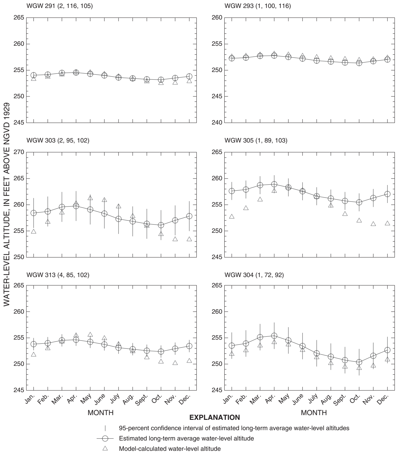
Figure 29 —Continued. Estimated monthly average and model-calculated ground-water altitudes at 21 observation wells within the Big River study area, Rhode Island. (Locations of wells shown on fig. 4.)
