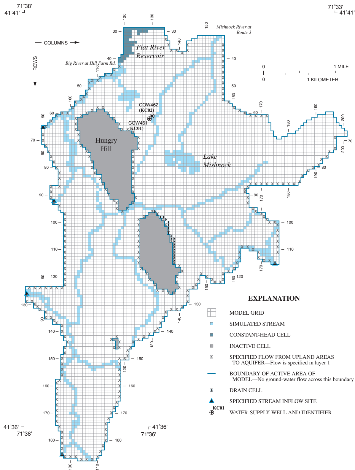
Figure 16. Grid and boundary conditions of the active model cells for the simulation model of the Big River study area, Rhode Island.
