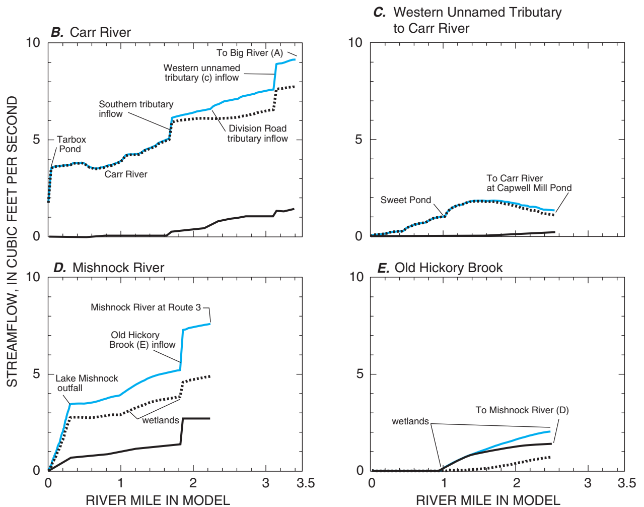
Figure 28—Continued. Model-calculated steady-state streamflows and streamflow depletions for scenario 10 in the (A) Congdon and Big Rivers, (B) Carr River, (C) western unnamed tributary to the Carr River, (D) Mishnock River, and (E) Old Hickory Brook, Rhode Island. (Streamflows calculated for model cells along the centerline of on-stream ponds were used.)
