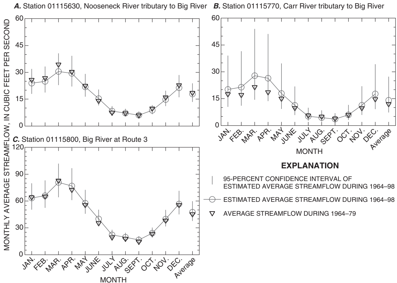
Figure 11. Estimated long-term average monthly streamflow at the Nooseneck River, Carr River, and Big River partial-record gaging stations compared to average monthly flows for the 1964–79 period of record for the Nooseneck River and Carr River gaging stations and an area-weighted estimate for the Big River from continuous-gage records at the Nooseneck River and Carr River tributaries, Rhode Island. (Gaging station identification information listed in tables 2 and 3. Locations of gages shown on figs. 2 and 4.)
