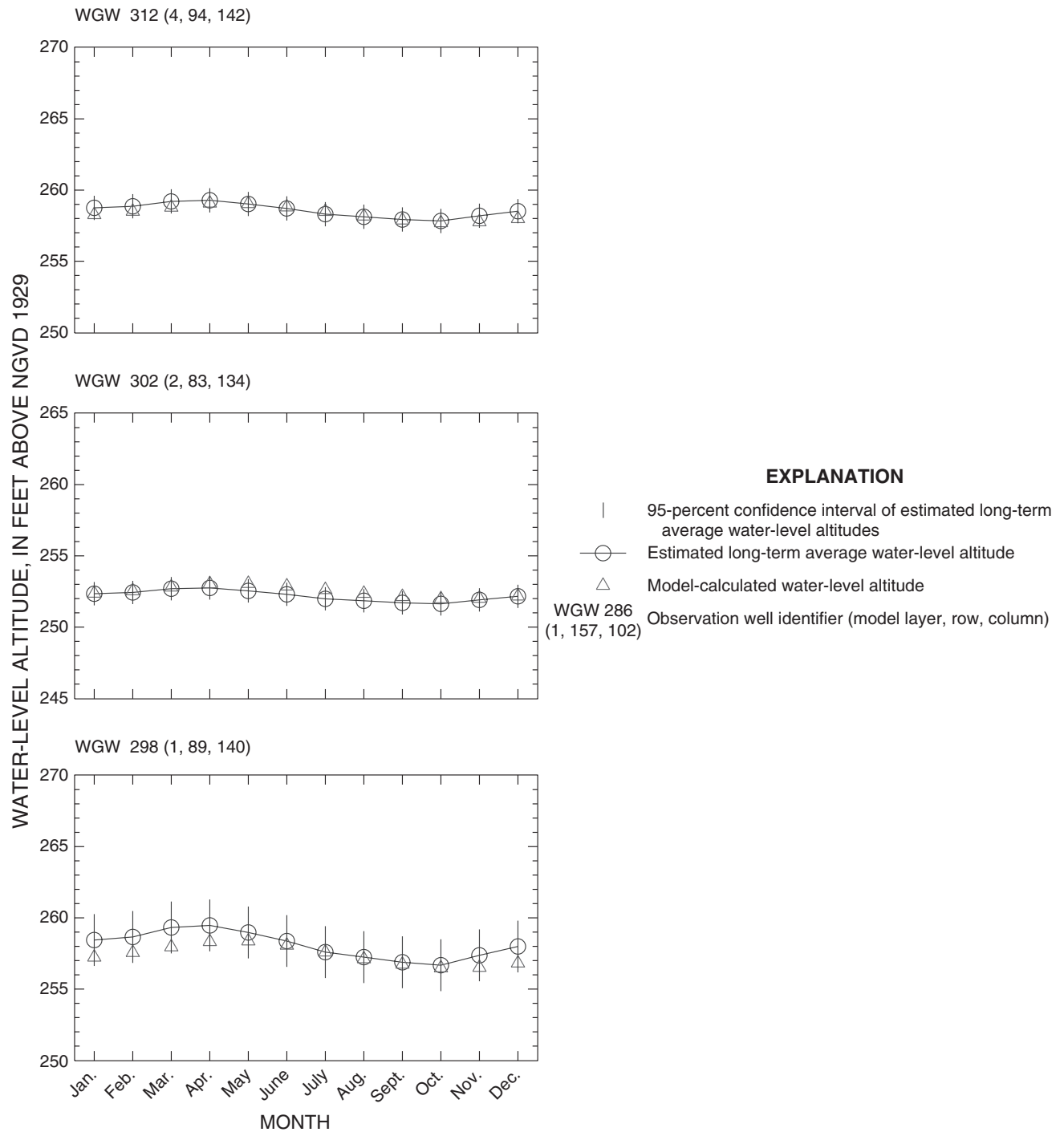
Figure 29—Continued Estimated monthly average and model-calculated ground-water altitudes at 21 observation wells within the Big River study area, Rhode Island. (Locations of wells shown on fig. 4.)
