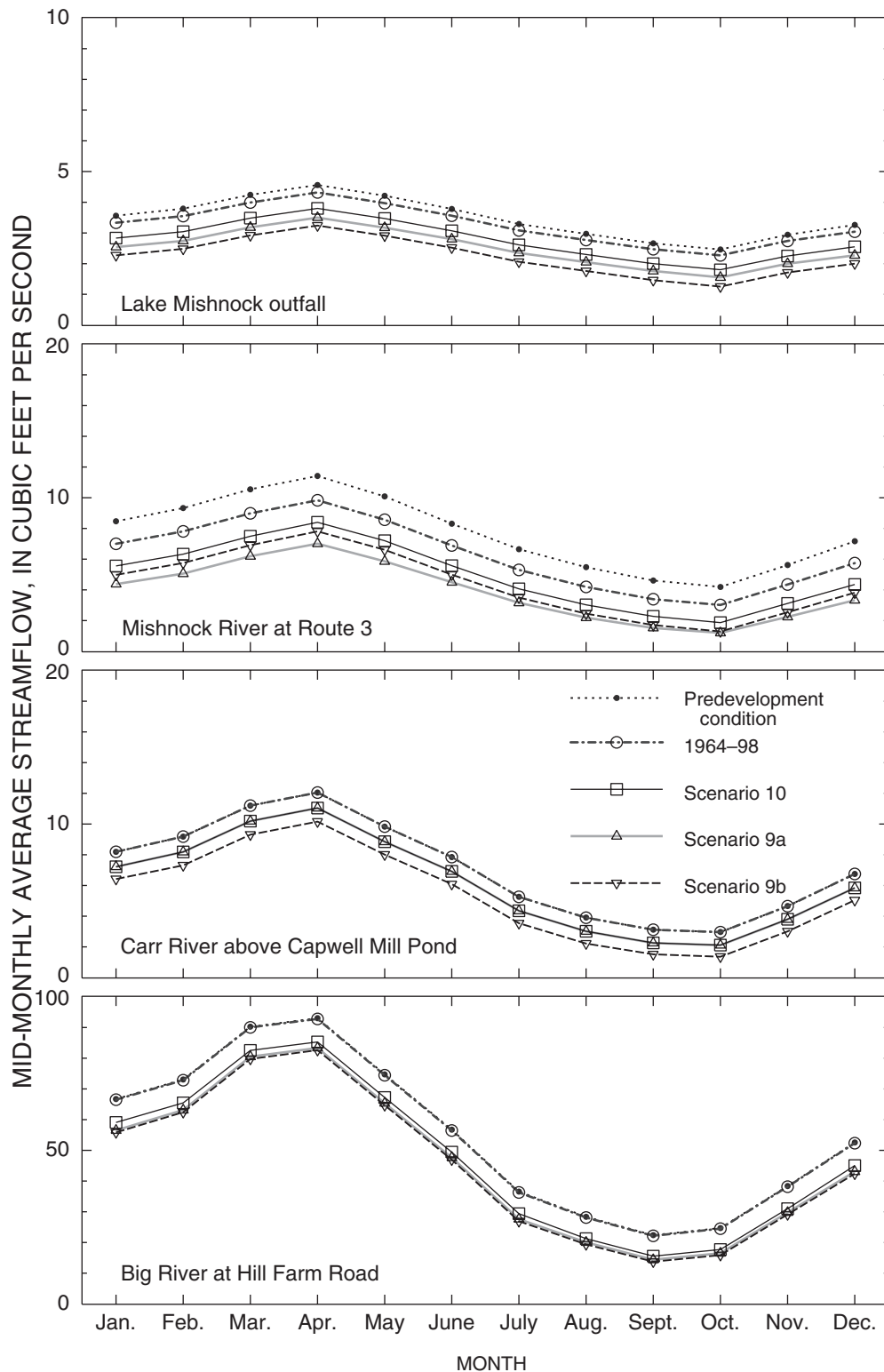
Figure 30—Continued. Model-calculated monthly average streamflow at the Lake Mishnock outfall, the Mishnock River at Route 3, the Carr River above Capwell Mill Pond, and the Big River at Hill Farm Road for the predevelopment conditions, conditions during 1964–98, and 14 withdrawal scenarios, Big River study area, Rhode Island. (Location of streamflow index sites shown on fig. 23; withdrawal scenarios described in table 10.)
