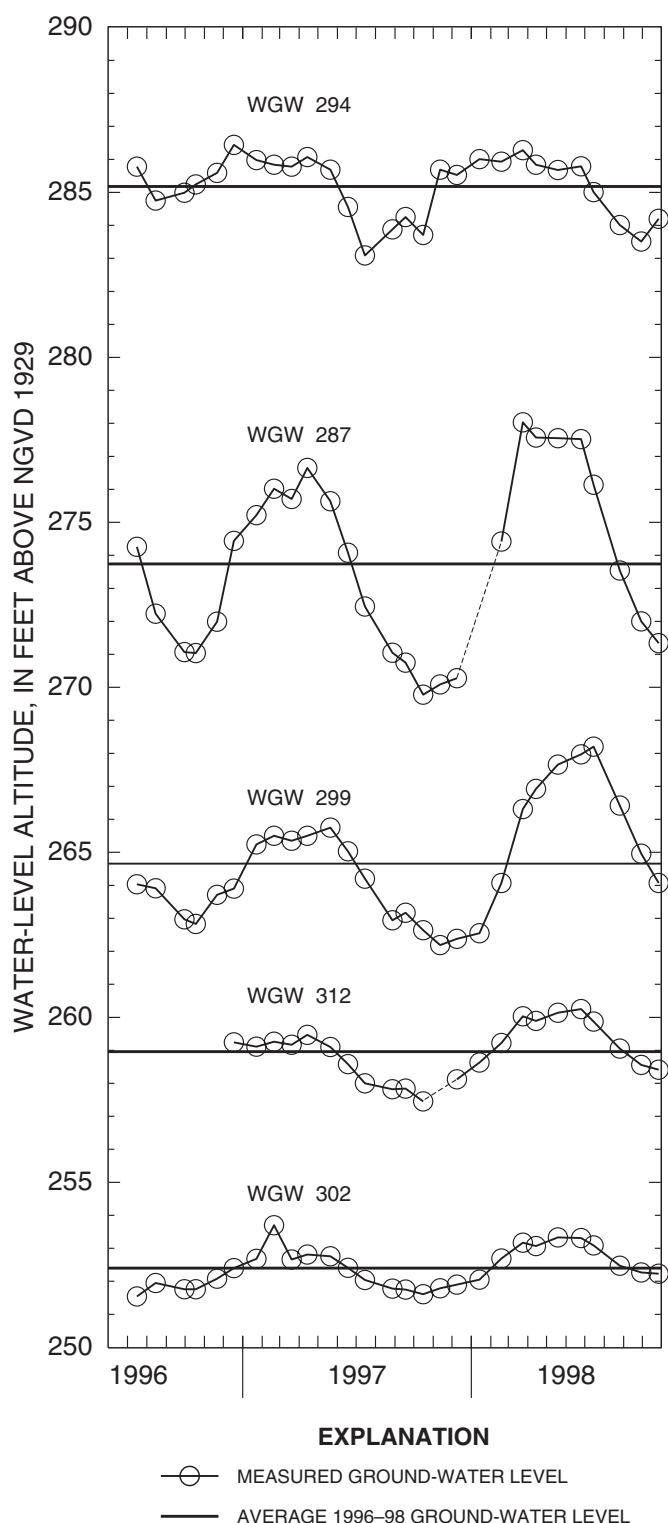
Figure 5. Water-level altitude measurements and the average of water-level altitudes measured in selected wells in the Big River study area, Rhode Island, 1996–98. (Well locations shown on fig. 4.)
