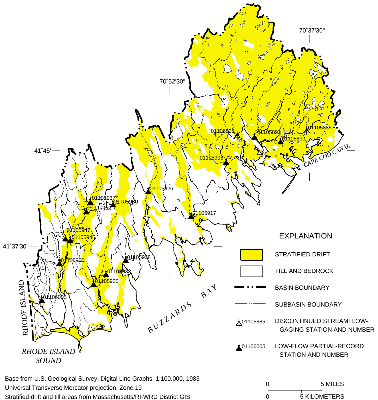
Figure 6. Location of low-flow partial-record stations and discontinued streamflow-gaging stations in Buzzards Bay Basin, southeastern Massachusetts.
