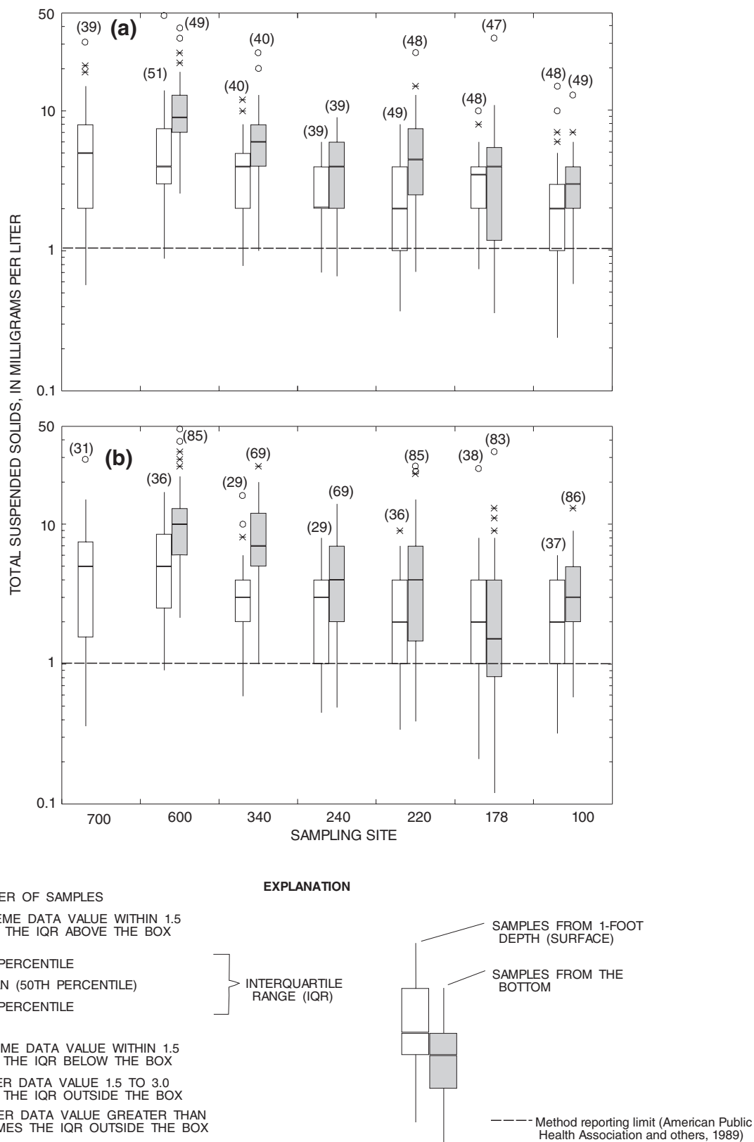
Figure 9. Range and distribution of total suspended solids at selected sites in Lake Travis, near Austin, Texas, during (a) thermally stratified period and (b) mixed period.
