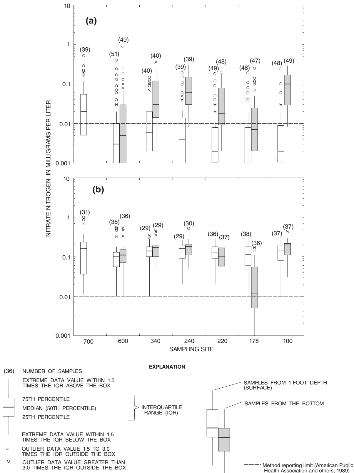
Figure 10. Range and distribution of nitrate nitrogen at selected sites in Lake Travis, near Austin, Texas, during (a) thermally stratified period and (b) mixed period.
