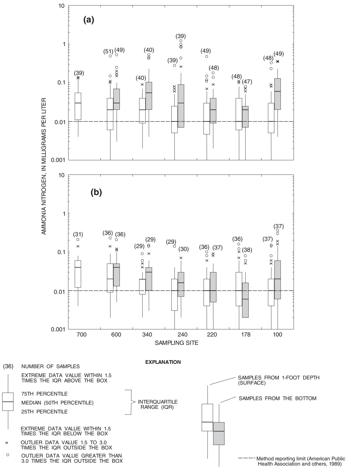
Figure 11. Range and distribution of ammonia nitrogen at selected sites in Lake Travis, near Austin, Texas, during (a) thermally stratified period and (b) mixed period.
