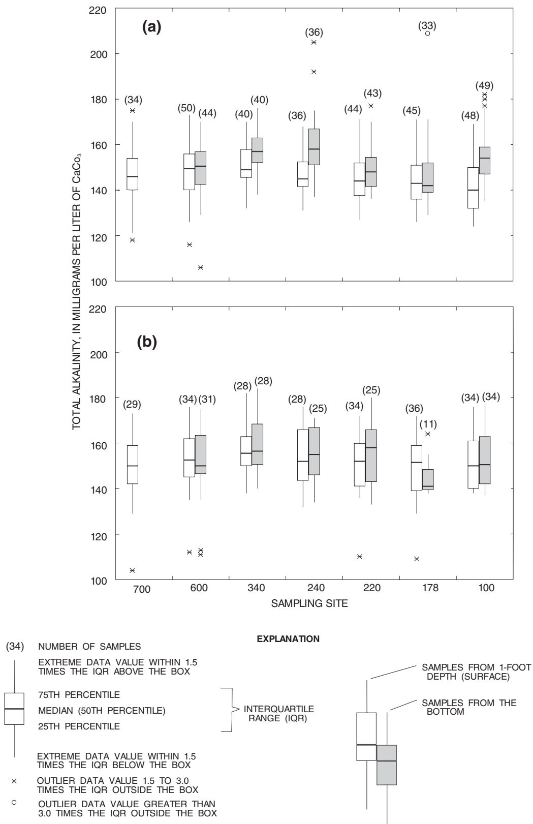
Figure 8. Range and distribution of total alkalinity as \text{CaCO}_3 at selected sites in Lake Travis, near Austin, Texas, during (a) thermally stratified period and (b) mixed period.
