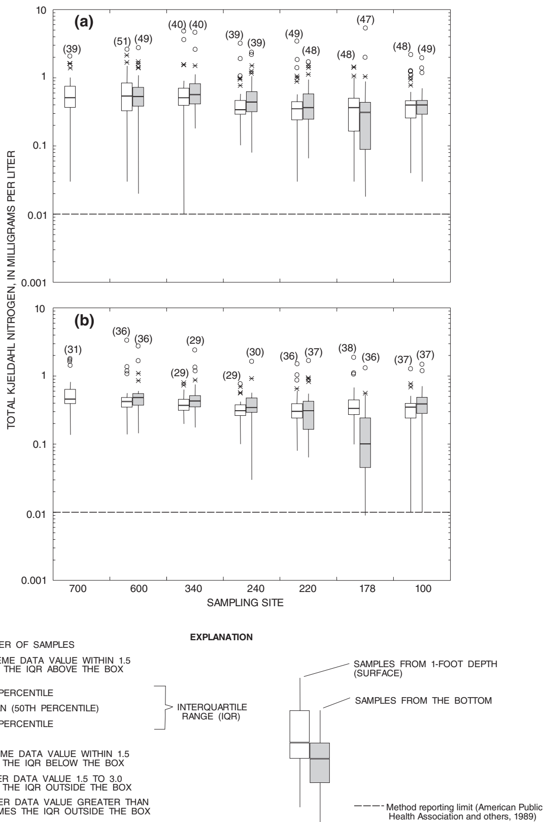
Figure 12. Range and distribution of total Kjeldahl nitrogen at selected sites in Lake Travis, near Austin, Texas, during (a) thermally stratified period and (b) mixed period.
