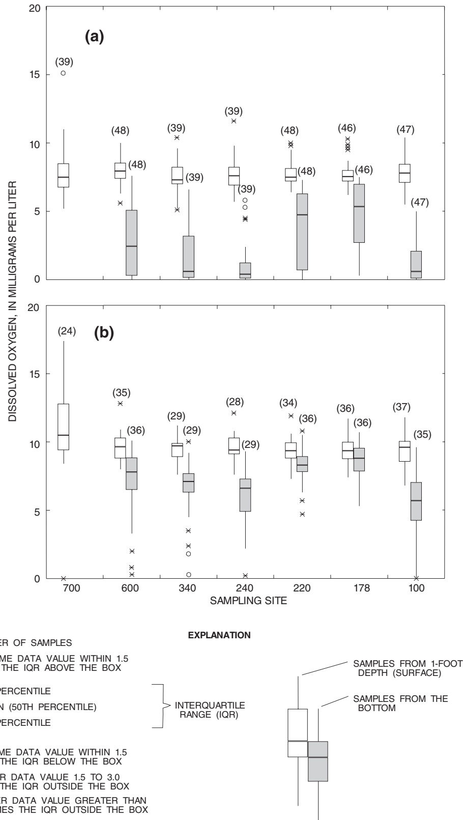
Figure 6. Range and distribution of dissolved oxygen at selected sites in Lake Travis, near Austin, Texas, during (a) thermally stratified period and (b) mixed period.
