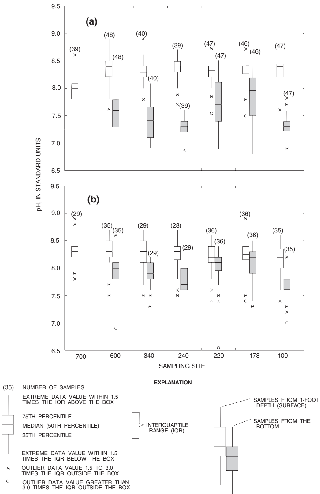
Figure 4. Range and distribution of pH at selected sites in Lake Travis, near Austin, Texas, during (a) thermally stratified period and (b) mixed period.
