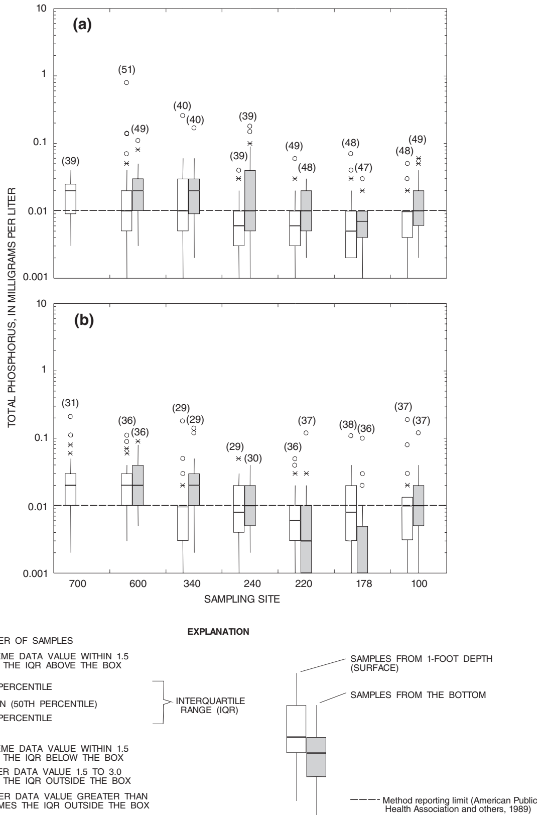
Figure 13. Range and distribution of total phosphorus at selected sites in Lake Travis, near Austin, Texas, during (a) thermally stratified period and (b) mixed period.
