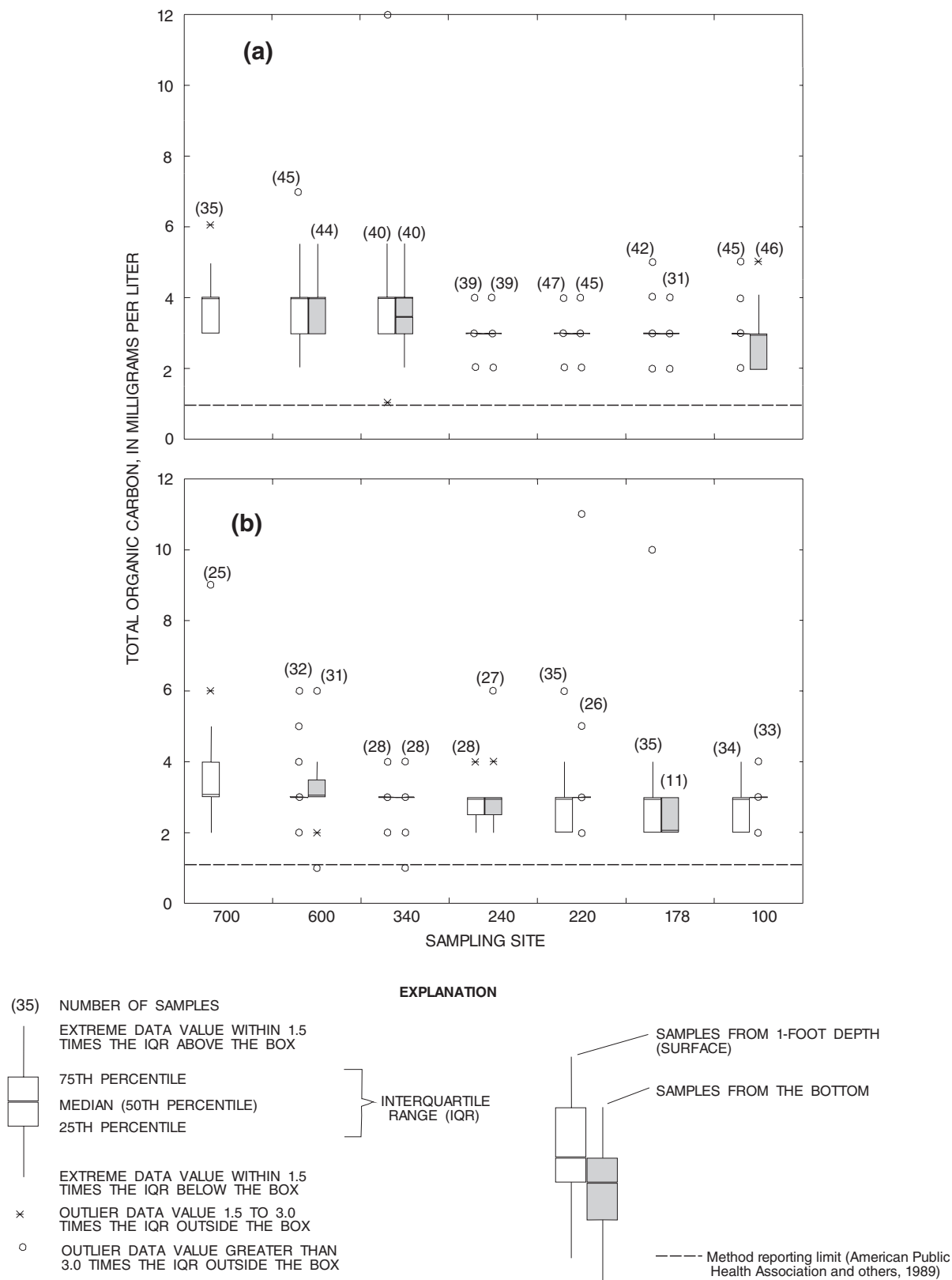
Figure 14. Range and distribution of total organic carbon at selected sites in Lake Travis, near Austin, Texas, during (a) thermally stratified period and (b) mixed period.
