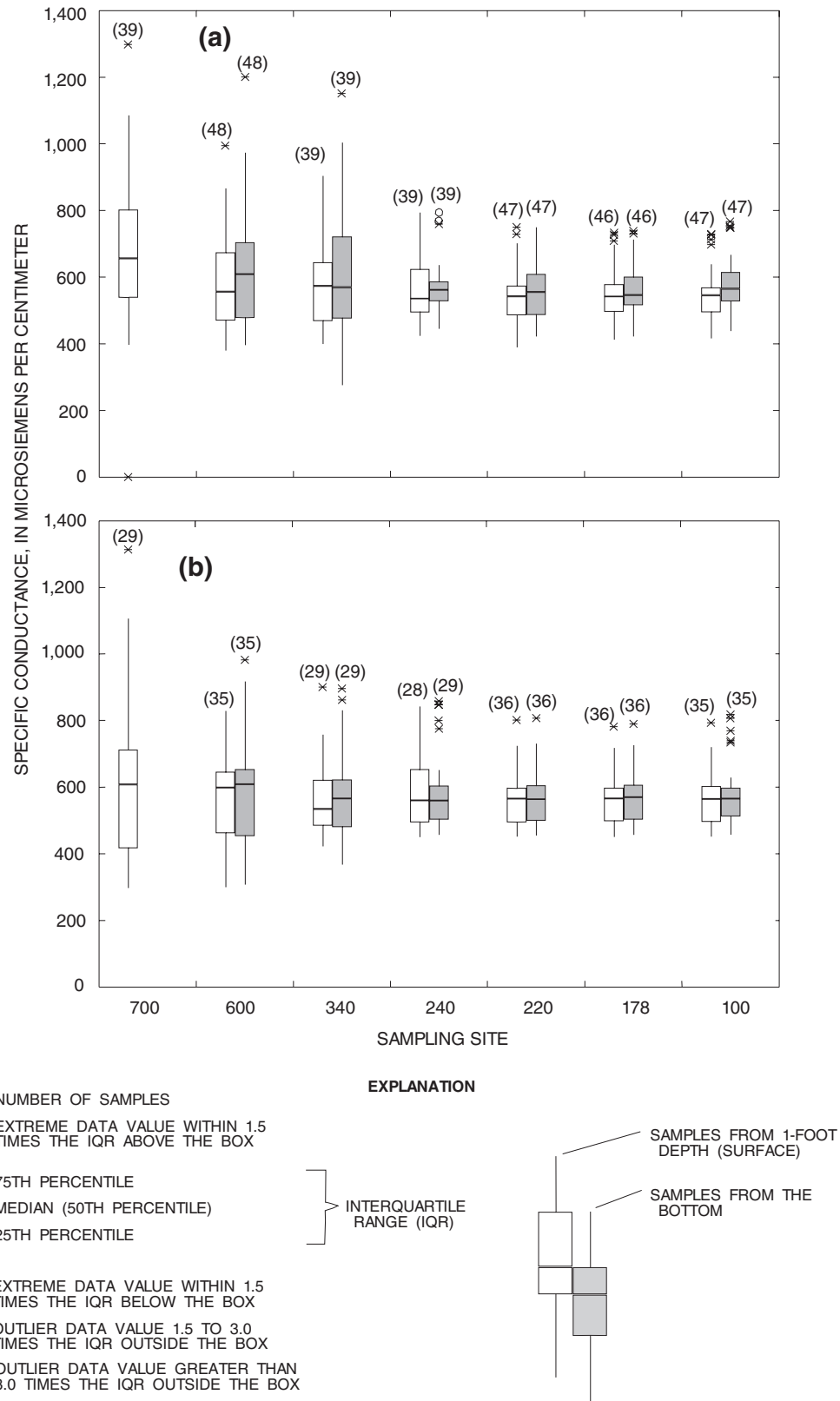
Figure 3. Range and distribution of specific conductance at selected sites in Lake Travis, near Austin, Texas, during (a) thermally stratified period and (b) mixed period.
