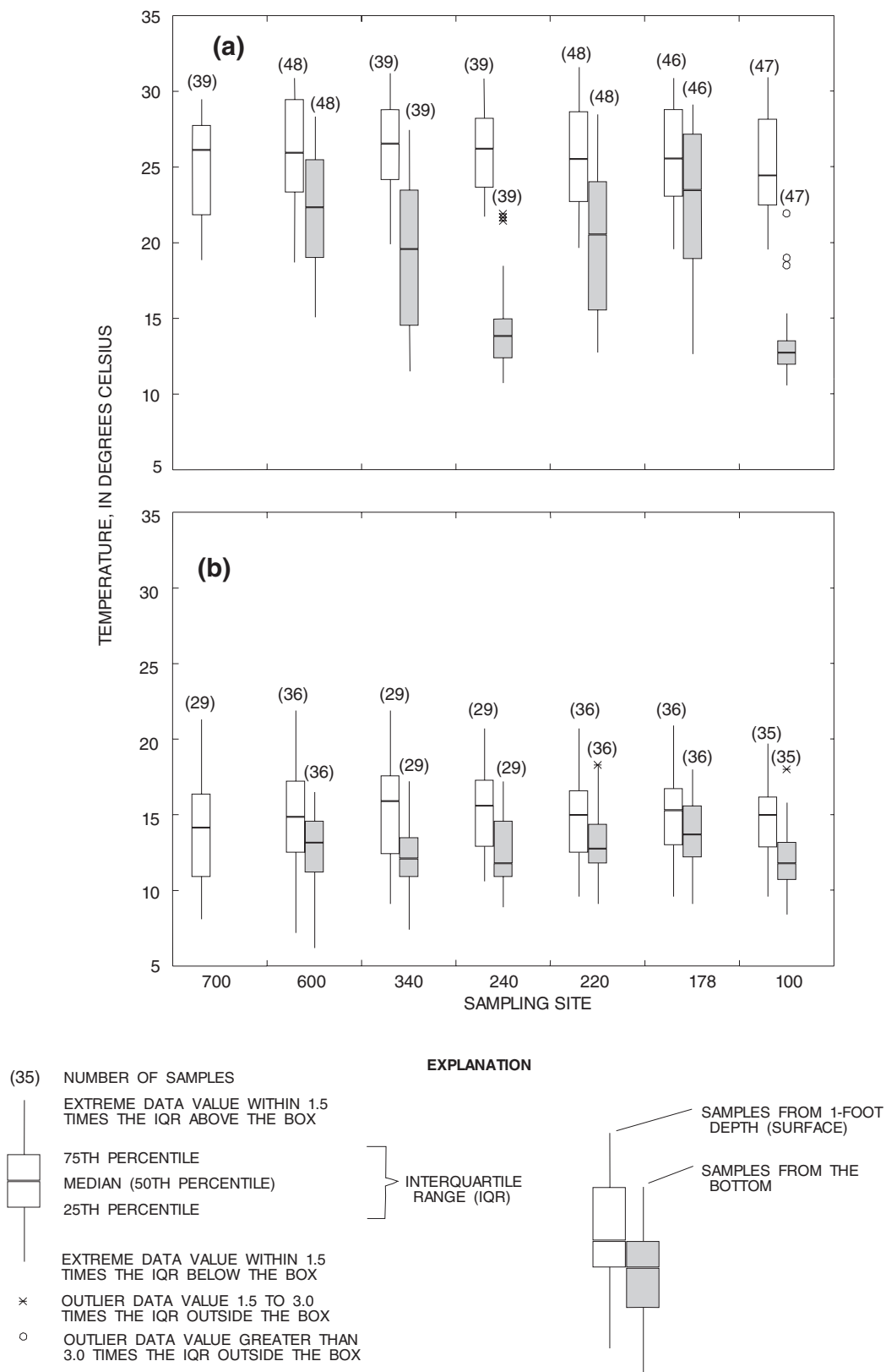
Figure 5. Range and distribution of temperature at selected sites in Lake Travis, near Austin, Texas, during (a) thermally stratified period and (b) mixed period.
