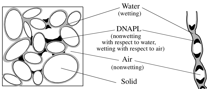
c. In partly saturated porous media
