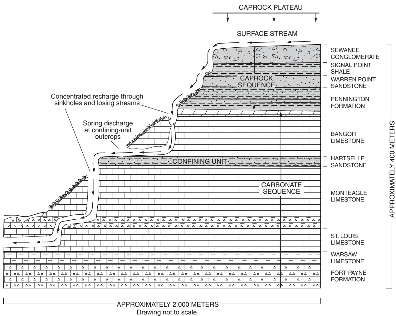
Figure 9. Generalized hydrogeologic section through the Cumberland Plateau escarpments in Tennessee. (Modified from Crawford, 1987.)
