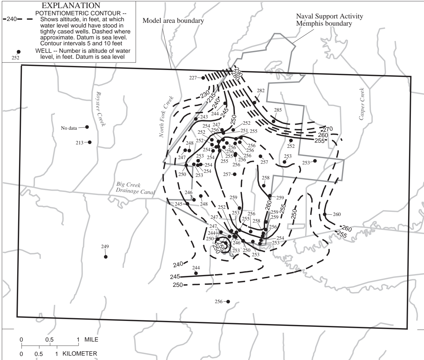
Figure 10. Altitude of the potentiometric surface of the alluvial-fluvial deposits aquifer at Naval Support Activity Memphis, Millington, Tennessee, October 1996.
