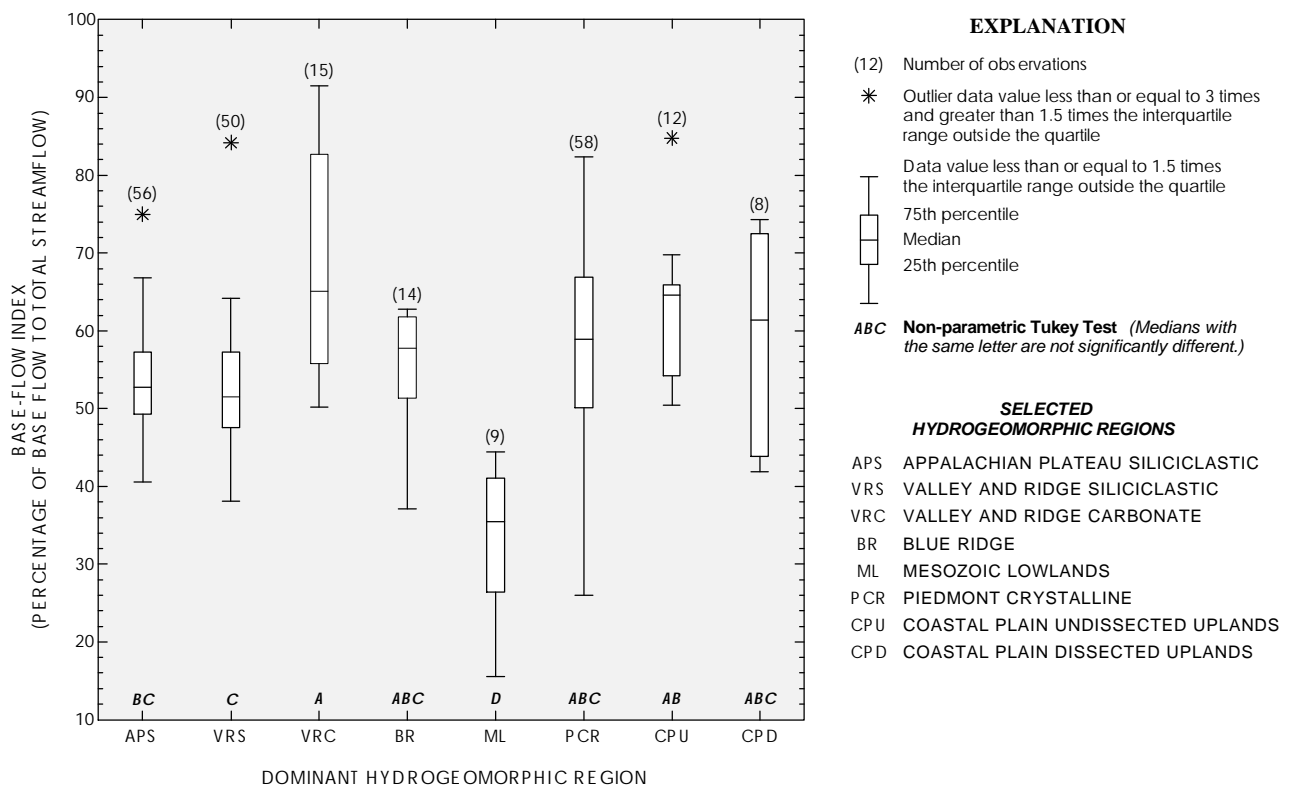
Figure 6. Distribution of base-flow index among hydrogeomorphic regions (HGMR's).
