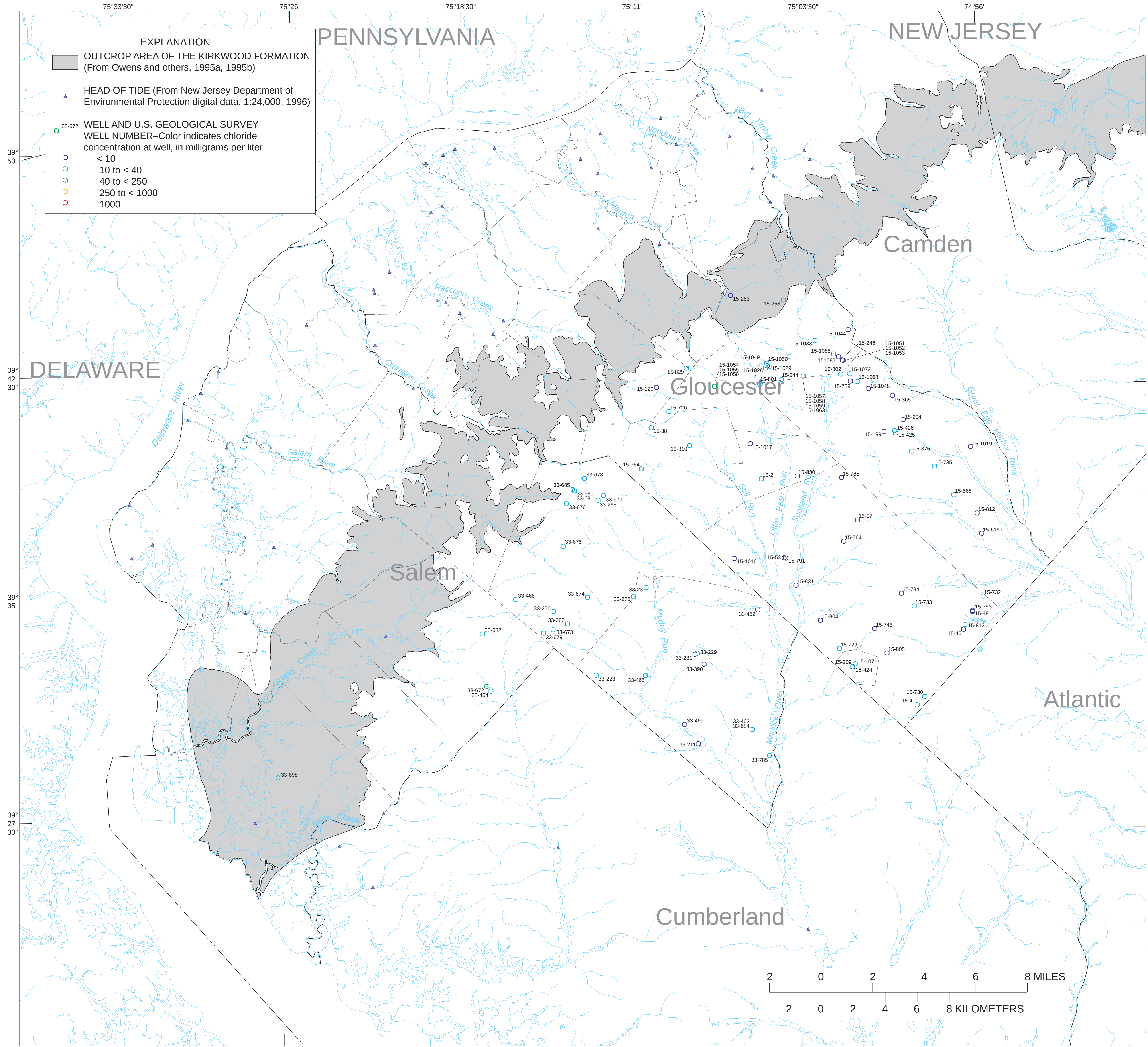
MAXIMUM CHLORIDE CONCENTRATION IN SAMPLES FROM WELLS SCREENED IN THE KIRKWOOD-COHANSEY AQUIFER SYSTEM, GLOUCESTER AND SALEM COUNTIES, NEW JERSEY
