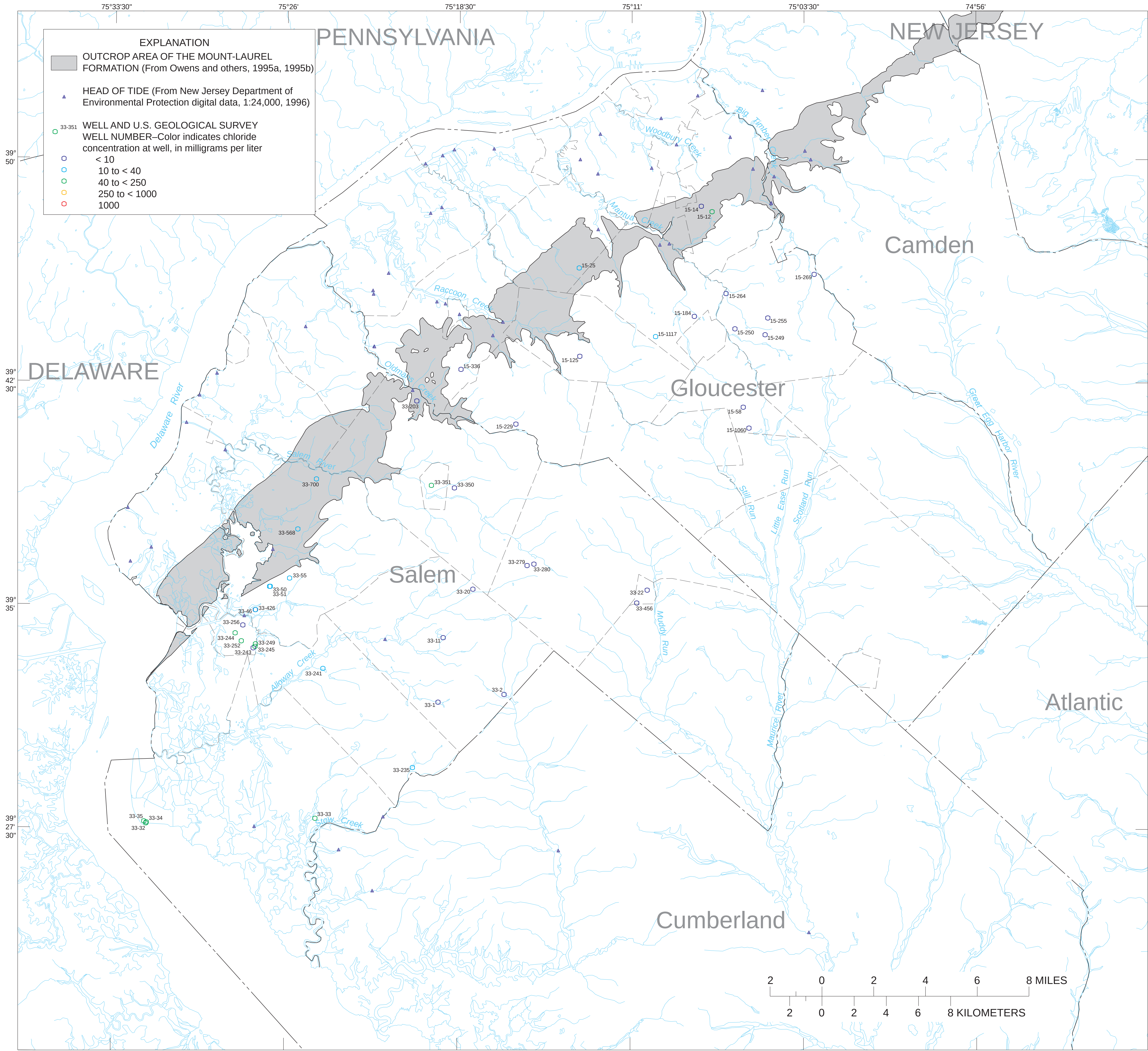
MAXIMUM CHLORIDE CONCENTRATION IN SAMPLES FROM WELLS SCREENED IN THE WENONAH-MOUNT LAUREL AQUIFER, GLOUCESTER AND SALEM COUNTIES, NEW JERSEY
