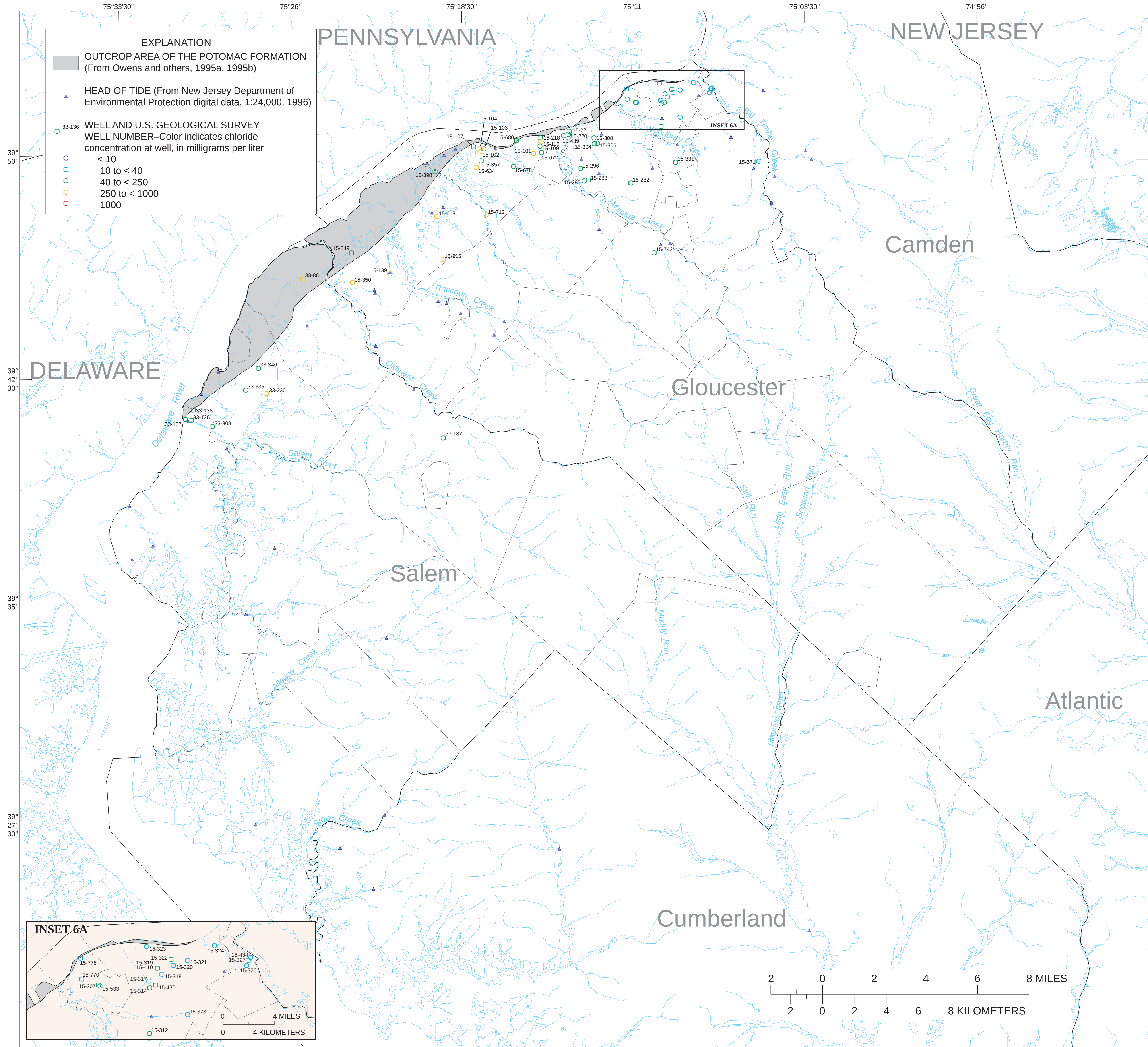
MAXIMUM CHLORIDE CONCENTRATION IN SAMPLES FROM WELLS SCREENED IN THE LOWER POTOMAC-RARITAN-MAGOTHY AQUIFER, GLOUCESTER AND SALEM COUNTIES, NEW JERSEY
