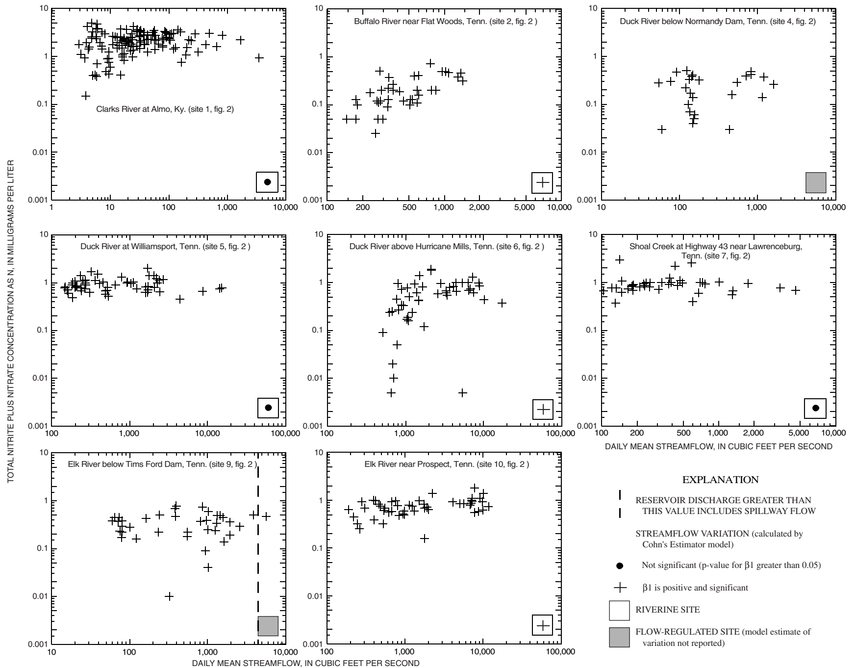
Appendix D1. Variation in total nitrite plus nitrate concentrations with streamflow and model estimate of streamflow variation in concentration at selected sites in the lower Tennessee River Basin, 1980-96.
