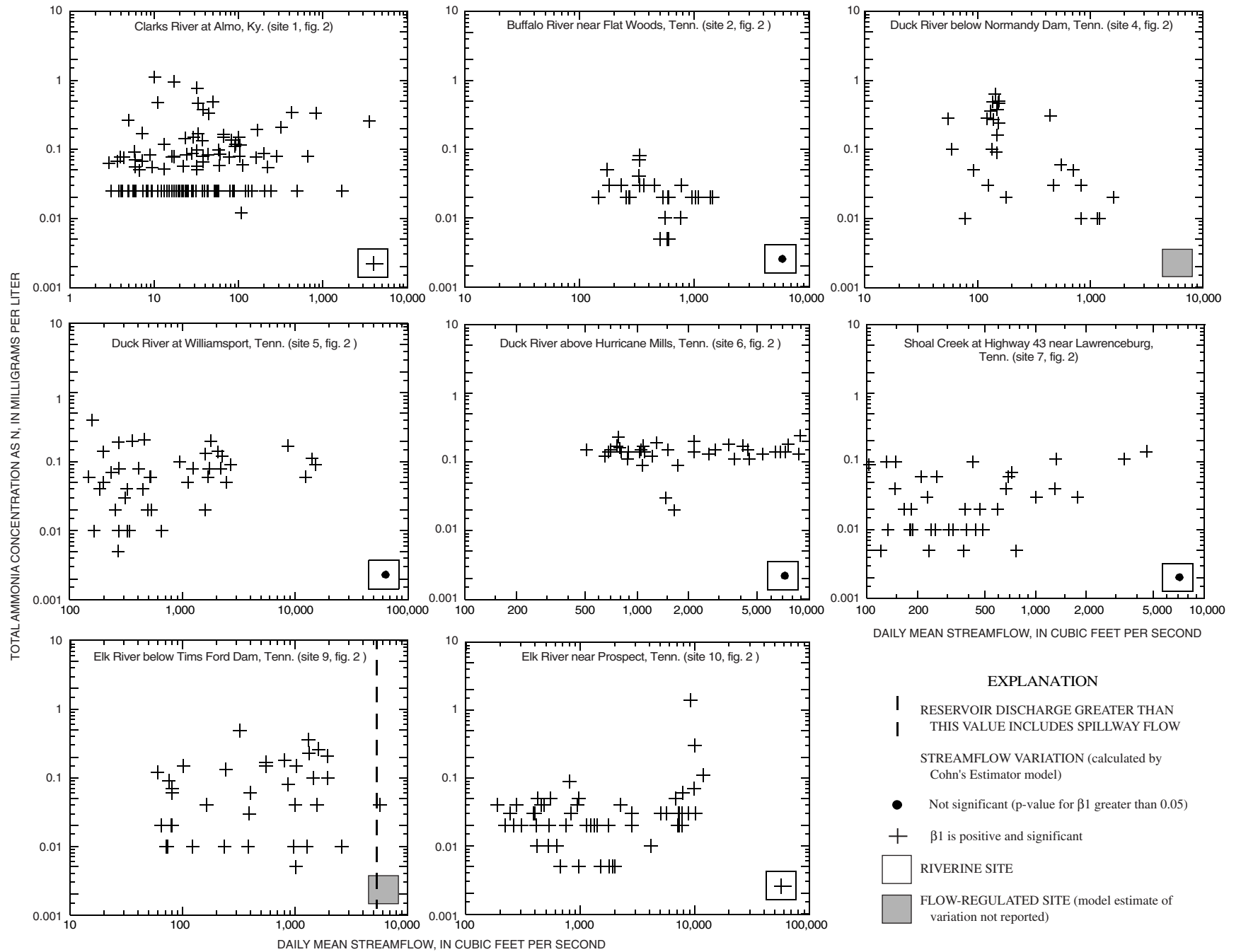
Appendix D2. Variation in total ammonia concentrations with streamflow and model estimate of streamflow variation in concentration at selected sites in the lower Tennessee River Basin, 1980-96.
