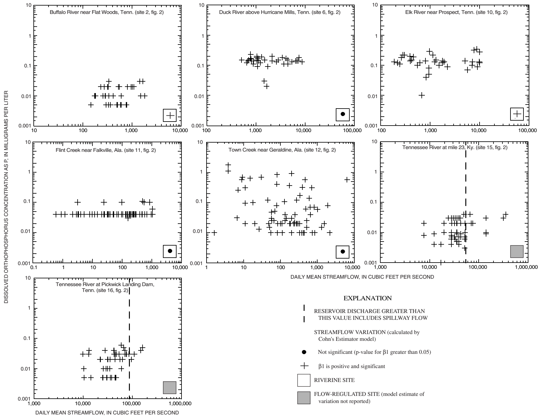
Appendix D4. Variation in dissolved orthophosphorus concentrations with streamflow and model estimate of streamflow variation in concentration at selected sites in the lower Tennessee River Basin, 1980-96.
