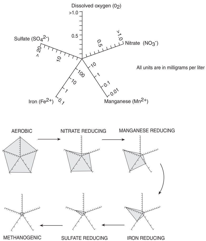
Figure 10. Radial diagrams used to illustrate electron acceptor processes. (Modified from Carey, 1998.)
