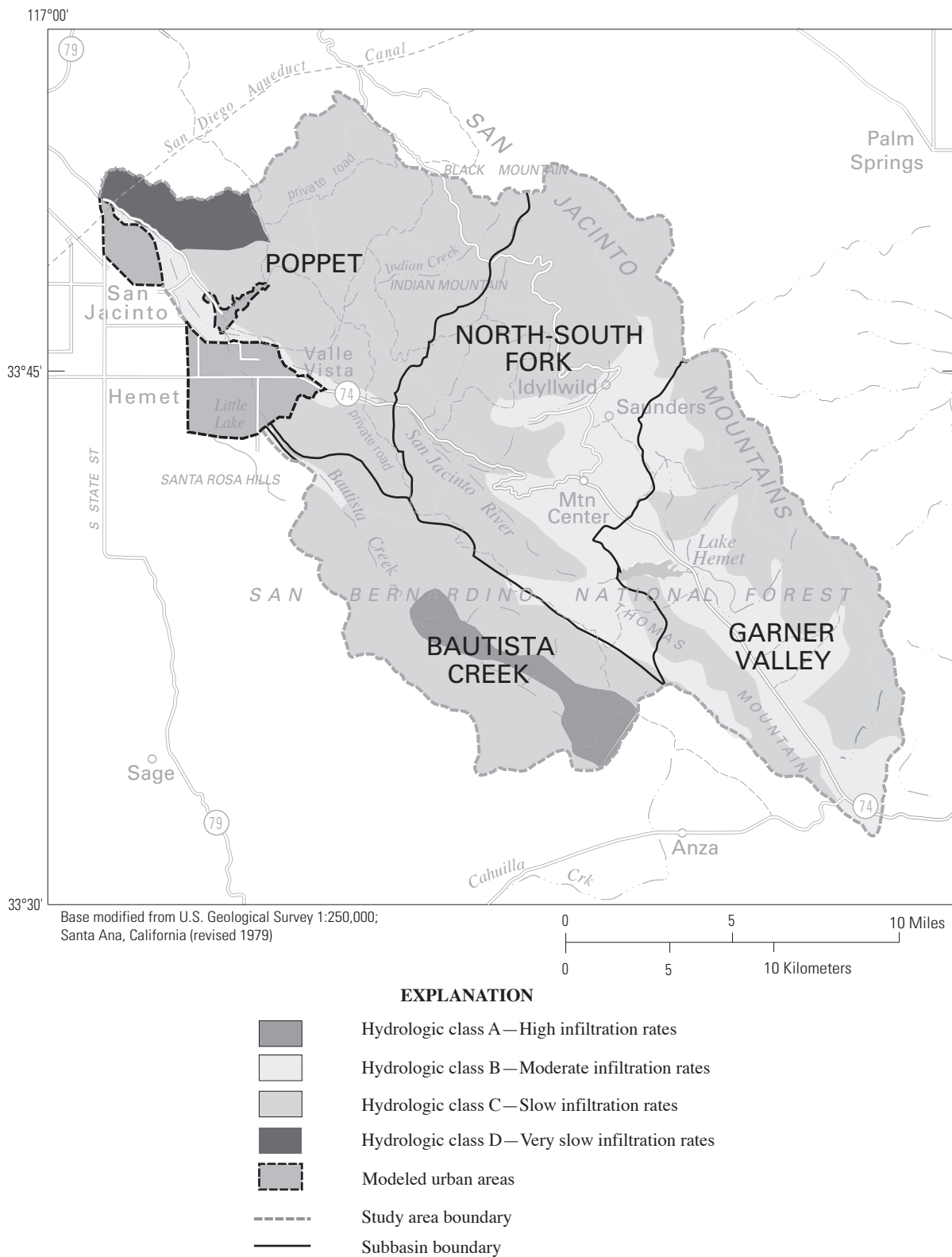
Figure 3. Hydrologic class soils in the eastern part of the San Jacinto River Basin, Riverside County, California. (From U.S. Department of Agriculture, 1994).
