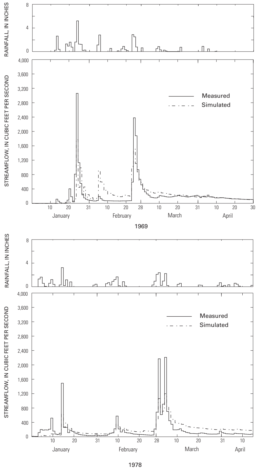
Figure 14. Measured daily rainfall for the Idyllwild precipitation station and measured and simulated daily streamflow for selected storms between 1950 and 1991 at San Jacinto River near San Jacinto (11069500) streamflow-gaging station in the eastern part of the San Jacinto River Basin, Riverside County, California.
