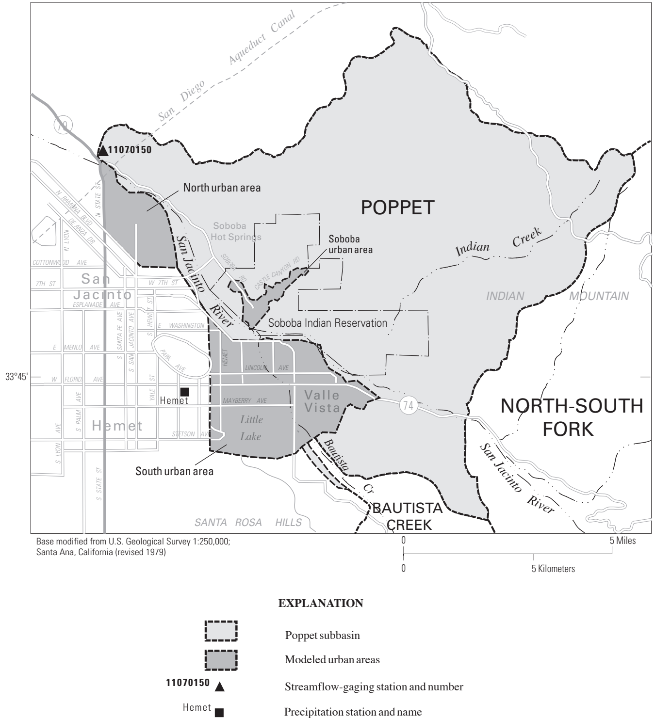
Figure 6. Poppet subbasin in the eastern part of the San Jacinto River Basin, Riverside County, California.
