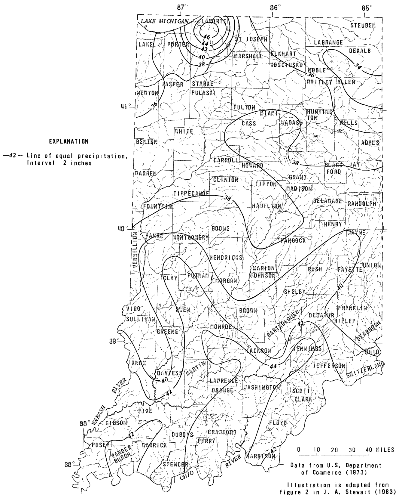
Figure 3.-- Mean annual precipitation, 1941-70.
