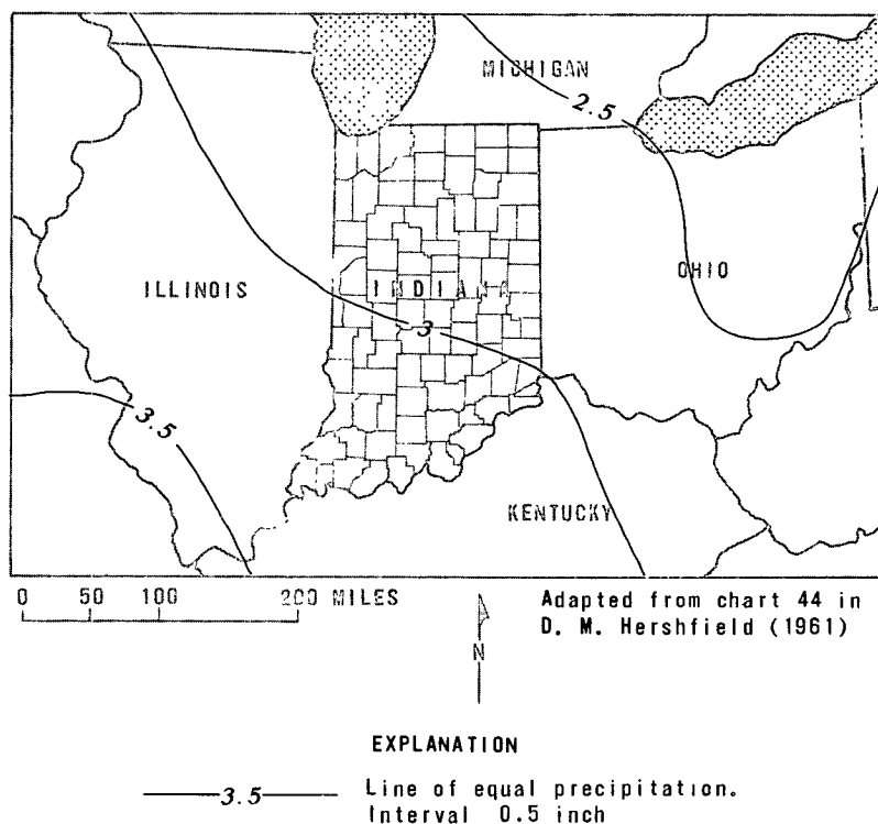
Figure 4.-- Two-year, 24-hour precipitation.
