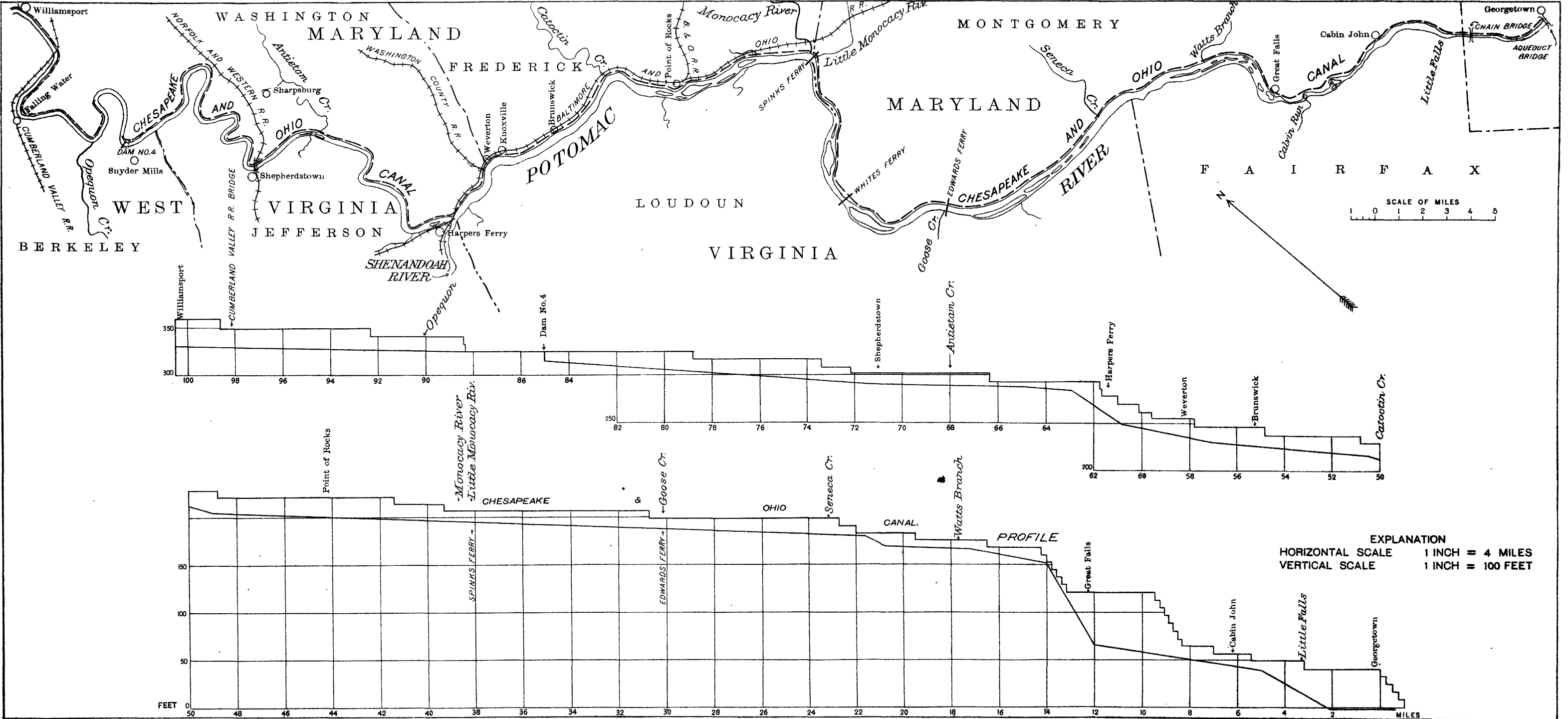
PLAN AND PROFILE OF POTOMAC RIVER FROM GEORGETOWN, D. C., TO WILLIAMSPORT, MD.
