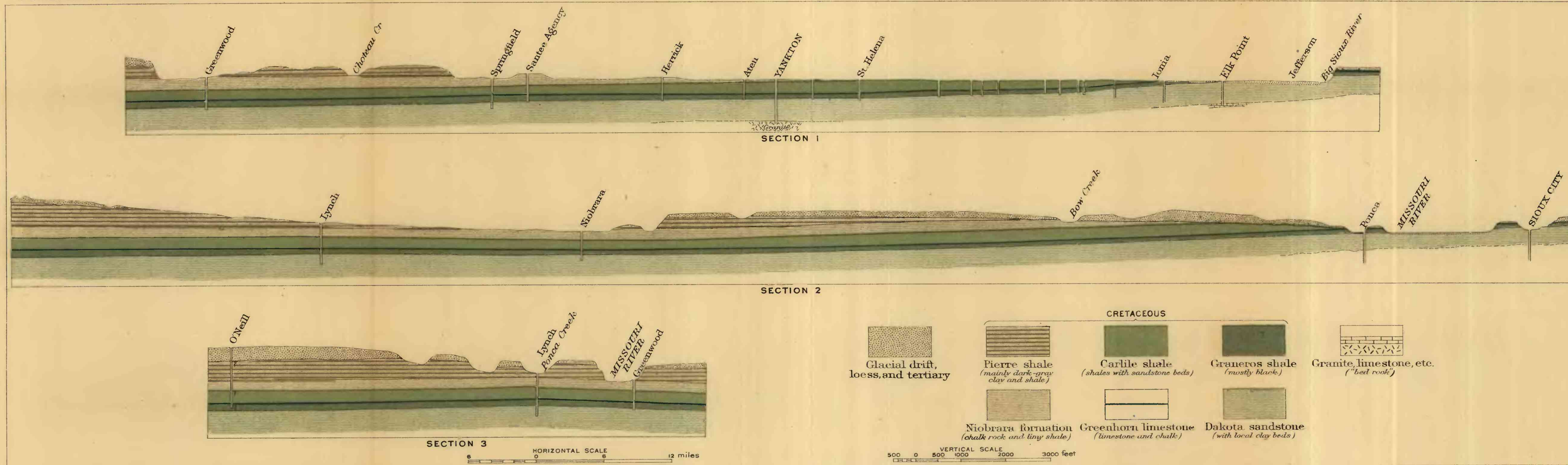
SECTIONS ACROSS NORTHEASTERN NEBRASKA AND ADJACENT PORTIONS OF SOUTH DAKOTA AND IOWA BY N. H. DARTON, G. E. CONDRA, AND J. E. TODD
