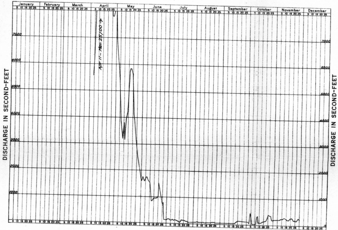
FLUCTUATIONS IN DISCHARGE OF MILK RIVER NEAR VANDALIA, MONT., 1915-1917
