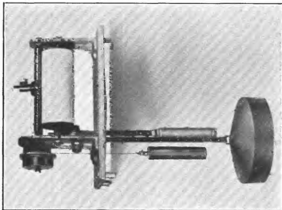
WATER-STAGE RECORDERS
