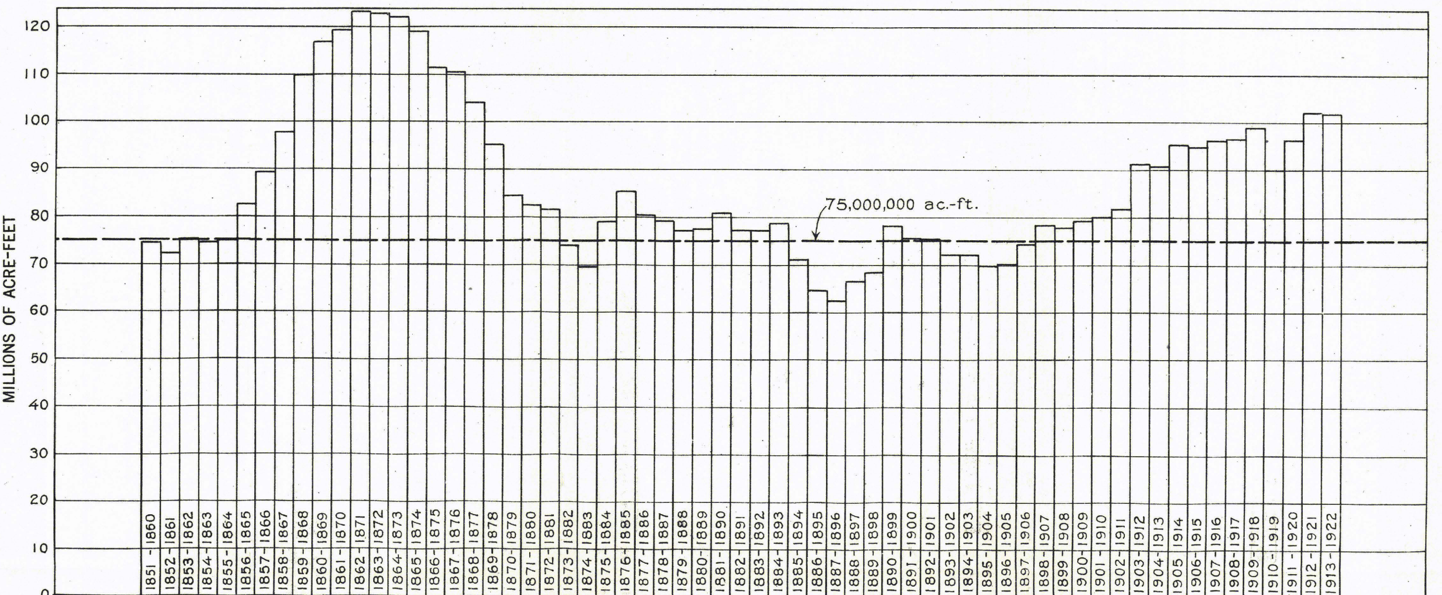
D. COLORADO RIVER AT LEES FERRY WITH COMPLETE IRRIGATION IN THE UPPER BASIN. 10-YEAR PERIODS
