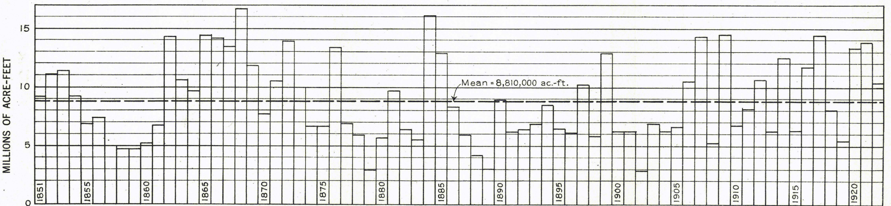
C. COLORADO RIVER AT LEES FERRY WITH COMPLETE IRRIGATION DEVELOPMENT IN THE UPPER BASIN
