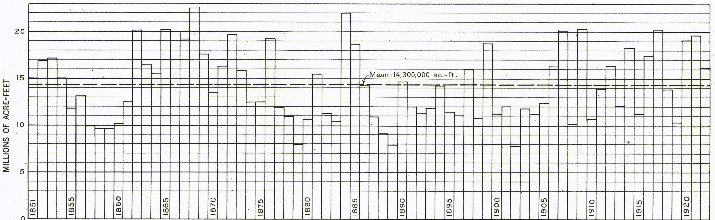
B. COLORADO RIVER AT LEES FERRY CORRECTED FOR PAST IRRIGATION DEPLETION
