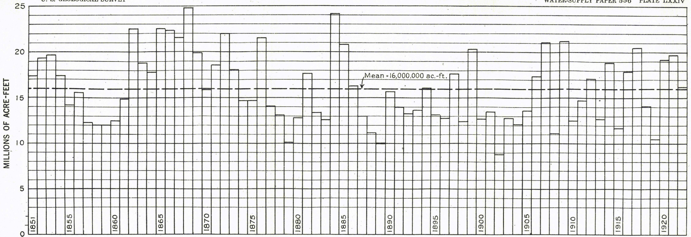
A. COLORADO RIVER AT LEES FERRY WITHOUT CORRECTION FOR DEPLETION
