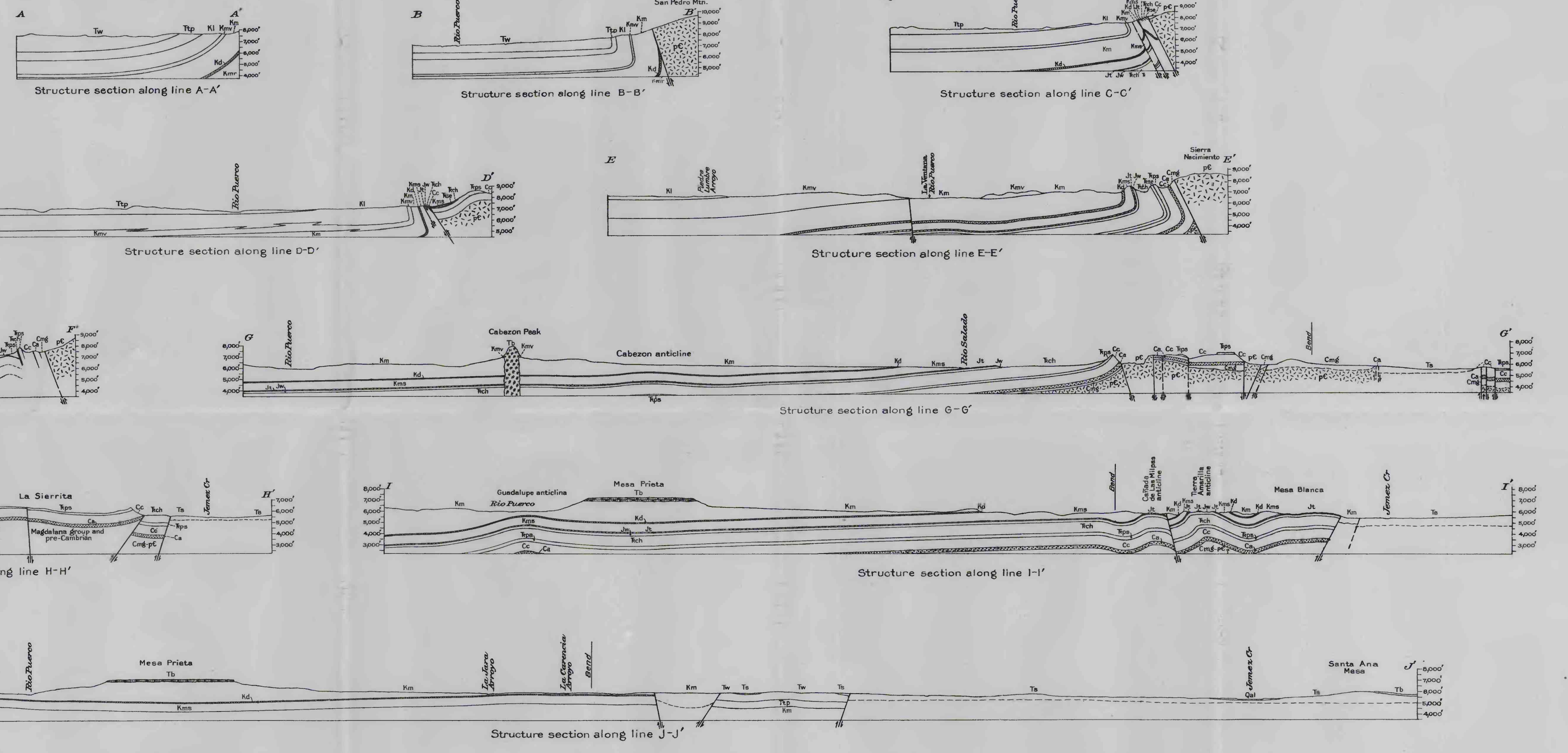
GEOLOGIC MAP AND SECTIONS OF THE WESTERN PART OF SANDOVAL COUNTY, N. MEX.
