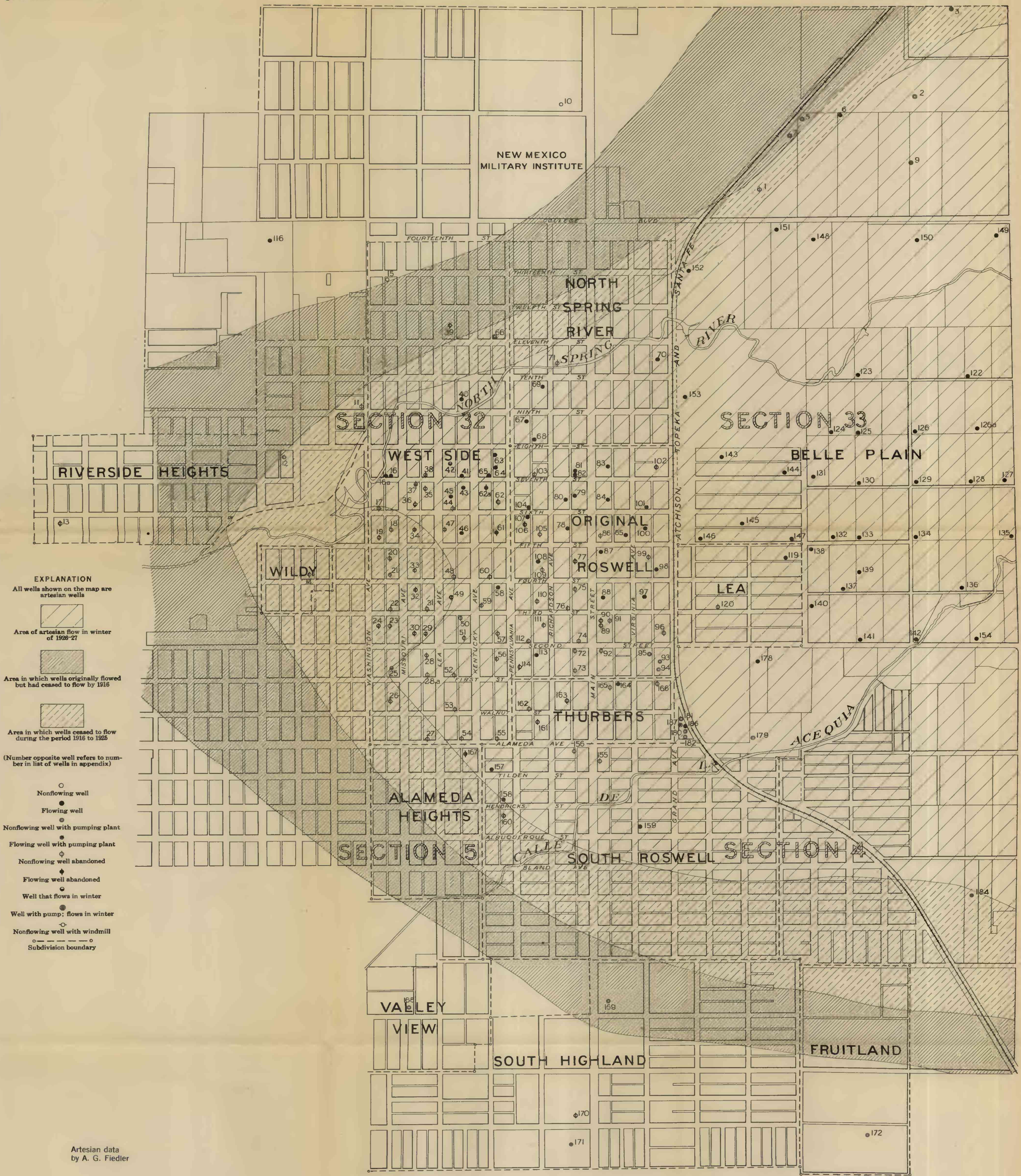
MAP OF CITY OF ROSWELL SHOWING ORIGINAL AREA OF ARTESIAN FLOW, AREAS OF FLOW IN 1916 AND 1926, AND LOCATION OF ARTESIAN WELLS
