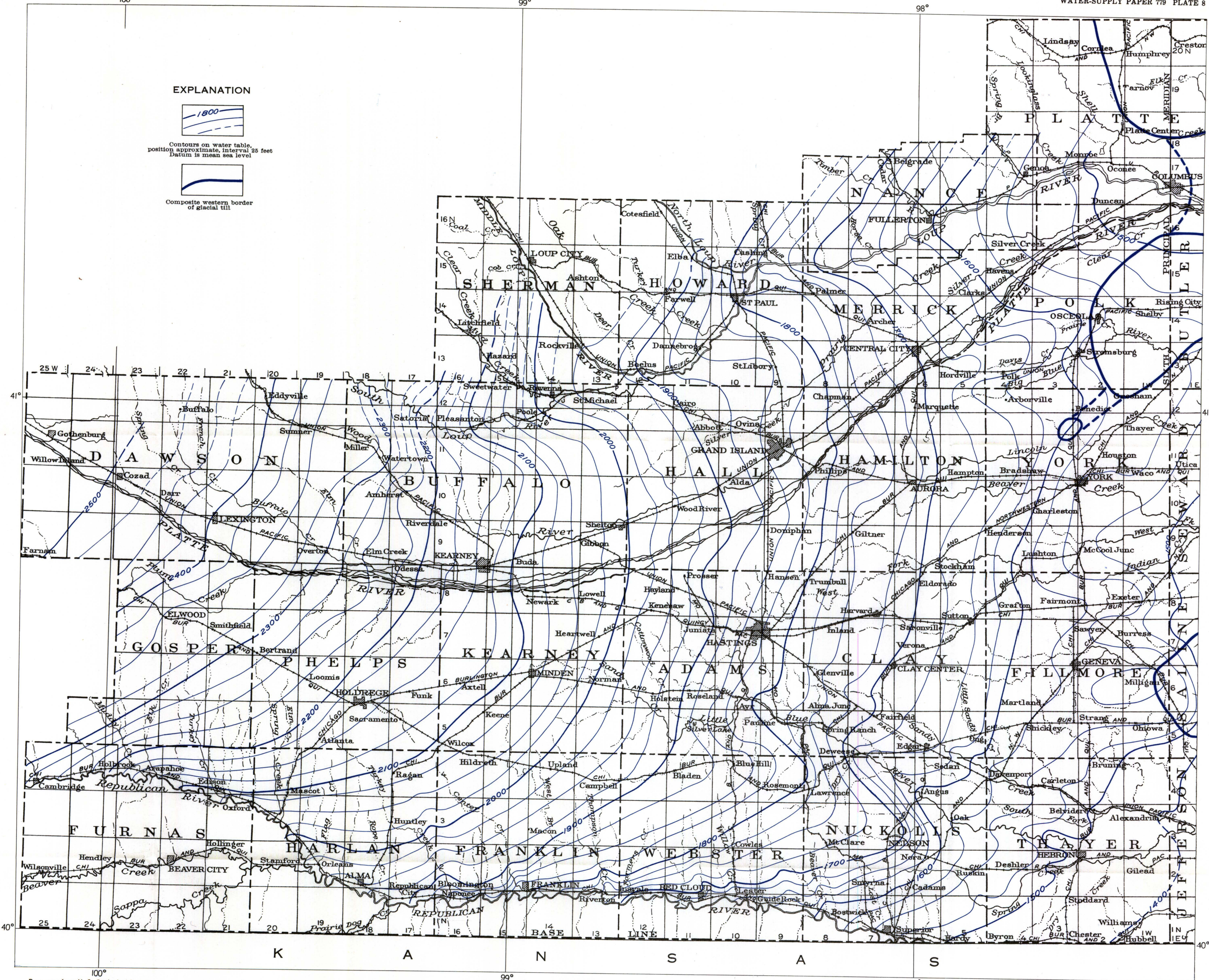
MAP SHOWING CONTOURS ON THE WATER TABLE FOR SOUTH-CENTRAL NEBRASKA
