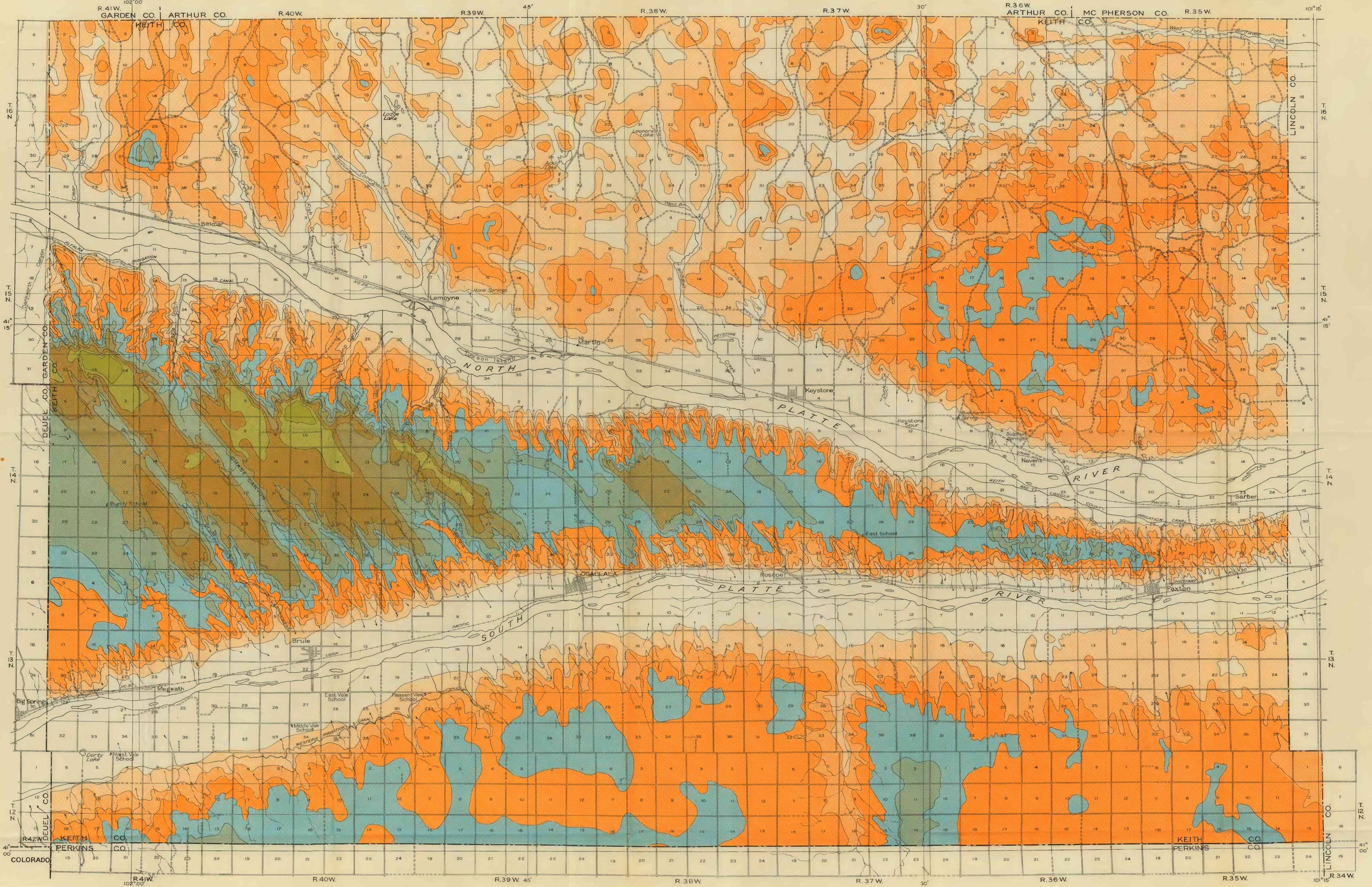
MAP SHOWING DEPTH OF THE WATER TABLE BELOW THE LAND SURFACE, KEITH COUNTY, NEBRASKA
