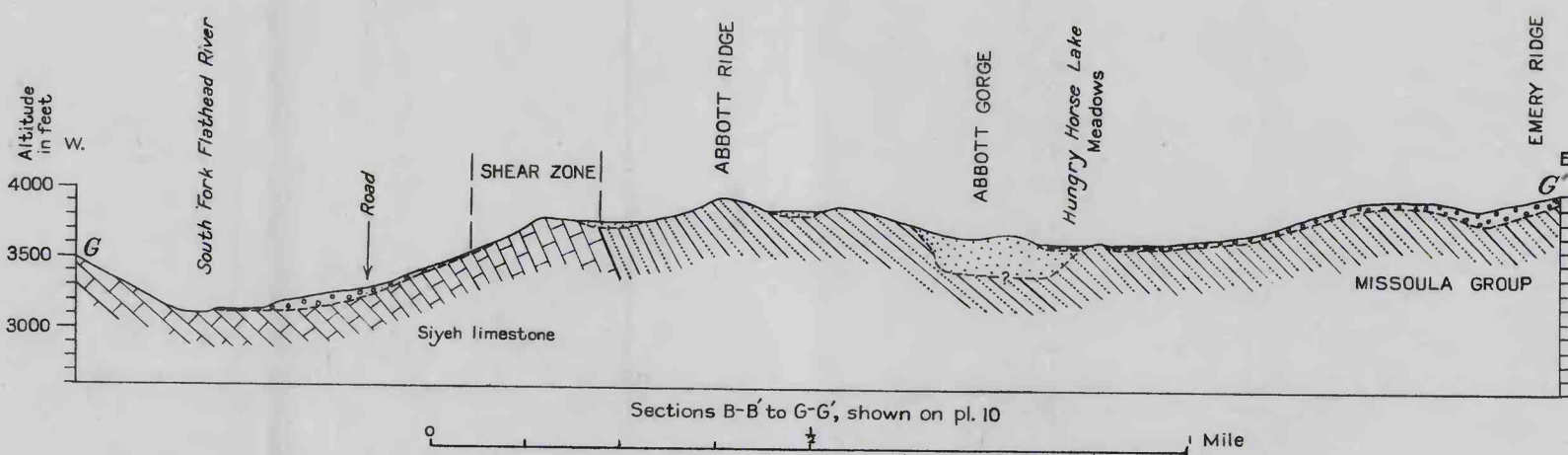
CROSS SECTIONS OF ABBOTT GORGE AND LION HILL GORGE, HUNGRY HORSE PROJECT
