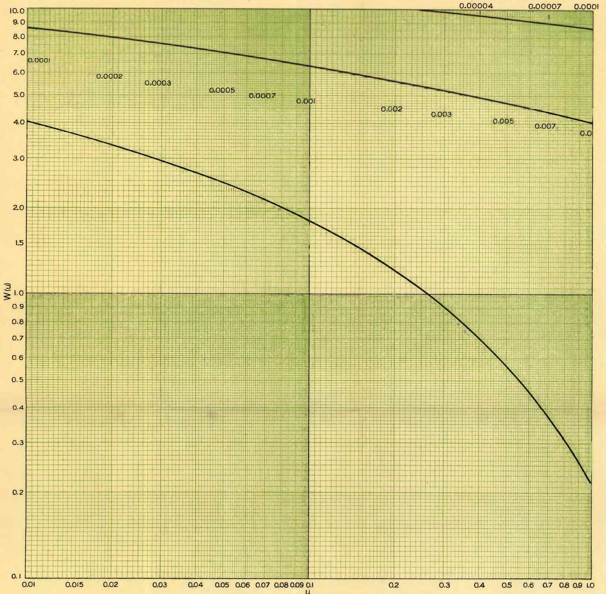
TYPE CURVE FOR NON-EQUILIBRIUM FORMULA.
