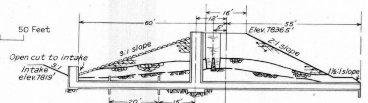
SECTION ON OUTLET CENTER LINE
