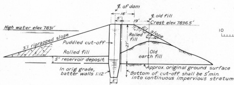
SECTION OF DAM
