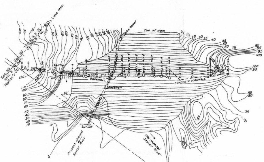
PLAN AND PRESENT TOPOGRAPHY OF ENLARGED SEVIER BRIDGE DAM Contour interval 5 feet Datum assumed
