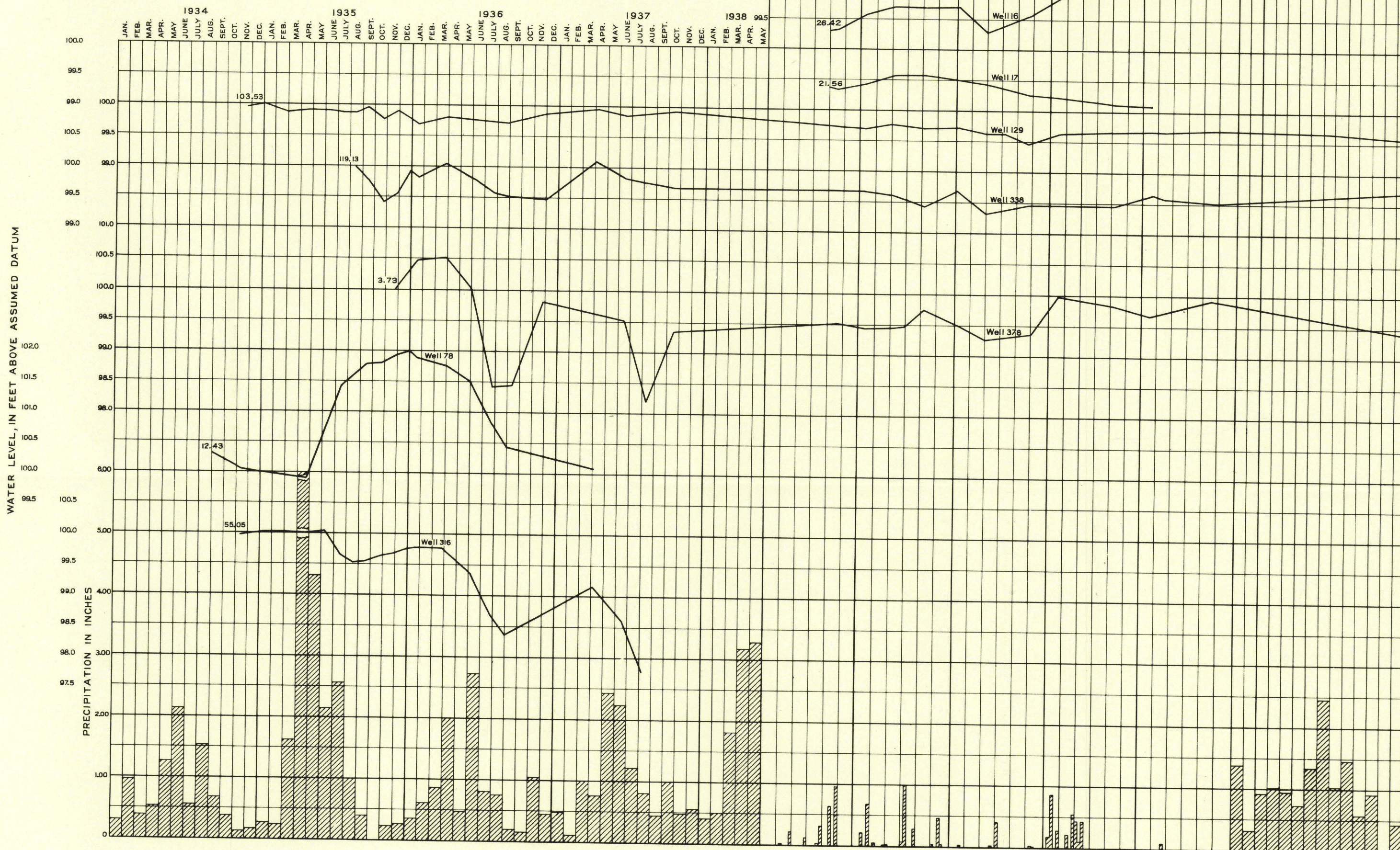
HYDROGRAPHS OF OBSERVATION WELLS IN BOX BUTTE COUNTY, NEBRASKA, FOR THE YEARS 1934-39
