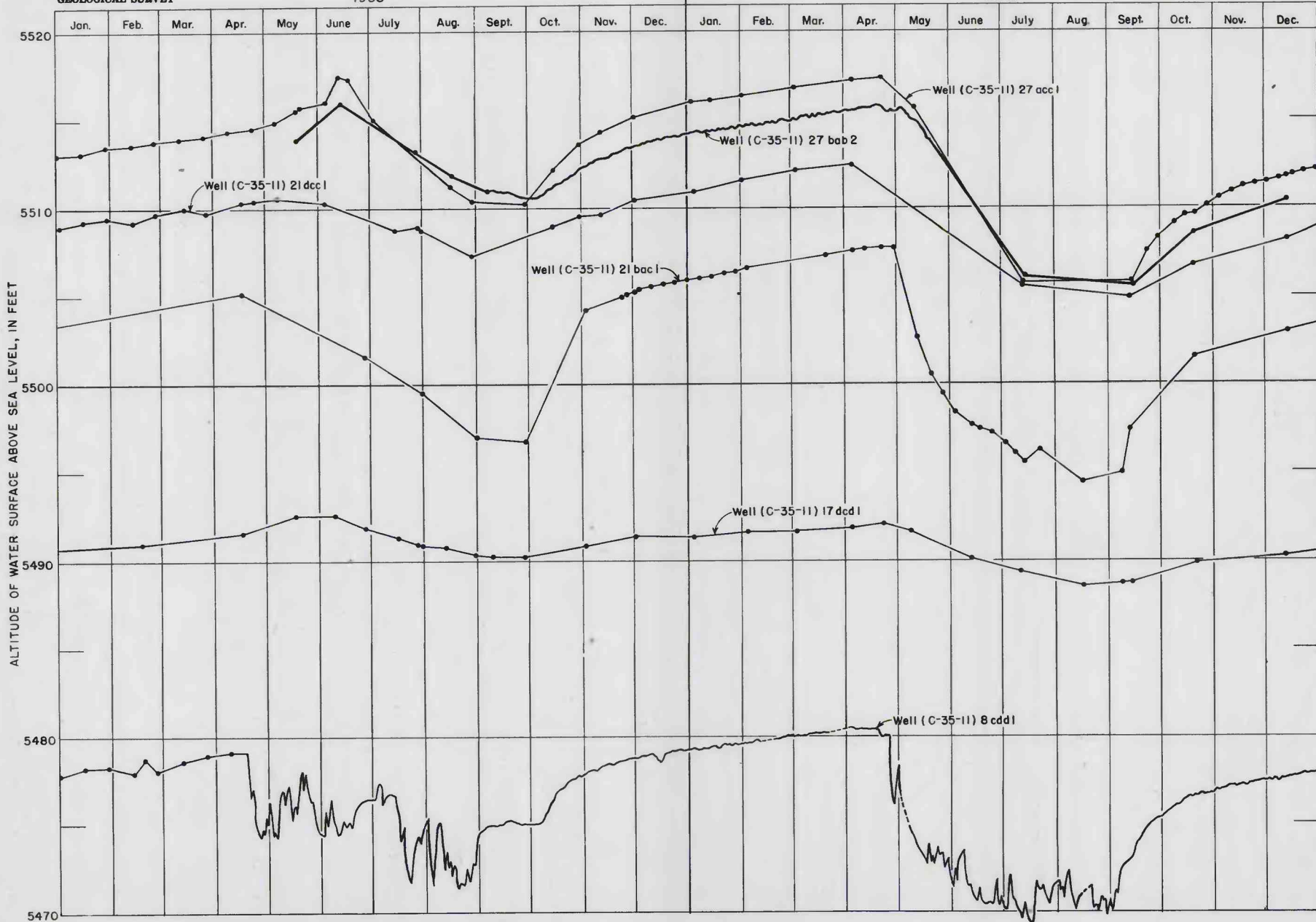
HYDROGRAPHS OF SIX WELLS THAT ARE LOCATED ALONG A LINE EXTENDING NORTHWESTERLY ACROSS SECS. 27, 21, 17, AND 8, T. 35 S., R. 11 W
