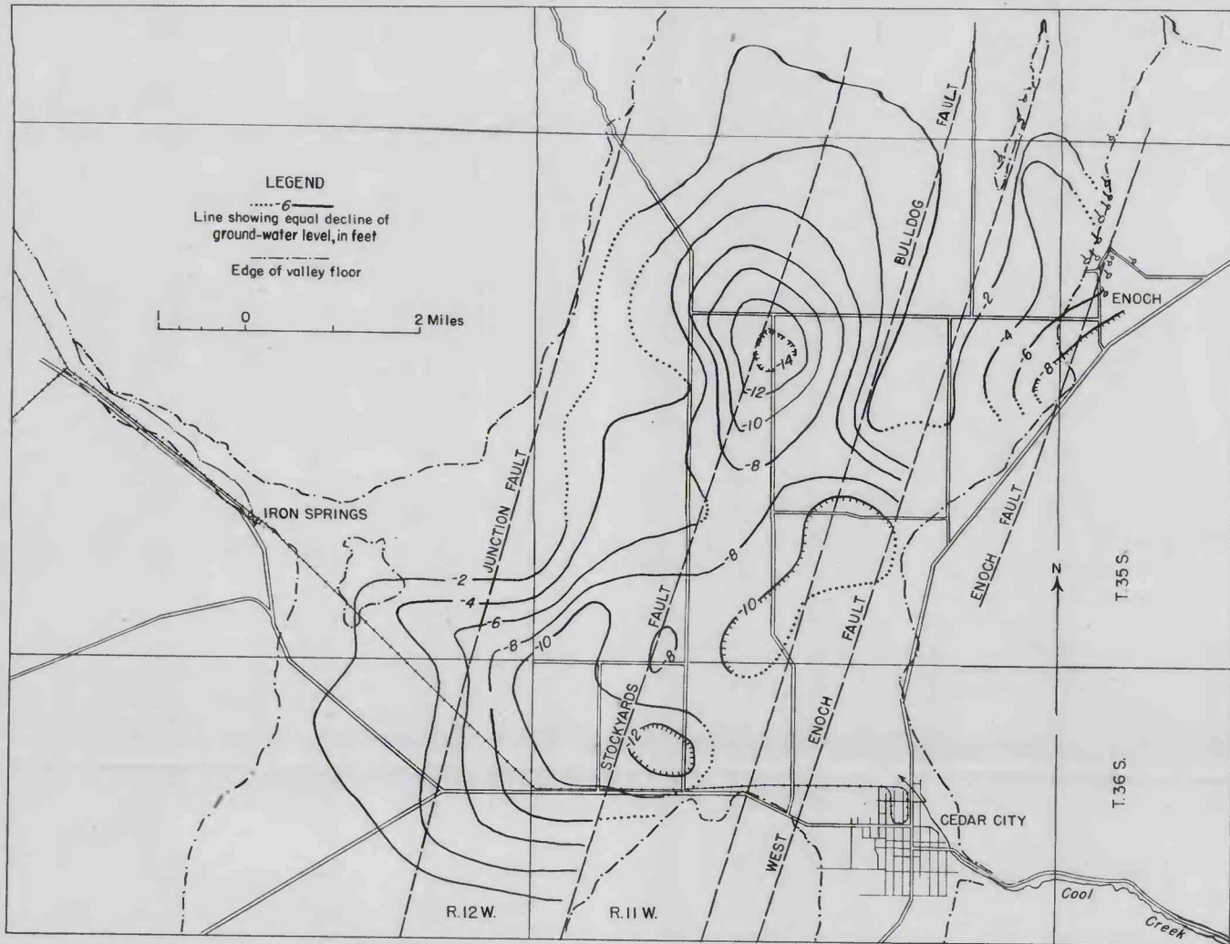
MAP OF PART OF CEDAR CITY VALLEY SHOWING DECLINE OF GROUND-WATER LEVELS BETWEEN APRIL 1 AND SEPTEMBER 15, 1939
